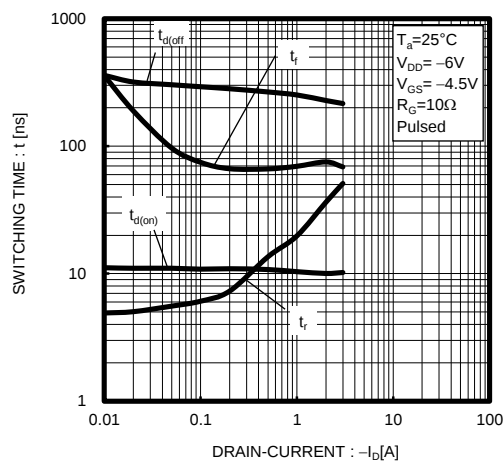
Fig.12 Switching Characteristics
