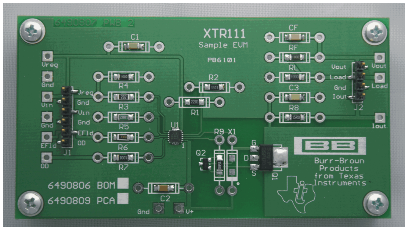
Figure 1. XTR111EVM
