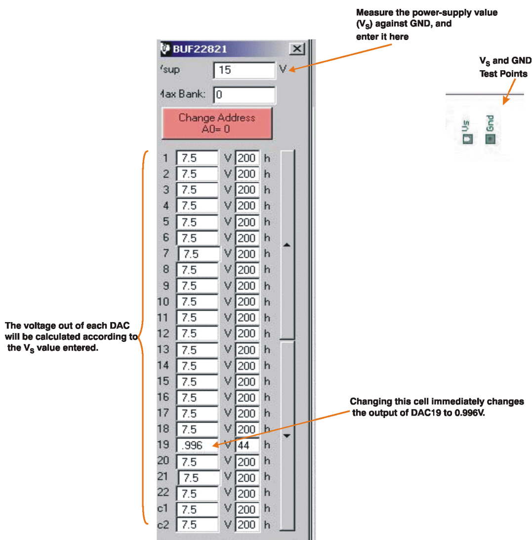
Figure 12. Power Supply Measurement and Recording
