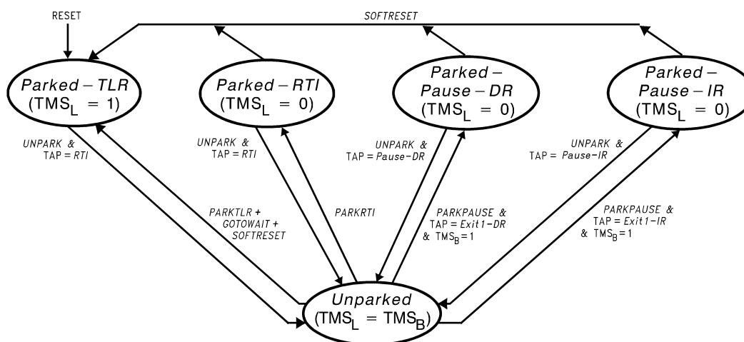
Figure 3-4. Local SCANPSC110F Bridge Port Configuration State Machine
