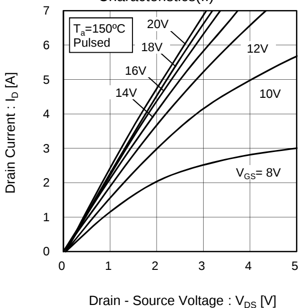
Fig.7 T j = 150°C Typical Output Characteristics(II)
