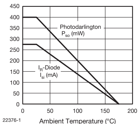
Fig. 2 - Derating Diagram
