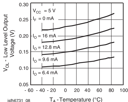
Fig. 8 - Typical Low Level Output Voltage vs. Temperature
