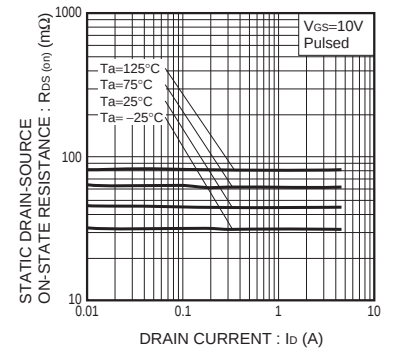
Fig.3 Static Drain-Source On-State Resistance vs. Drain Current(II)
