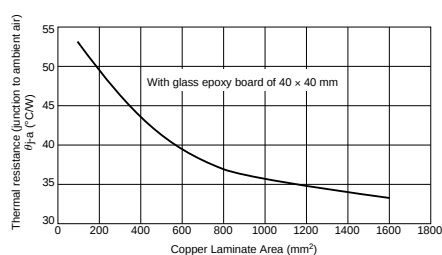
Copper Lamine Area on Glass Epoxy Board vs. thermal resistance (junction to ambient air) (Typical Value)
