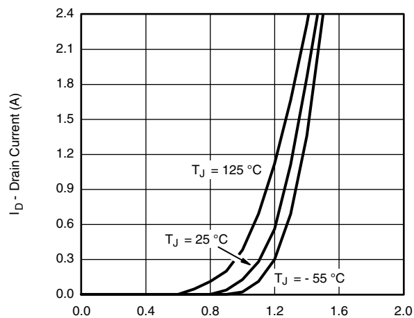
V_{GS} - Gate-to-Source Voltage (V) Transfer Characteristics Curves vs. Temperature
