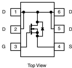
SOT-363 SC-70 (6-LEADS)
