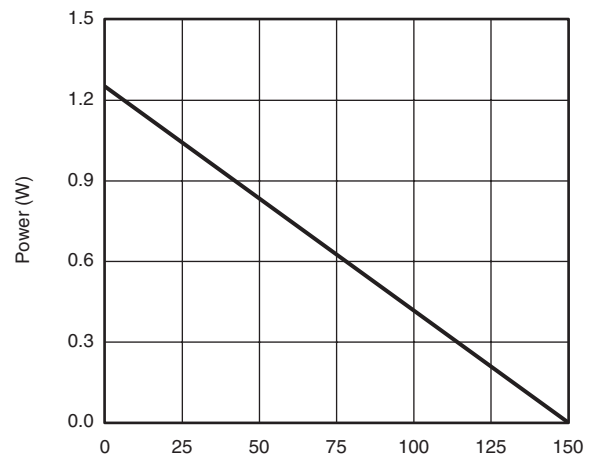
Power Derating ( T_A )
