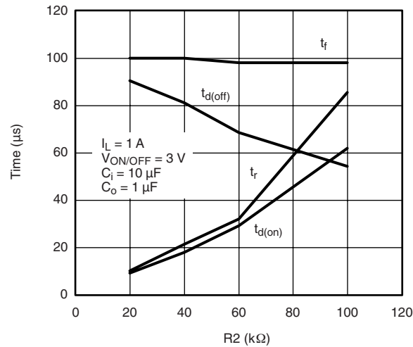
Switching Variation R2 at V_{\text{IN}} = 4.5 \text{ V} , R1 = 300 \text{ kΩ}
