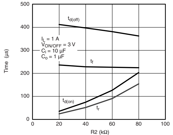
Switching Variation R2 at V_{IN} = 1.8 V, R1 = 300 kΩ
