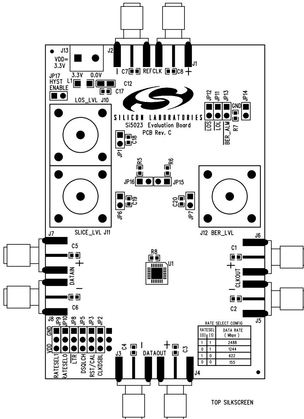
Figure 5. Si5023 Silkscreen
