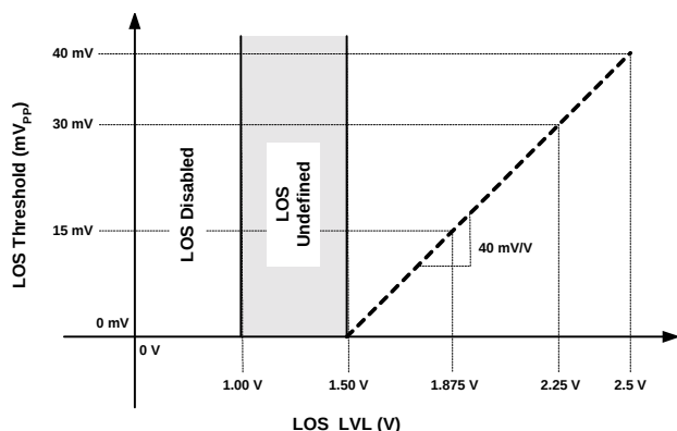
Figure 2. LOS_LVL Mapping
