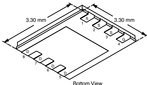
PowerPAK® 1212-8
