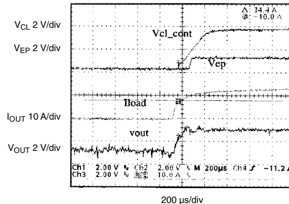
Figure 10. Overload Recovery
