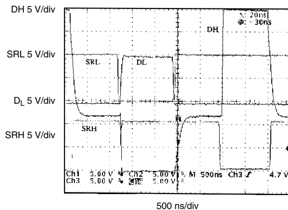
Figure 12. Drive Waveforms
