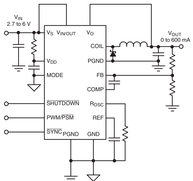
Buck Configuration
