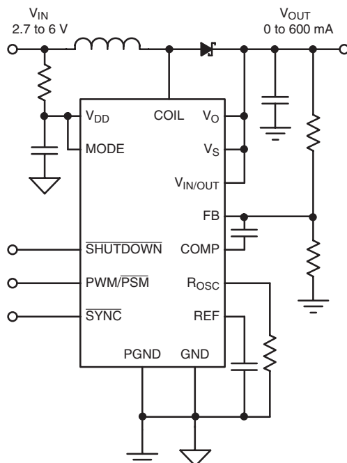
Boost Configuration
