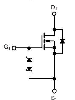
N-Channel MOSFET
