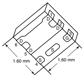
PowerPAK SC-75-6L-Single
