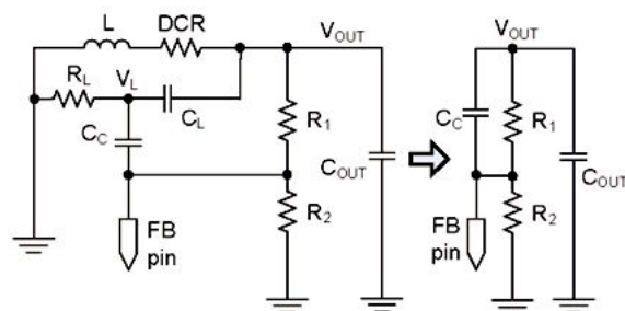
Figure 16 - FB Voltage by Output Voltage
