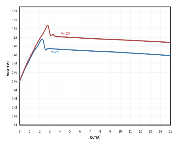
Load Regulation - P-Save (V_{DD} = 3.3\text{ V}, V_{OUT} = 1.5\text{ V}, \text{SiC401B})
