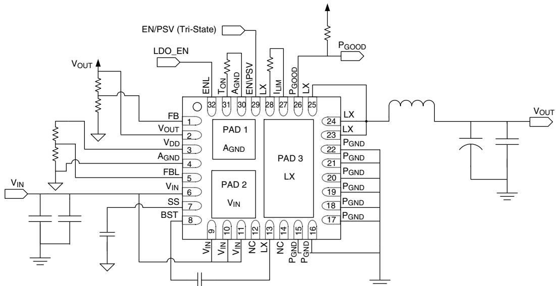
Typical Application Circuit for SiC401A/B (PowerPAK MLP5x5-32L)
