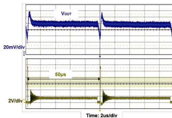
Figure 17 - Ultra-sonic PSM - SiC402ACD ( V_{DD} = 5\text{ V} , V_{IN} = 12\text{ V} , V_{OUT} = 1.5\text{ V} , I_{OUT} = 0\text{ A} )
