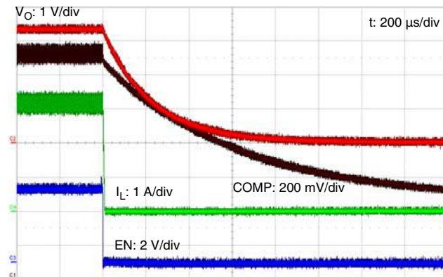
System shuts down with EN pin becoming LOW. V_{IN} = 12\text{ V} , V_O = 3.3\text{ V} and I_O comes down from about 3 A.
