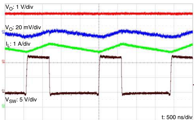
V_O ripple and V_{SW} switching waveform. V_{IN} = 12\text{ V} , V_O = 3.3\text{ V} and L = 10\text{ μH} (IHL2525EZ type). C_O consists of MLCC of 4.7 \mu\text{F} and tantalum of 100 \mu\text{F}/20\text{ V} \times 2
