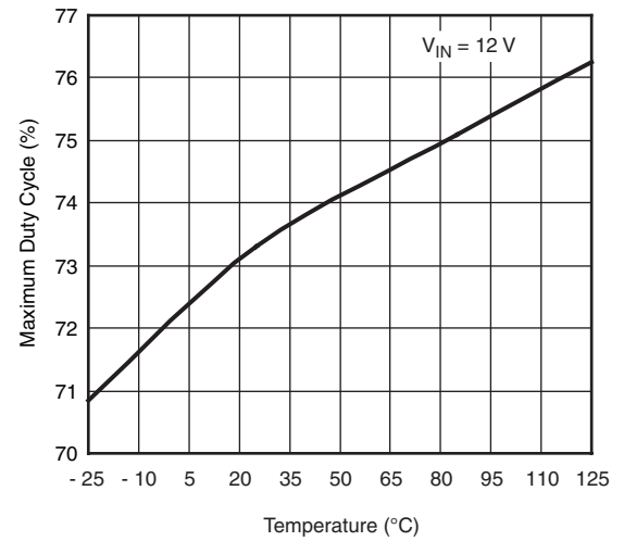
Maximum Duty Cycle vs. Temperature
