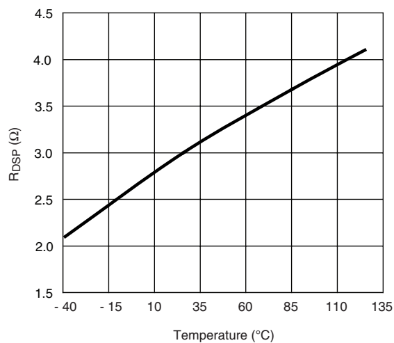
DL R_{DSP} vs. Temperature
