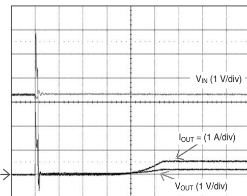
Short Circuit through 0.3 \Omega , V_{in} = 3.3 \text{ V}
