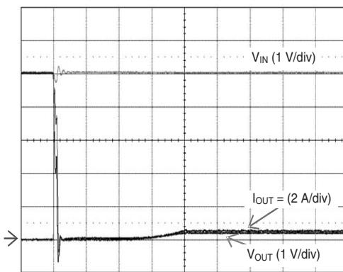
Short Circuit through 0.3 \Omega , V_{in} = 5 \text{ V}
