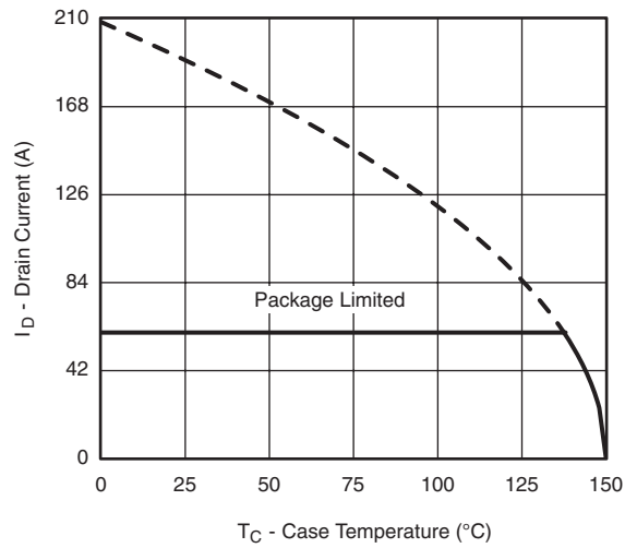
Current Derating*
