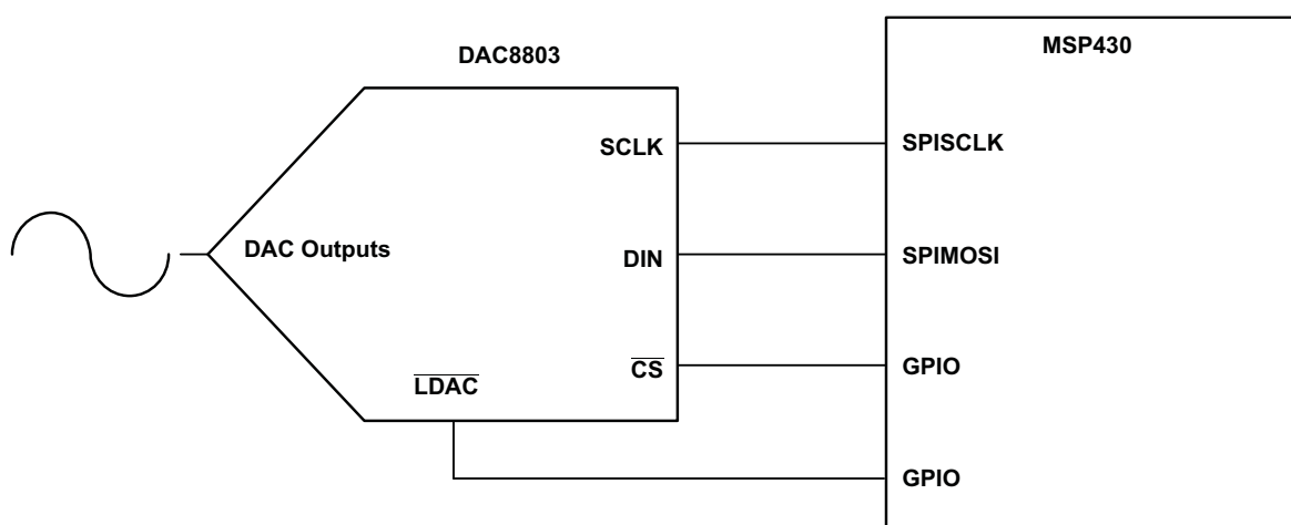
Figure 1. Basic Hardware Interface
