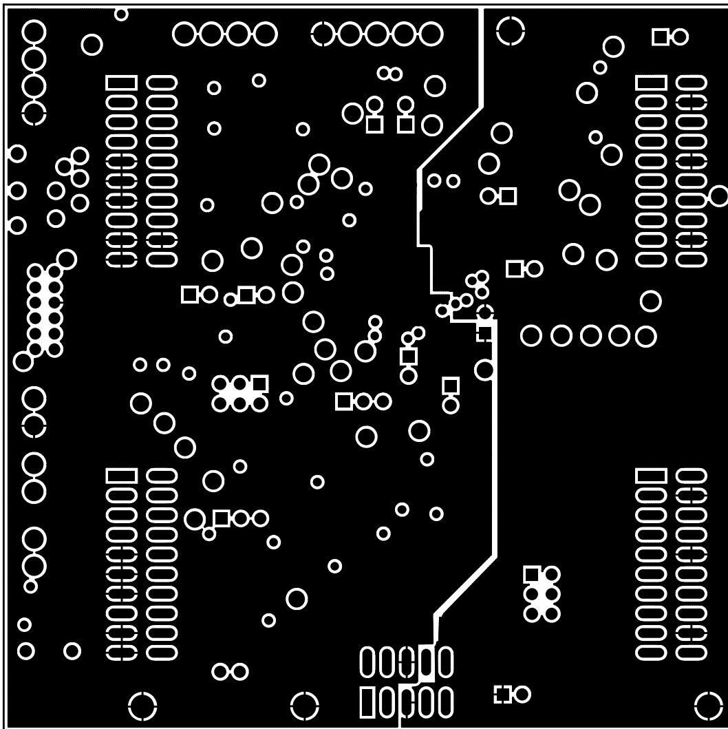
Figure 12. Power/Ground Plane 1
