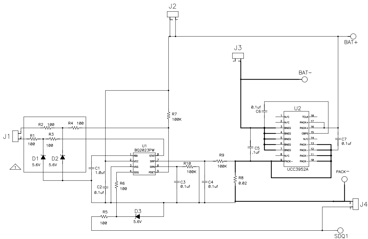
Figure 2–1. Schematic
