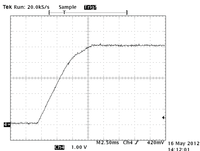
Figure 6. 5-Ω Load
