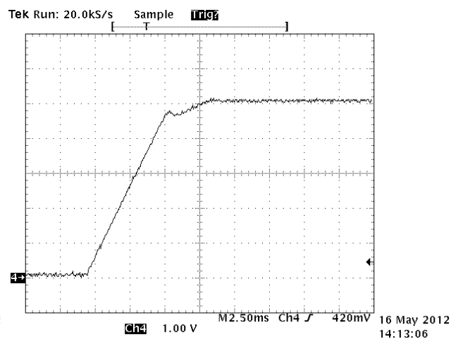
Figure 8. 5-Ω Load
