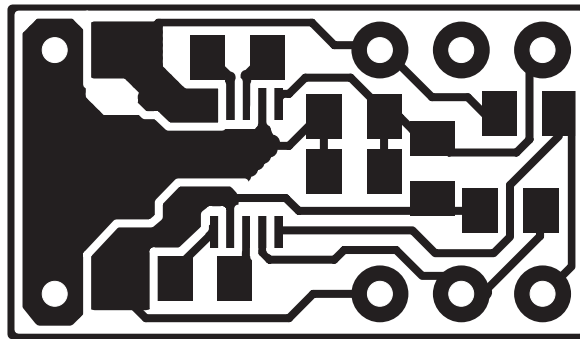
Figure 2–4. Actual Size of the EVM, 17,9 mm × 10,2 mm
