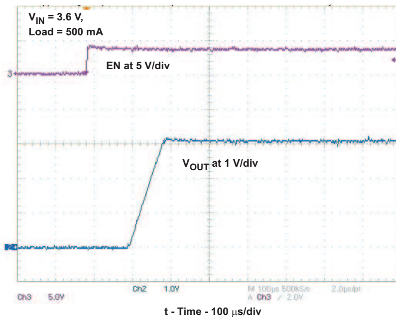
Figure 1. Vout Start-up From Enable
