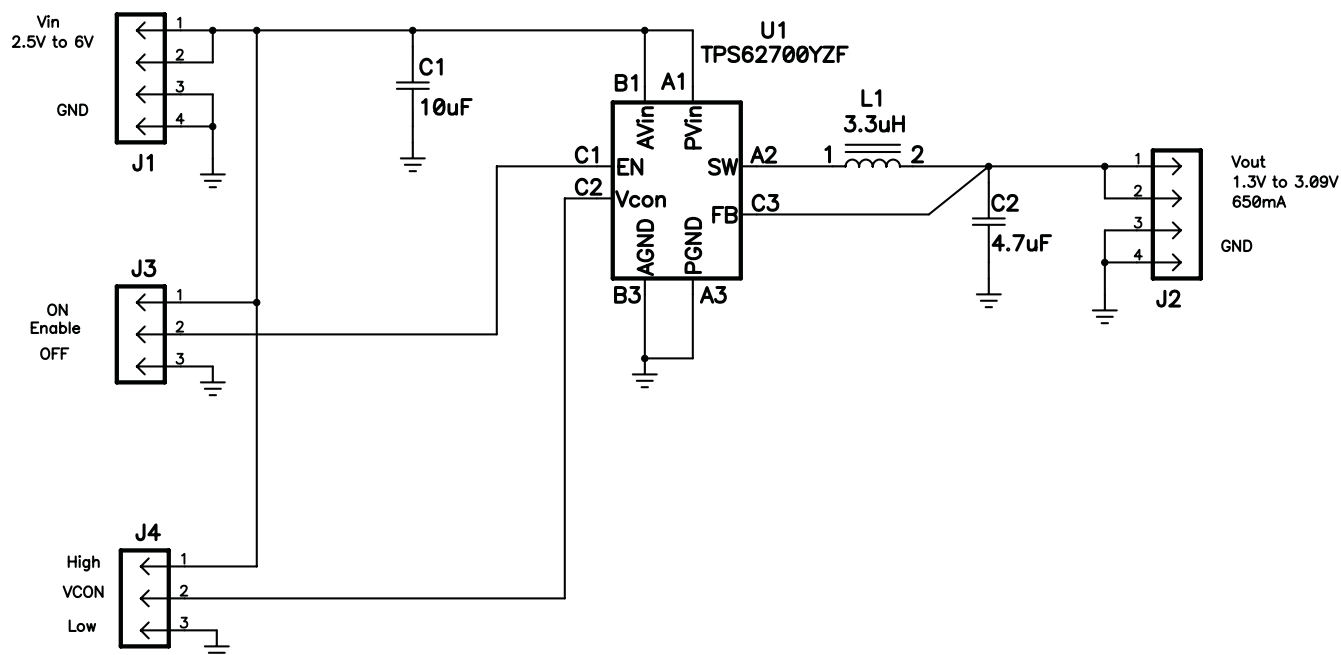
Figure 10. TPS62700EVM-264 Schematic
