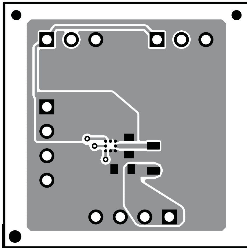
Figure 8. Top Layer
