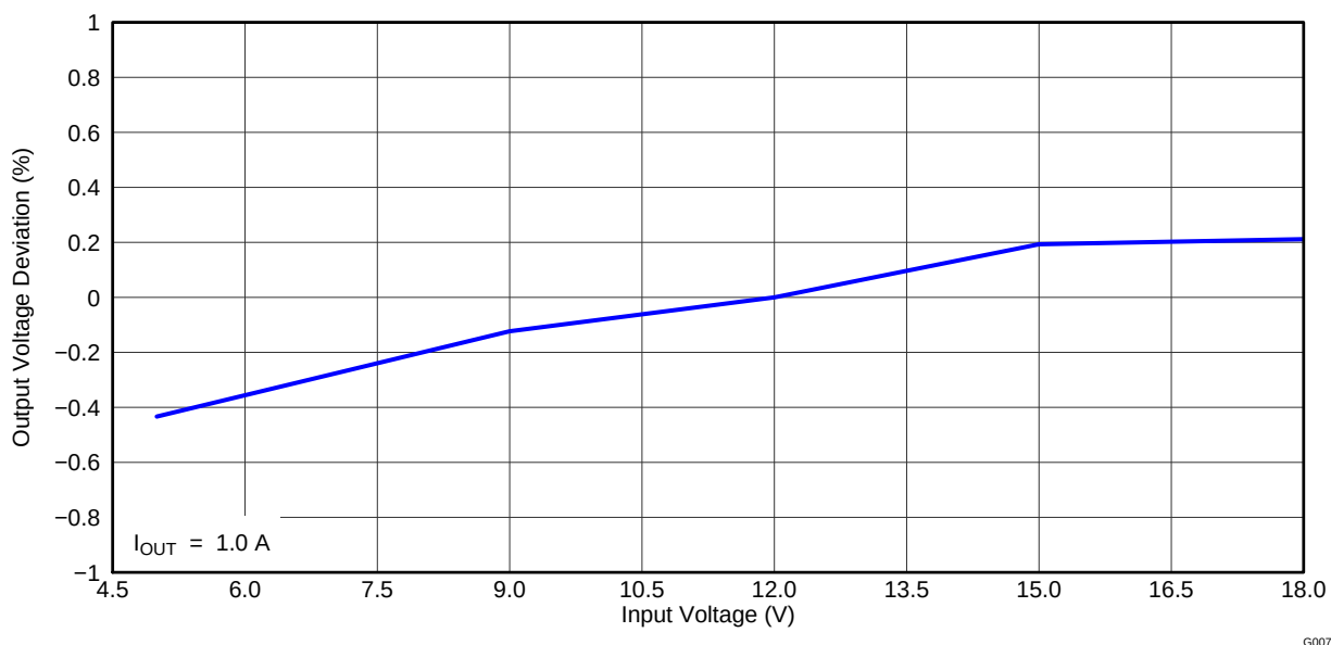
Figure 8. TPS54495EVM Converter 2 Line Regulation
