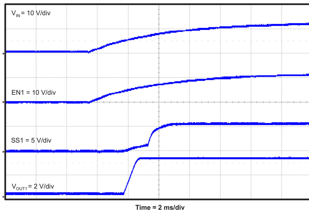
Figure 16. TPS54495EVM Converter 1 Start-Up Relative to V_{IN}
