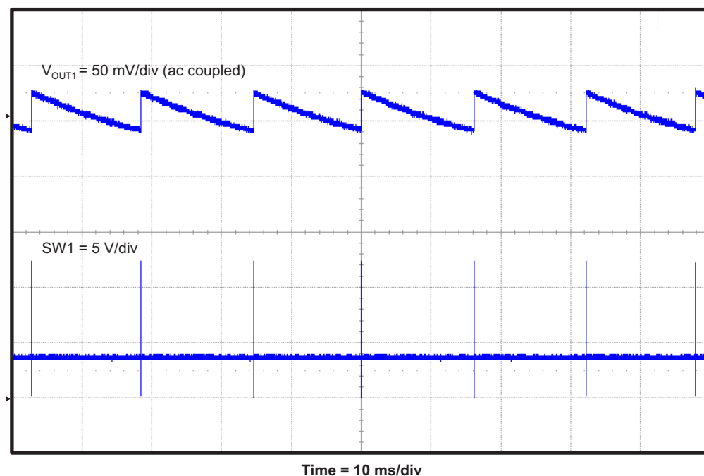
Figure 12. TPS54495EVM Converter 1 Eco-mode™ Output Voltage Ripple at No Load
