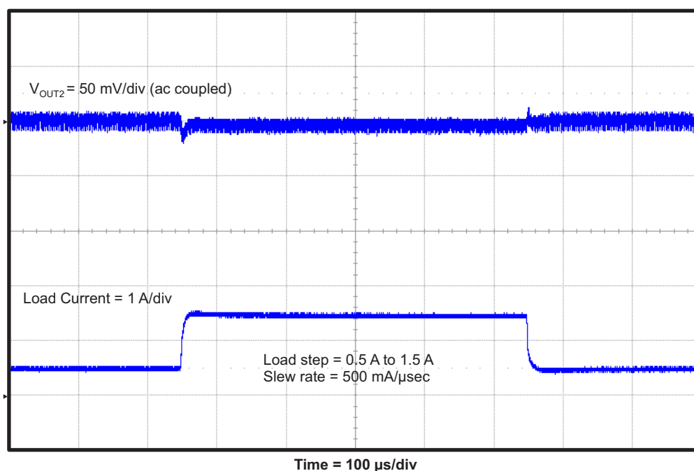
Figure 10. TPS54495EVM Converter 2 Load Transient Response
