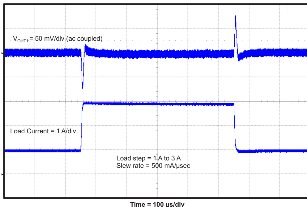
Figure 9. TPS54495EVM Converter 1 Load Transient Response
