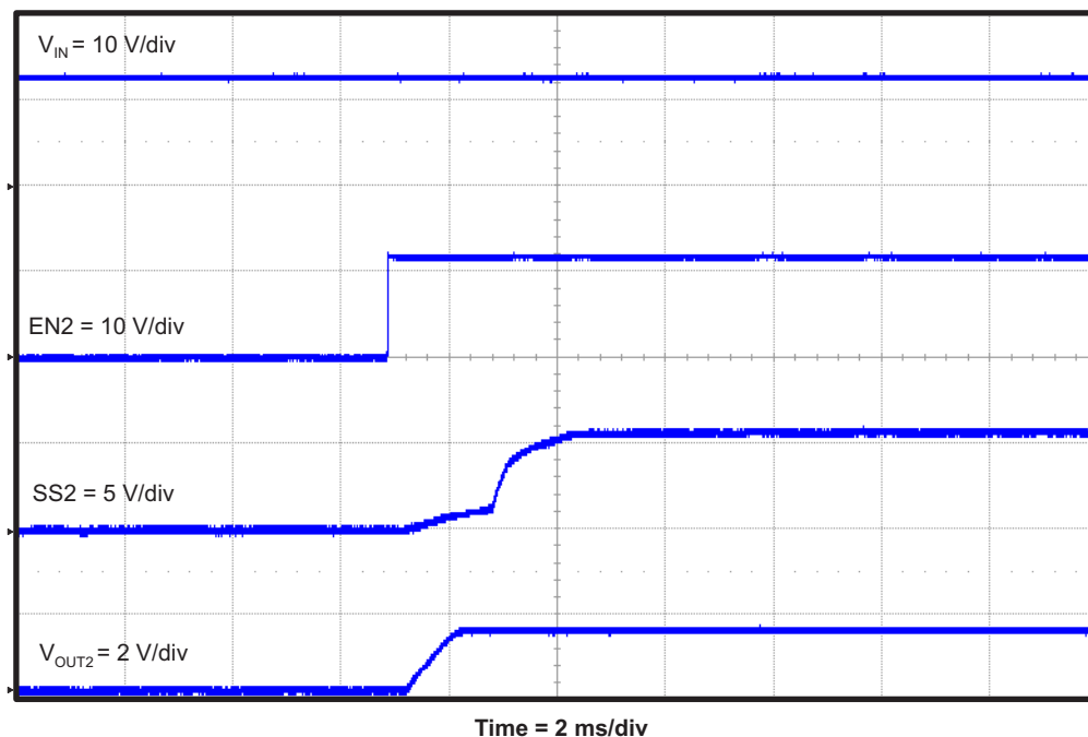
Figure 19. TPS54495EVM Start-Up Relative to EN2
