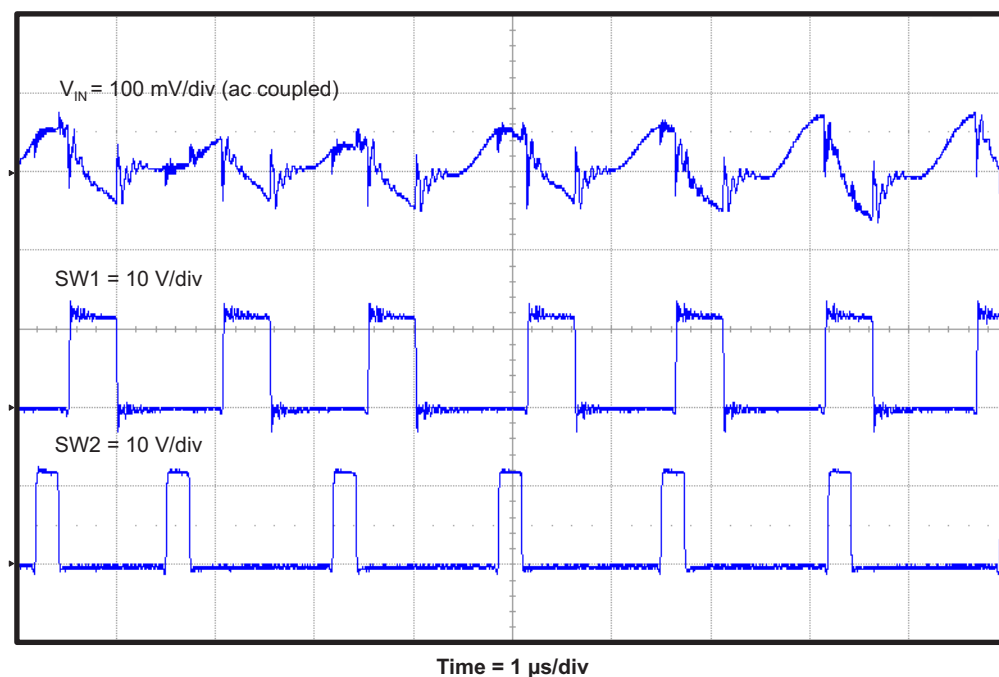
Figure 15. TPS54495EVM Input Voltage Ripple
