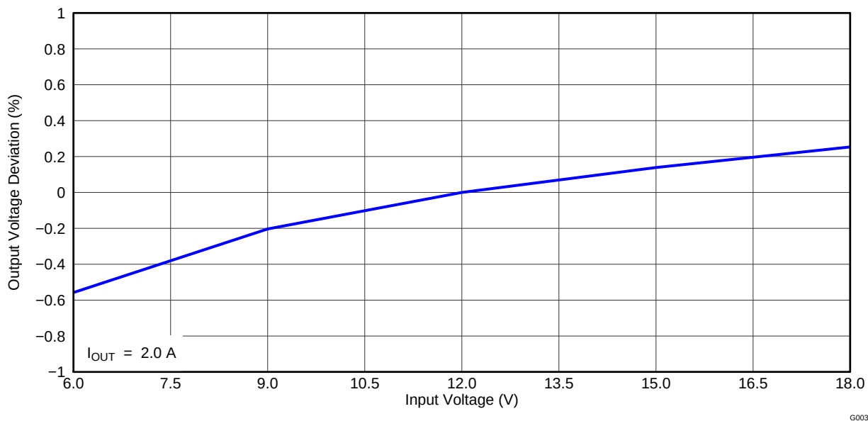
Figure 7. TPS54495EVM Converter 1 Line Regulation
