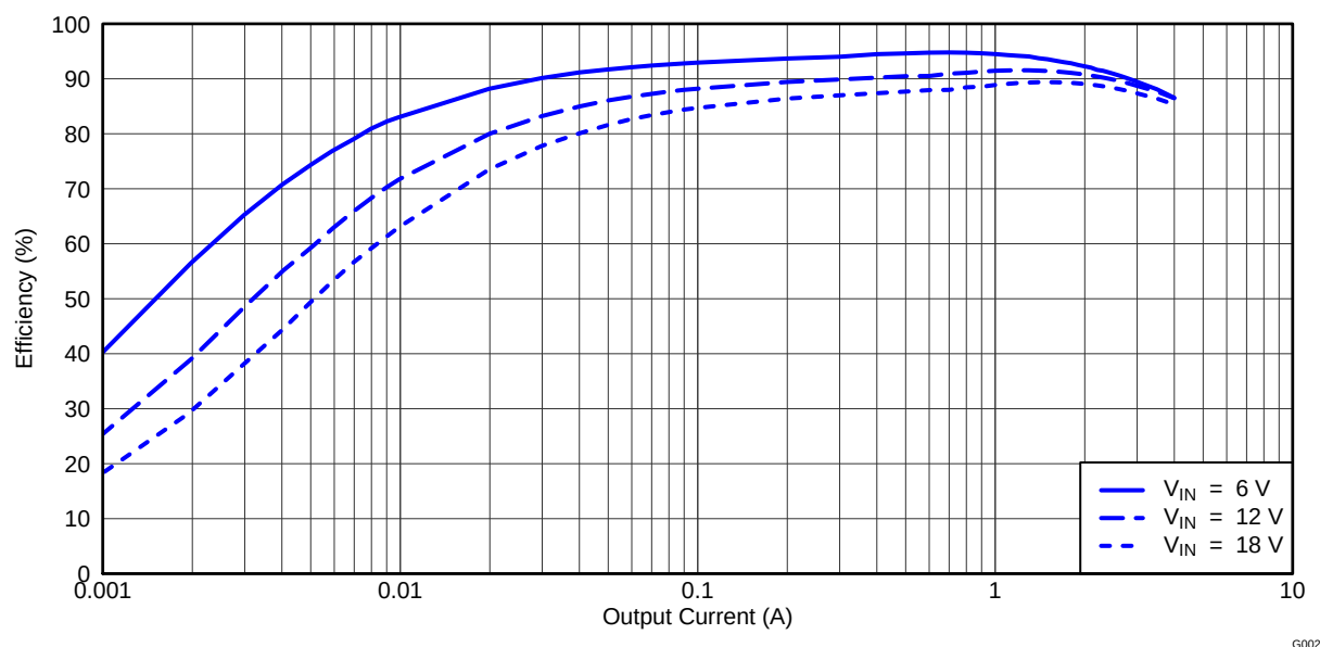
Figure 2. TPS54495EVM Converter 1 Light Load Efficiency
