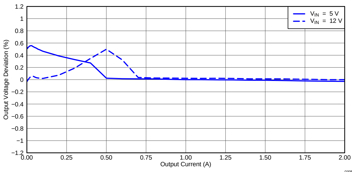
Figure 6. TPS54495EVM Converter 2 Load Regulation
