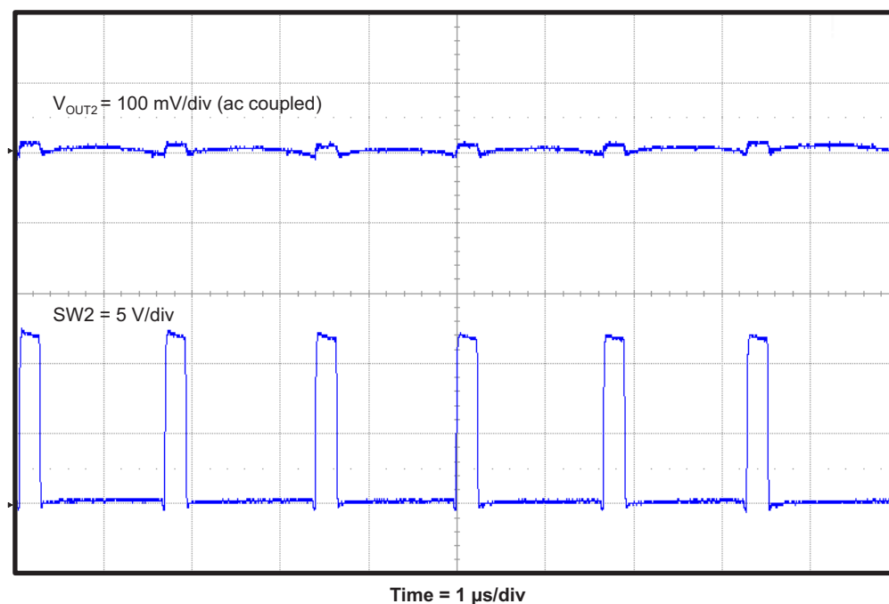
Figure 13. TPS54495EVM Converter 2 Output Voltage Ripple
