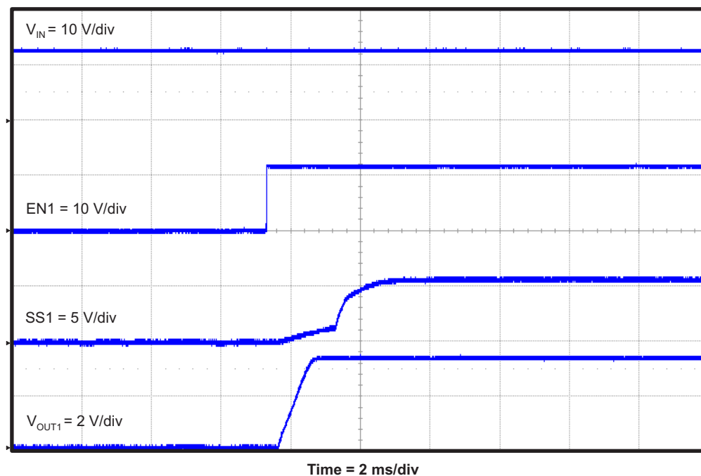
Figure 17. TPS54495EVM Start-Up Relative to EN1
