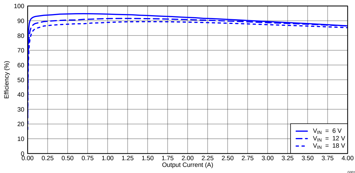
Figure 1. TPS54495EVM Converter 1 Efficiency
