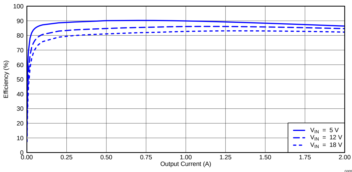
Figure 3. TPS54495EVM Converter 2 Efficiency
