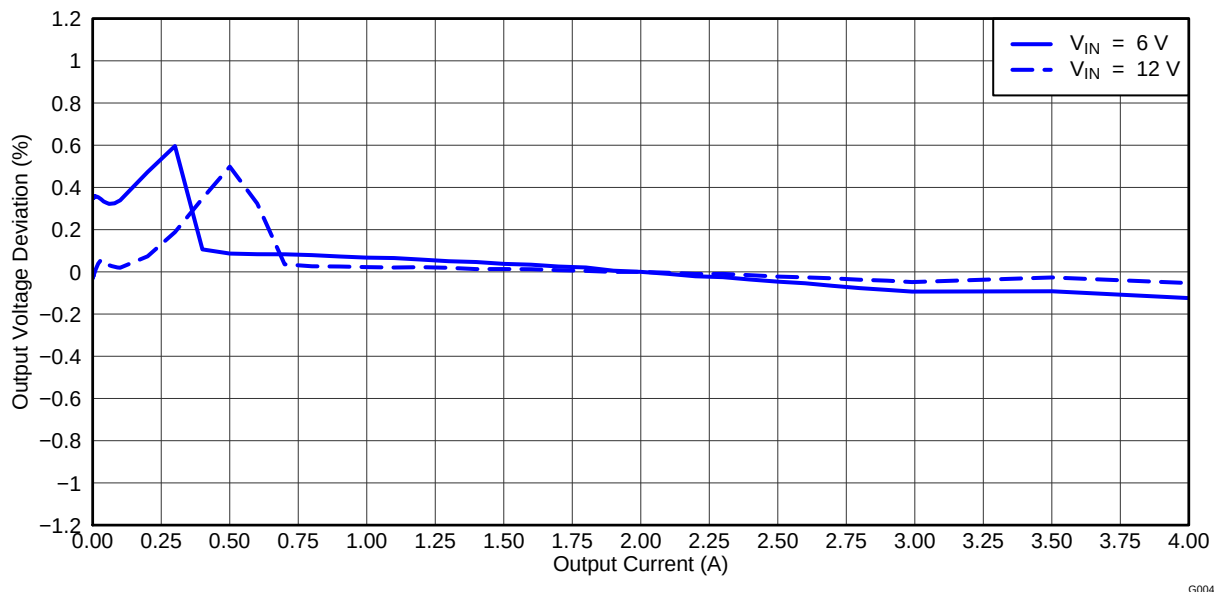
Figure 5. TPS54495EVM Converter 1 Load Regulation
