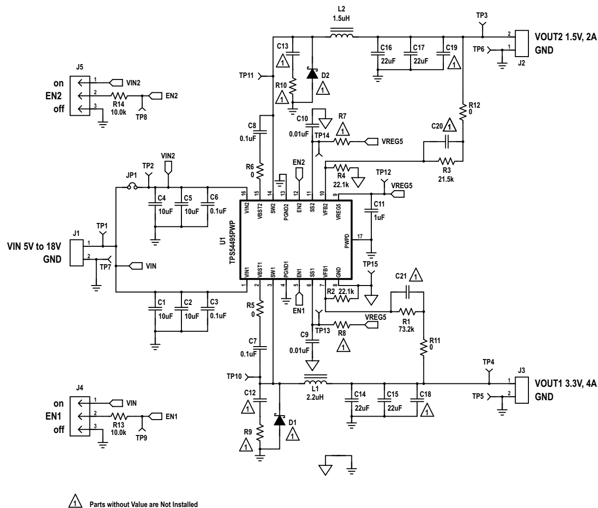
Figure 26. TPS54495EVM Schematic Diagram
