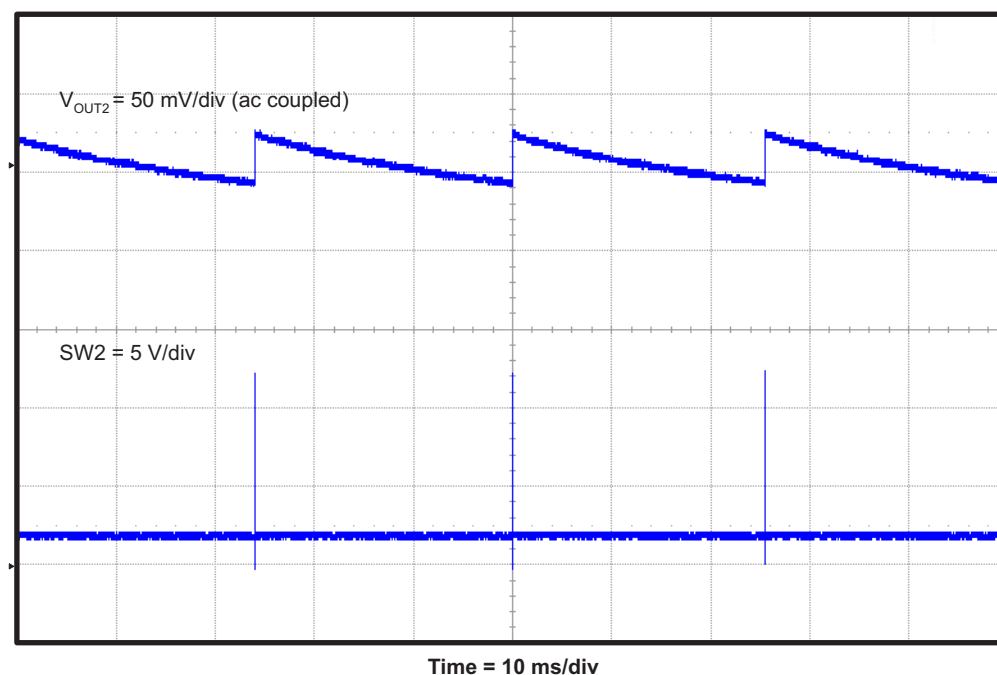
Figure 14. TPS54495EVM Converter 2 Eco-mode™ Output Voltage Ripple at No Load
