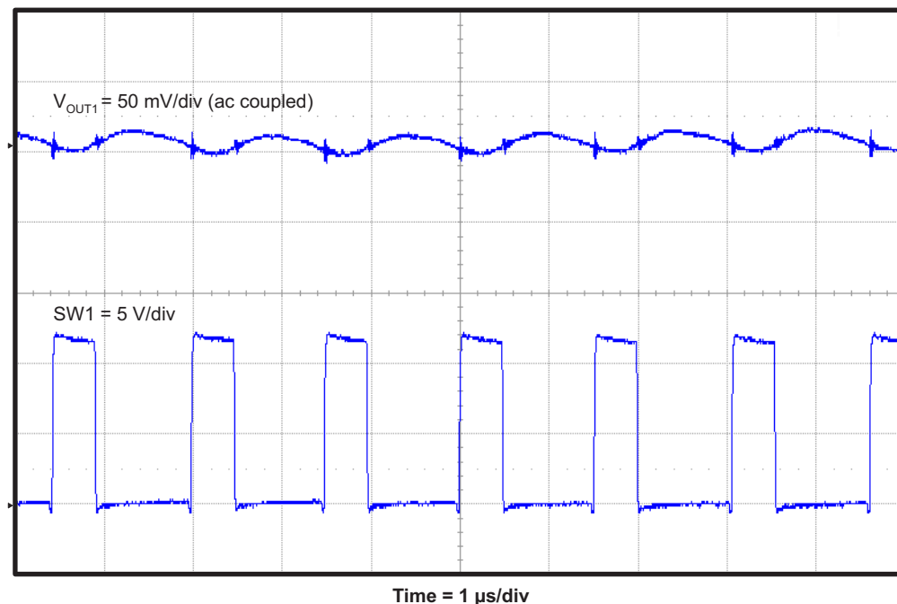
Figure 11. TPS54495EVM Converter 1 Output Voltage Ripple
