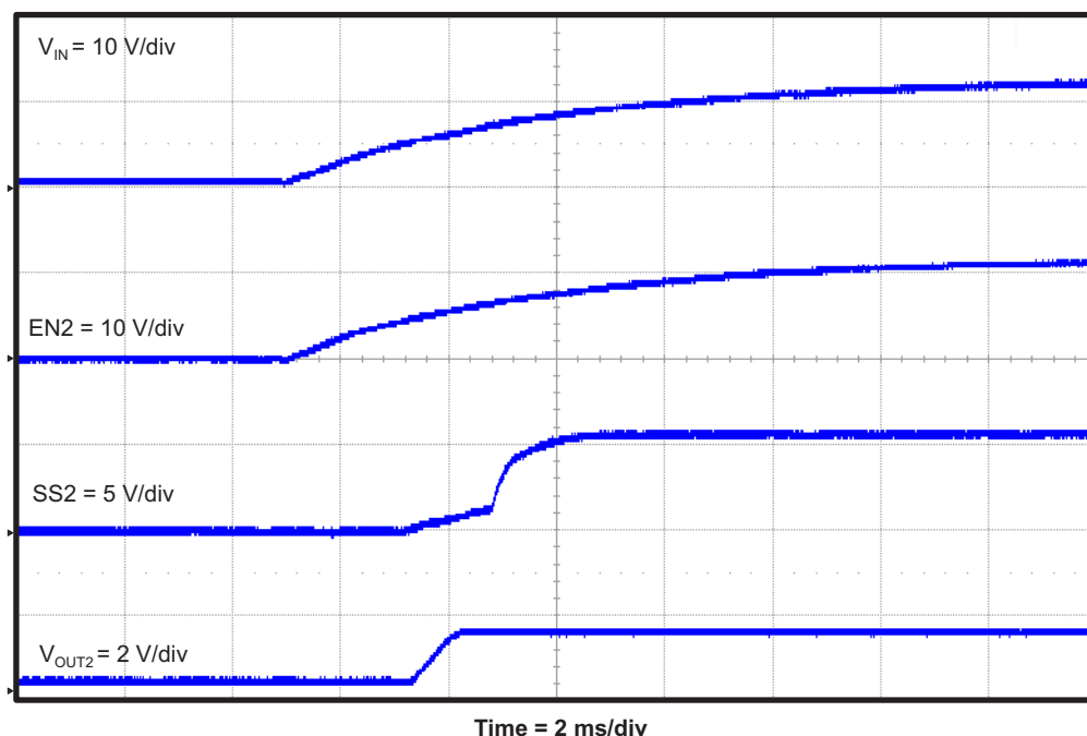
Figure 18. TPS54495EVM Converter 2 Start-Up Relative to V_{IN}
