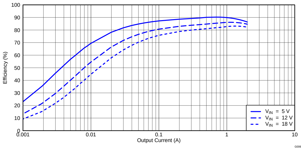
Figure 4. TPS54495EVM Converter 2 Light Load Efficiency
