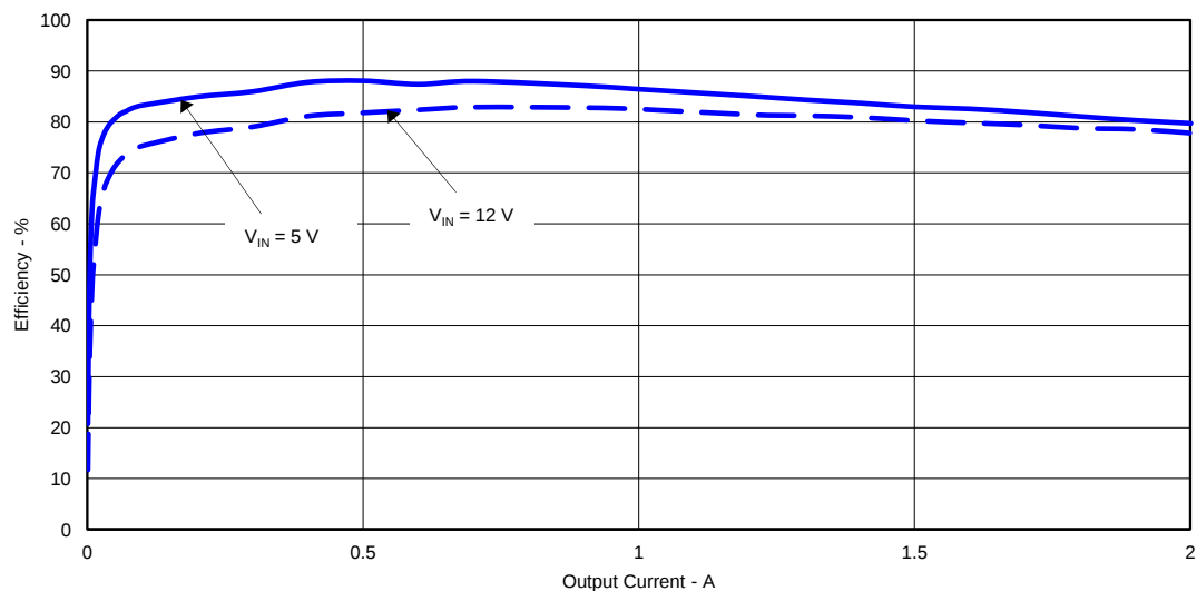
Figure 1. TPS54239EEVM-056 Efficiency
