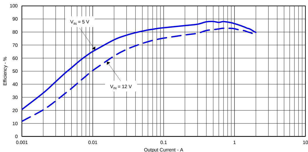
Figure 2. TPS54239EEVM-056 Light-Load Efficiency
