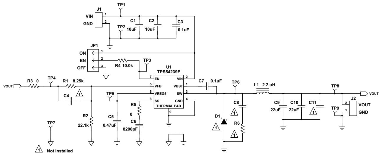
Figure 19. TPS54239EEVM-056 Schematic Diagram
