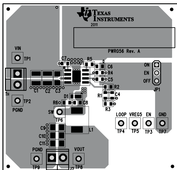
Figure 14. Top Assembly
