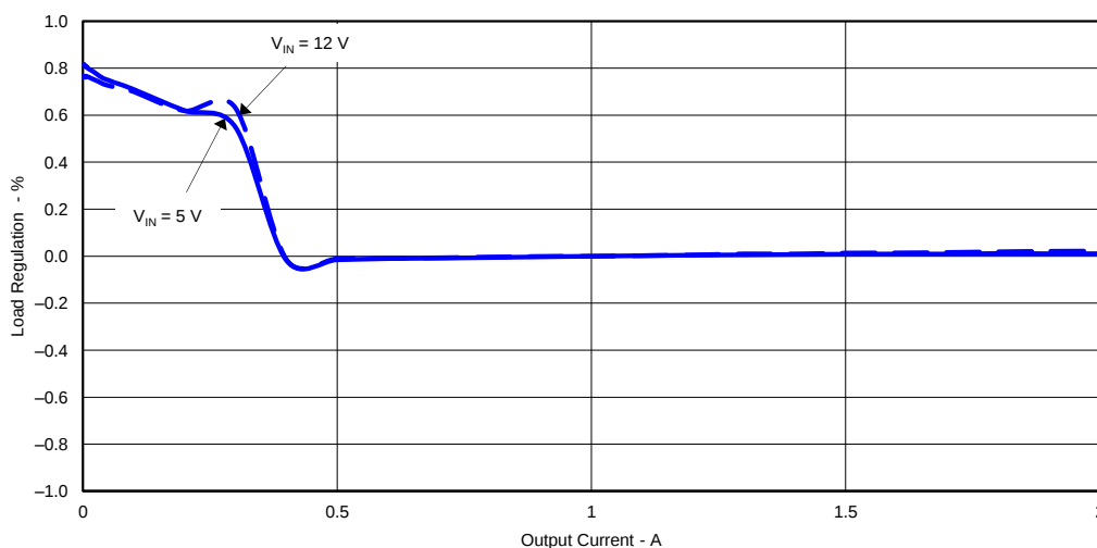
Figure 3. TPS54239EEVM-056 Load Regulation, V_{IN} = 5\text{ V} and V_{IN} = 12\text{ V} .
