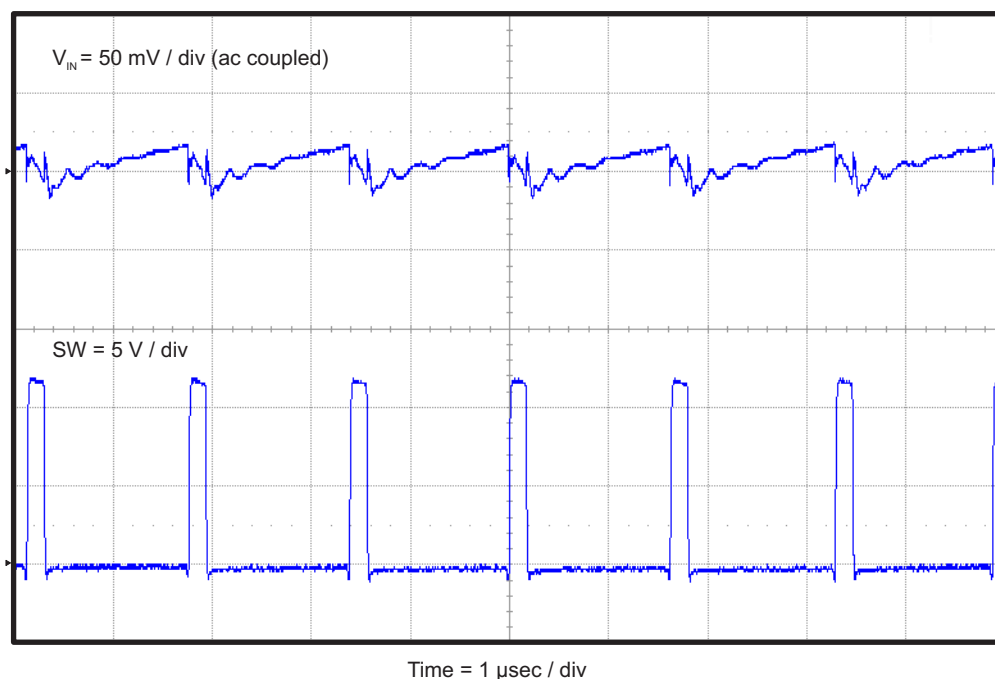
Figure 9. TPS54239EEVM-056 Input Voltage Ripple
