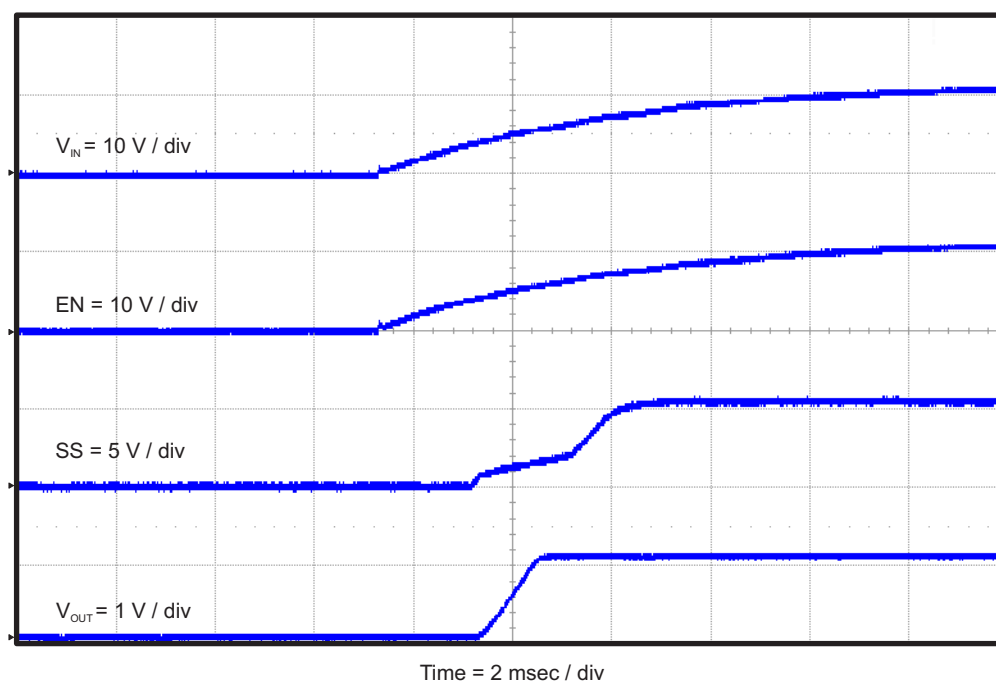
Figure 10. TPS54239EEVM-056 Start-Up Relative to V_{IN} with SS
