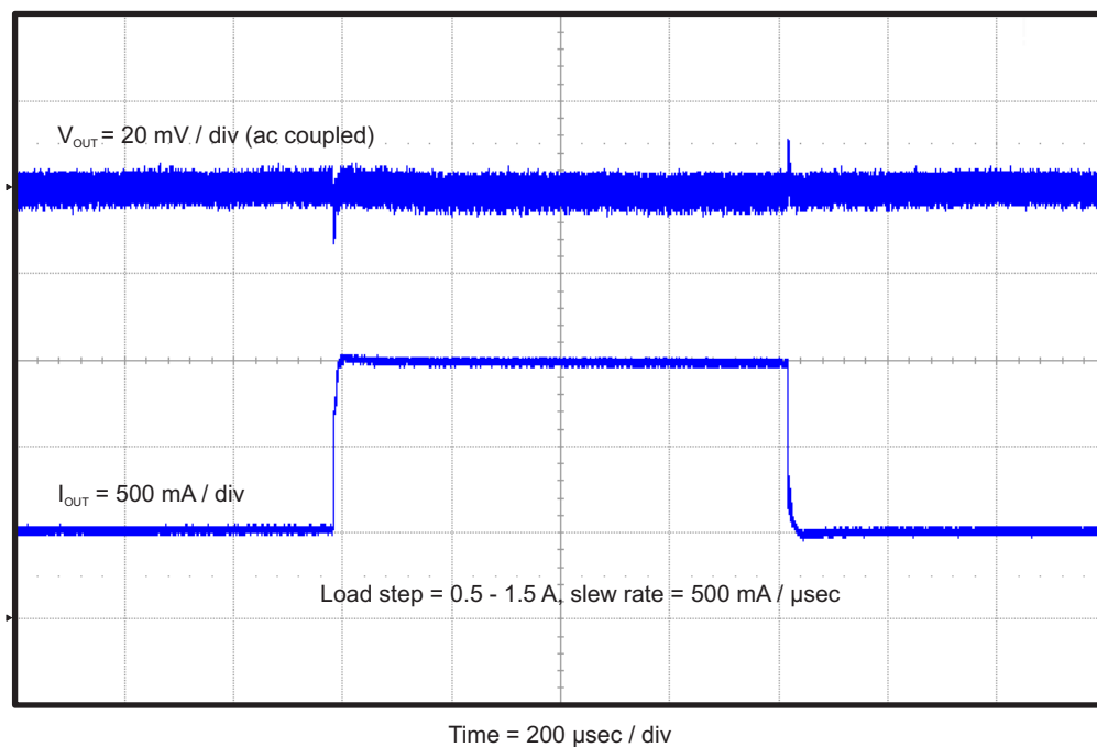
Figure 5. TPS54239EEVM-056 Load Transient Response
