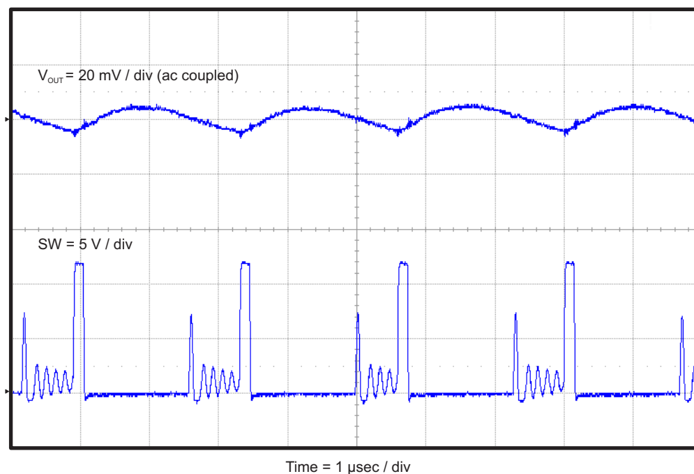
Figure 7. TPS54239EEVM-056 Output Voltage Ripple ( I_{OUT} = 50 \text{ mA} )
