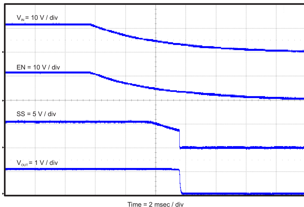
Figure 12. TPS54239EEVM-056 Shut-Down Relative to V_{IN} with SS
