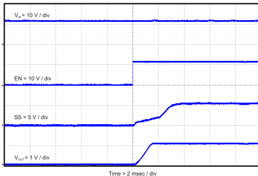
Figure 11. TPS54239EEVM-056 Start-Up Relative to EN with SS
