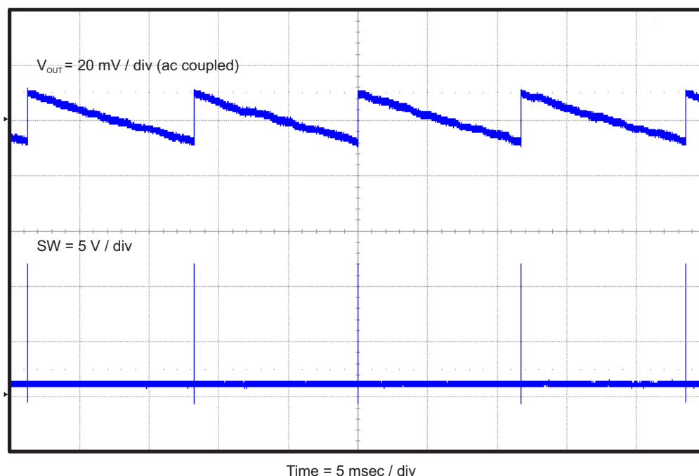
Figure 8. TPS54239EEVM-056 Output Voltage Ripple ( I_{OUT} = 0 \text{ A} )
