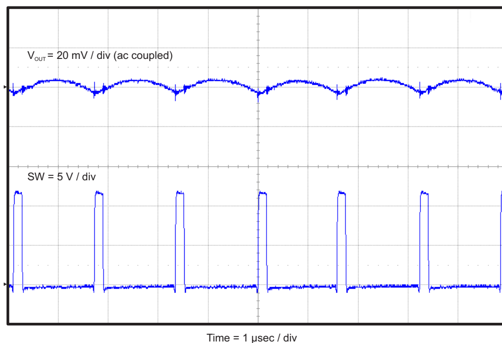
Figure 6. TPS54239EEVM-056 Output Voltage Ripple ( I_{OUT} = 2 \text{ A} )
