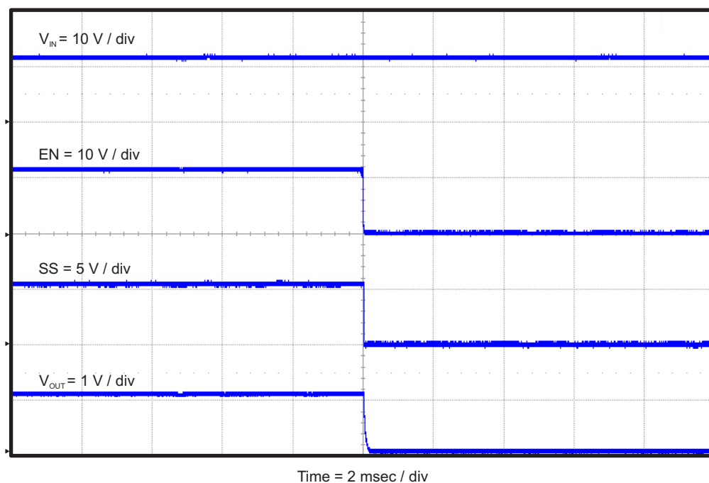
Figure 13. TPS54239EEVM-056 Shut-Down Relative to EN with SS
