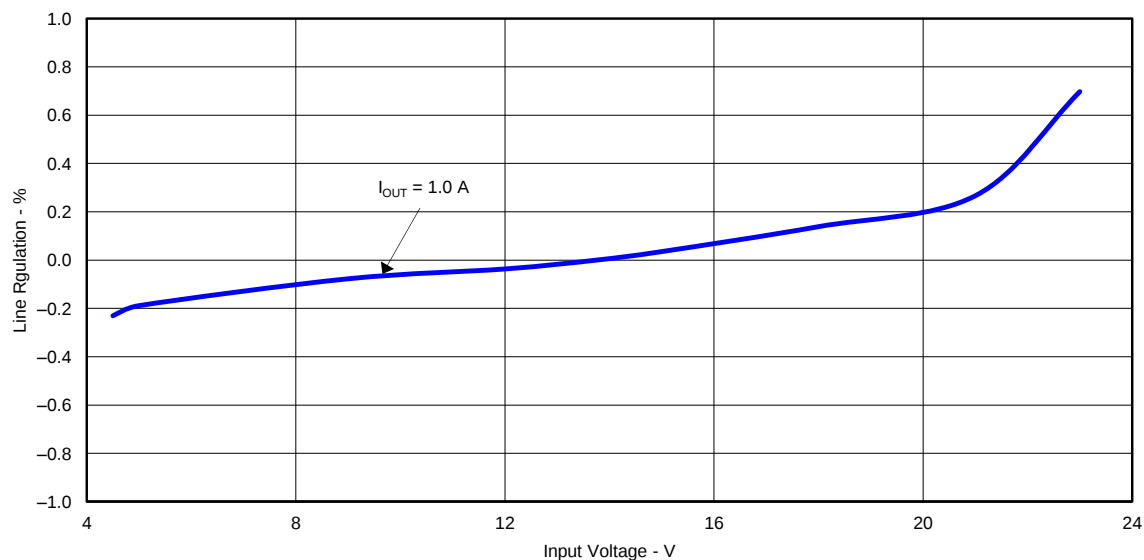
Figure 4. TPS54239EEVM-056 Line Regulation
