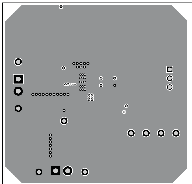
Figure 17. Internal Layer 2
