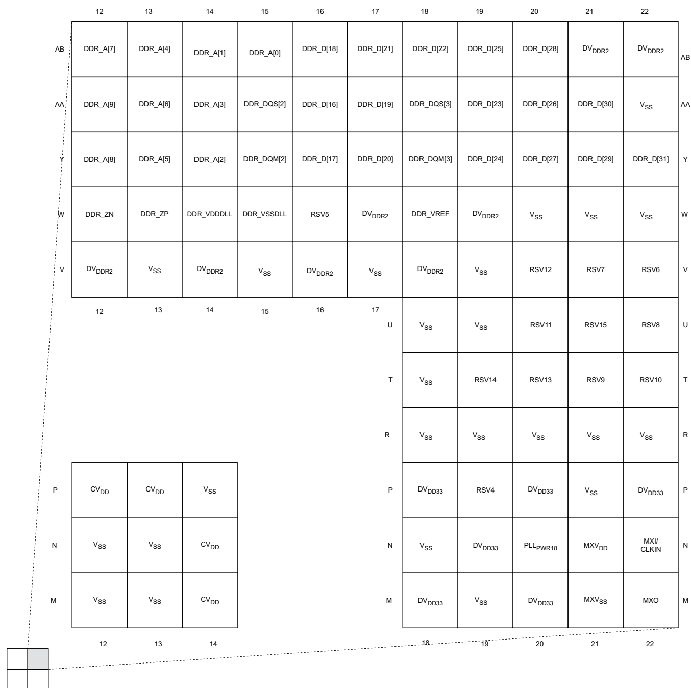
Figure 2-7. GDU Pin Map [Quadrant B]
