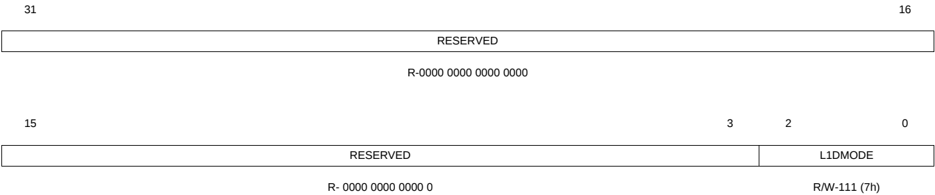
Figure 2-5. L1DCFG Register
