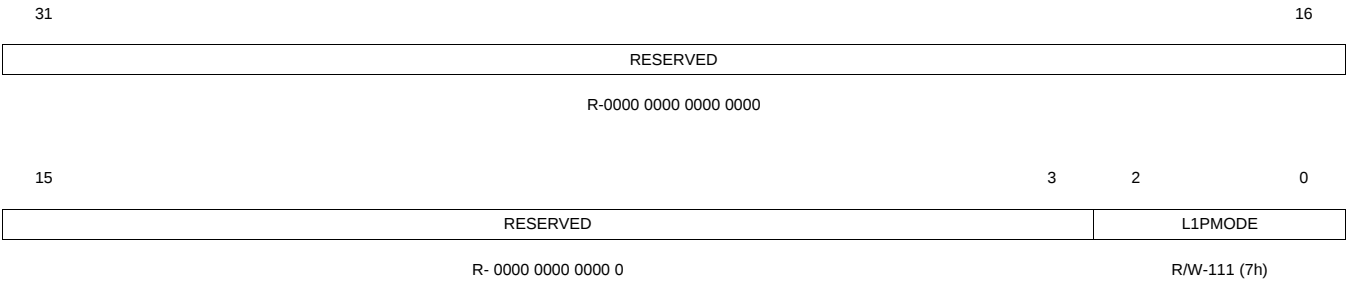
Figure 2-4. L1PCFG Register
