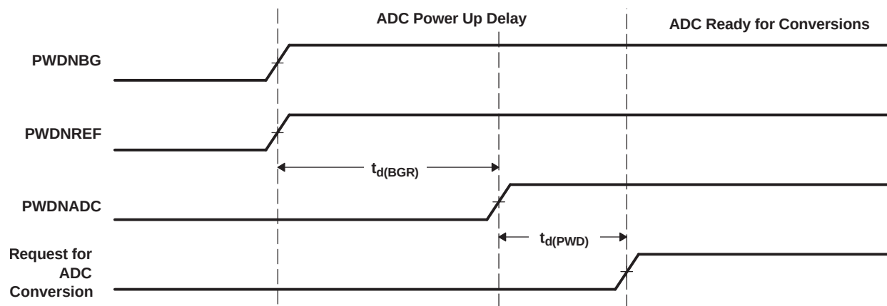
Figure 6-34. ADC Power-Up Control Bit Timing
