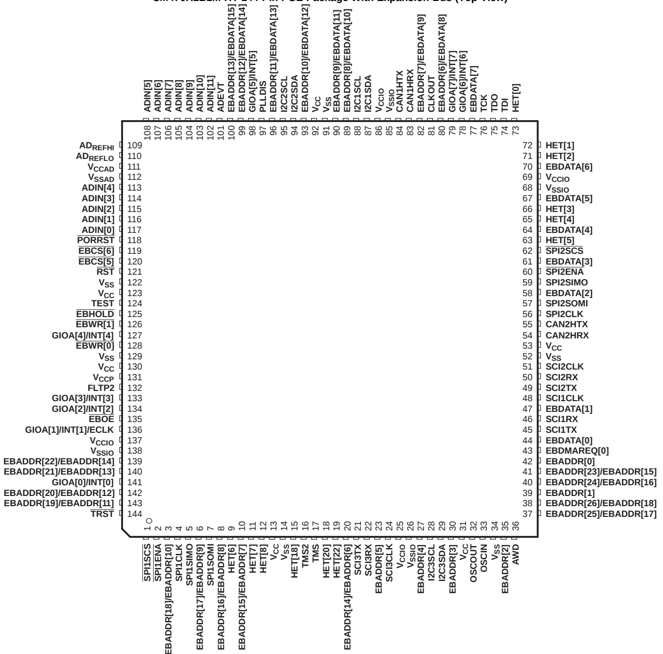
SM470R1B1M-HT 144-Pin PGE Package With Expansion Bus (Top View)
