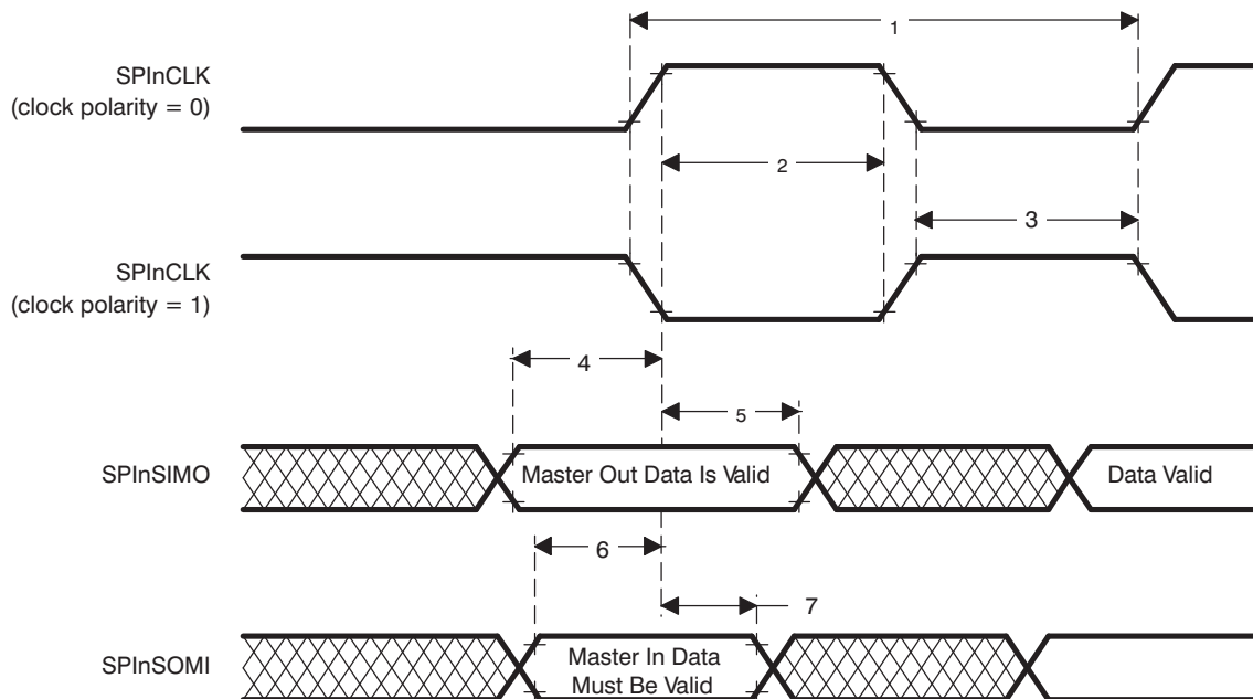
Figure 17. SPIn Master Mode External Timing (CLOCK PHASE = 1)
