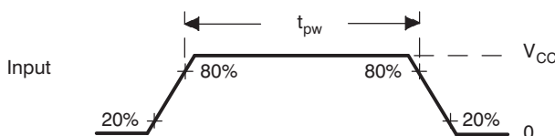
Figure 15. CMOS-Level Inputs
