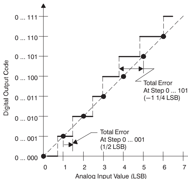
Figure 28. Absolute Accuracy (Total) Error
