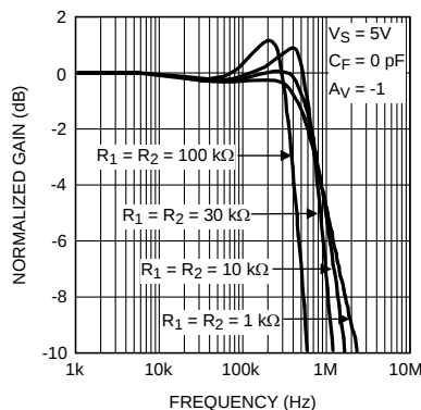
Figure 43. Closed Loop Gain vs. Frequency
