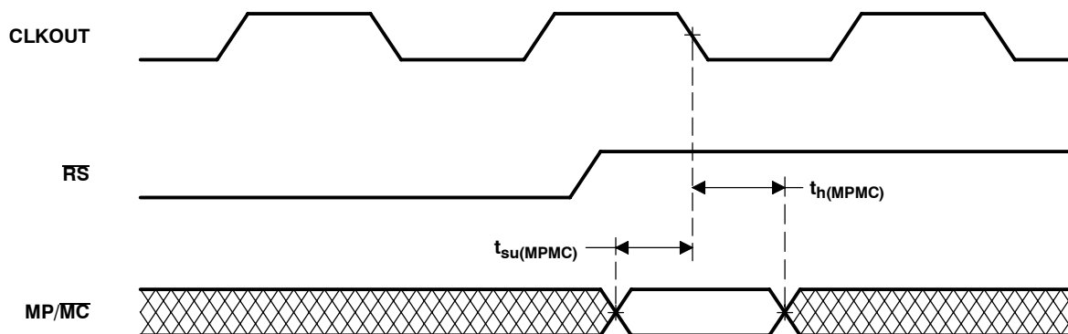
Figure 5-17. MP/ \overline{MC} Timing
