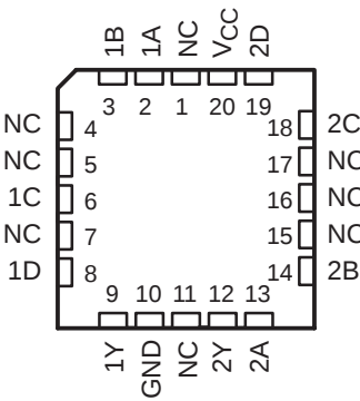
SN54F20 . . . FK PACKAGE (TOP VIEW)
