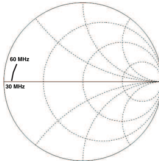
Figure 37. AIFOUT
