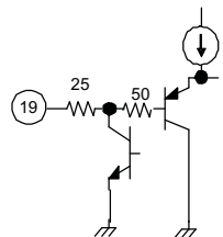
Figure 11. P5/ADC
