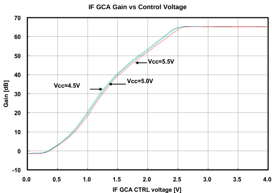
Figure 28. IF GCA Gain vs Control Voltage
