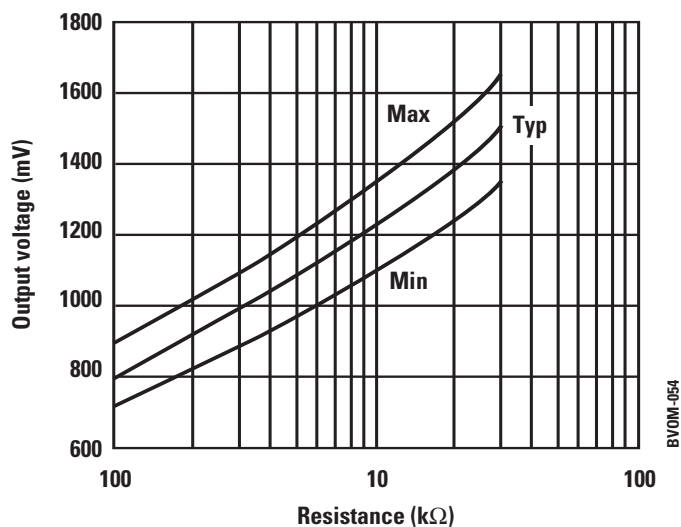
Figure 2.27. Voltage adjustment resistance vs. output voltage
