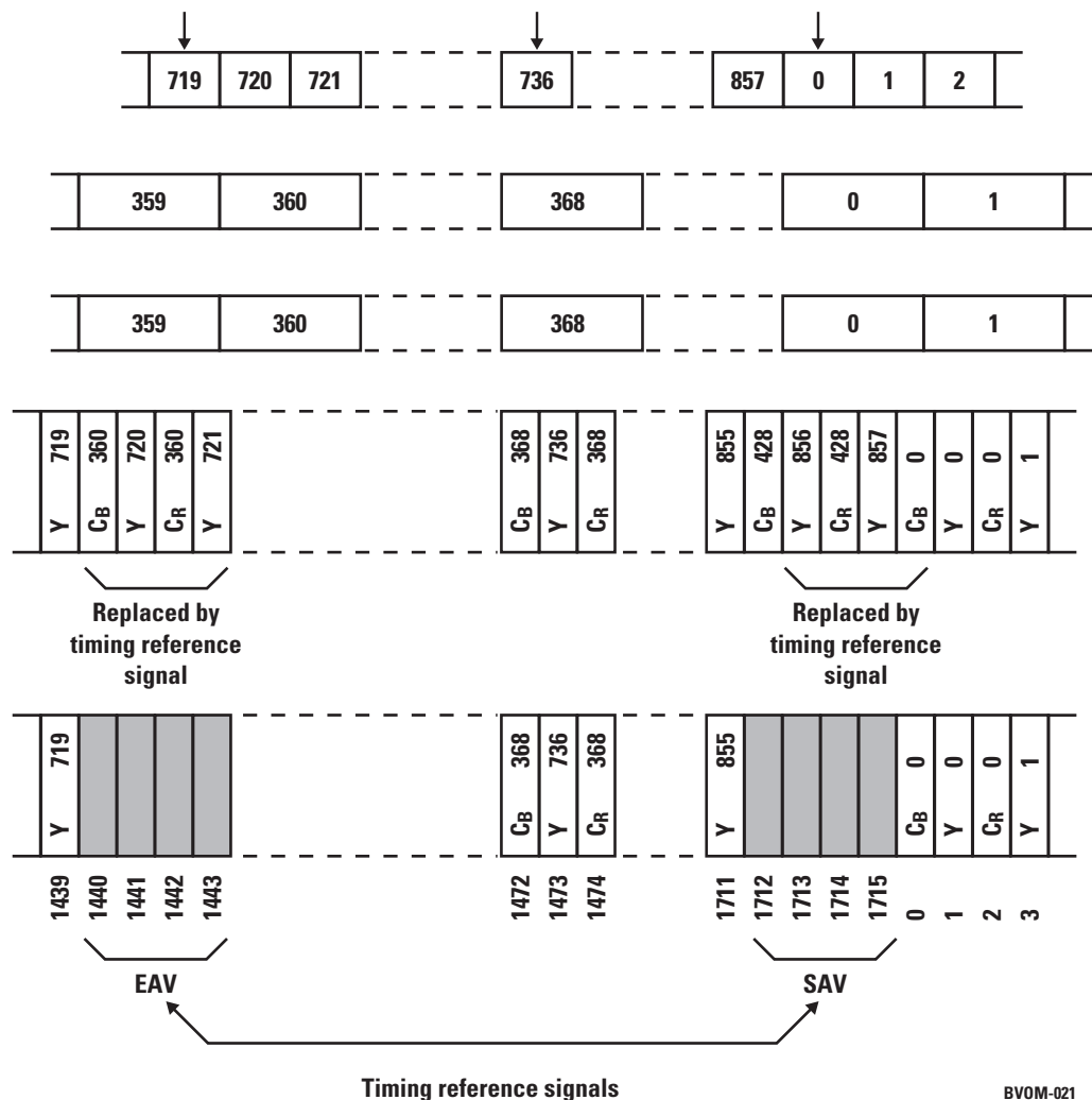
Figure 1.1. Example of multiplex data structure
