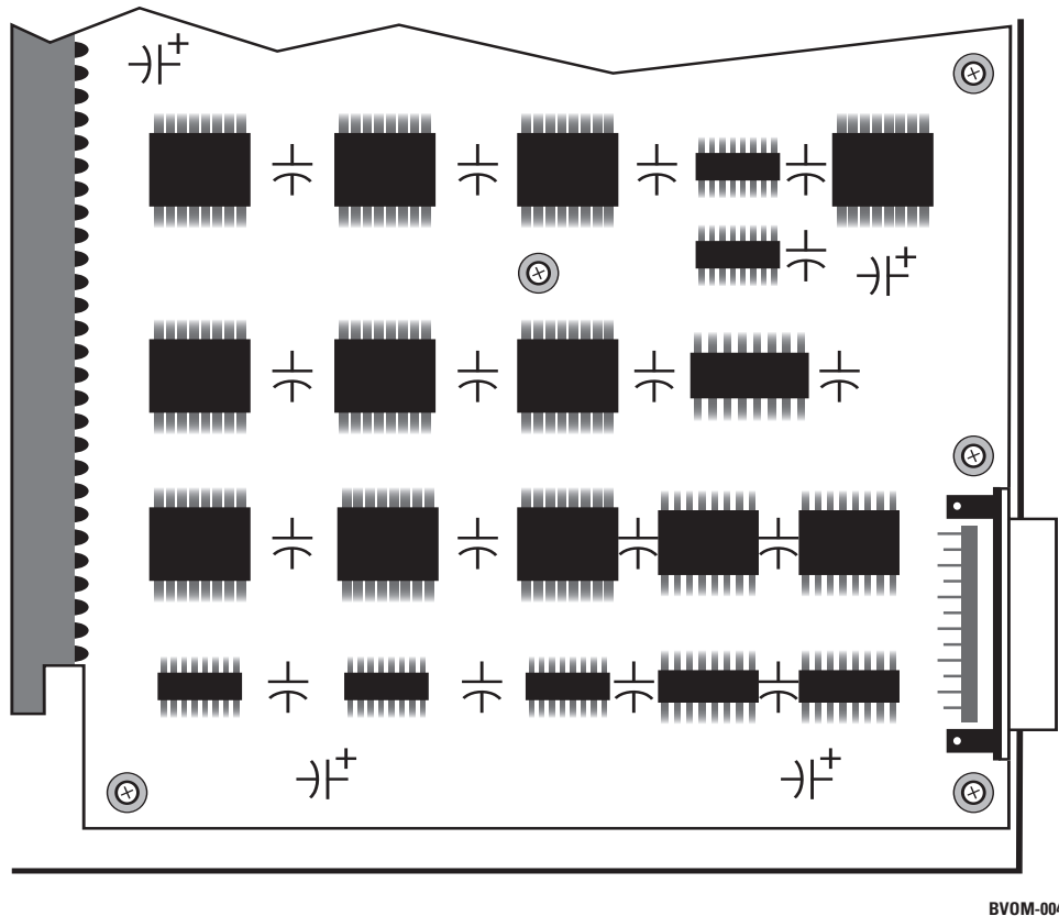
Figure 2.3. The result of adequate bypassing
