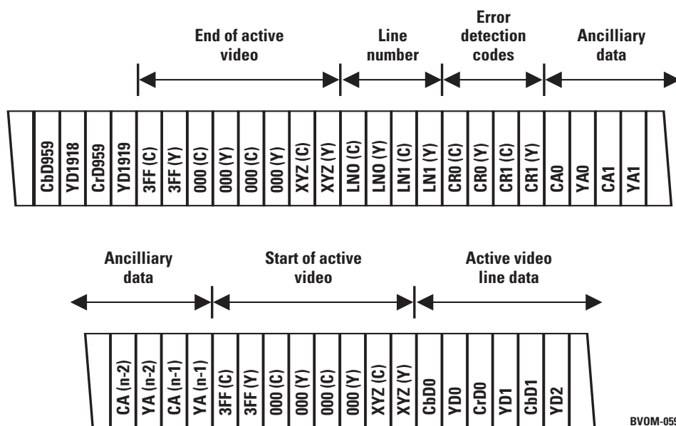
Figure 4.3. HDTV video line data sequence
