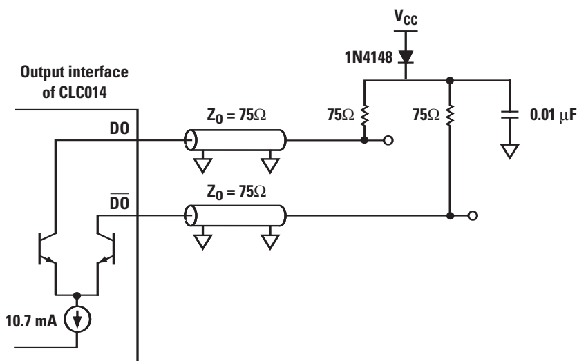
Figure 2.31. ECL-compatible output
