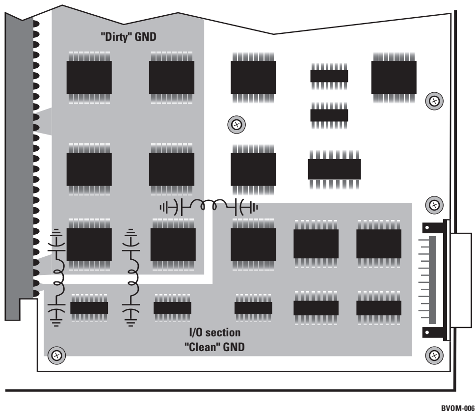
Figure 2.5. Isolate noisy components
