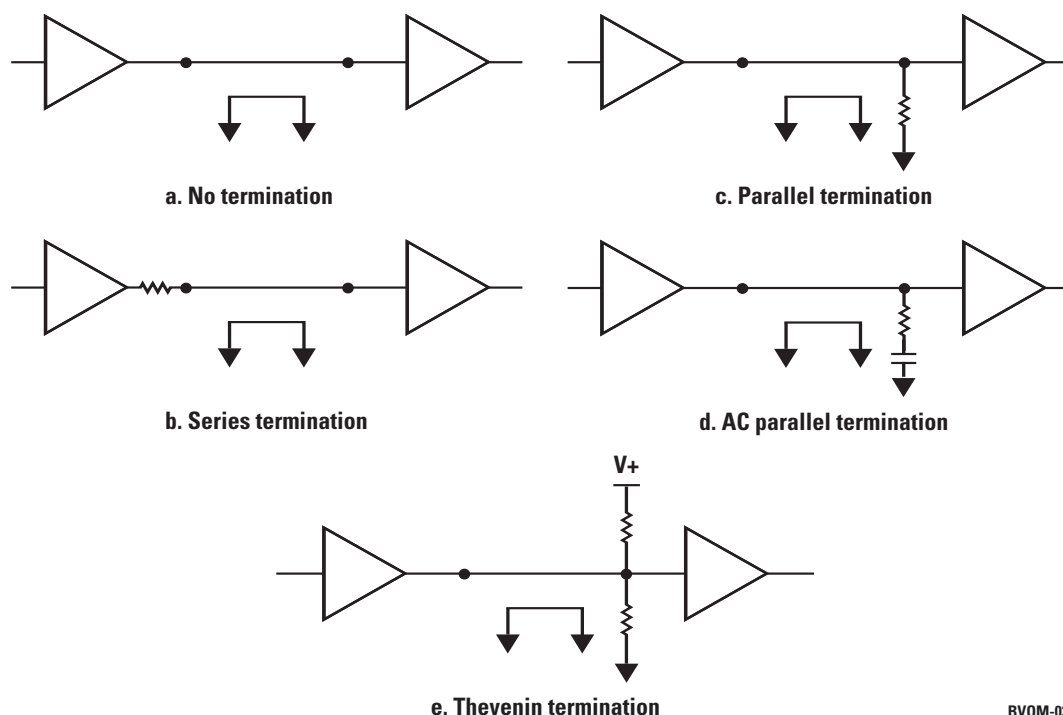
Figure 2.15. Single-ended termination
