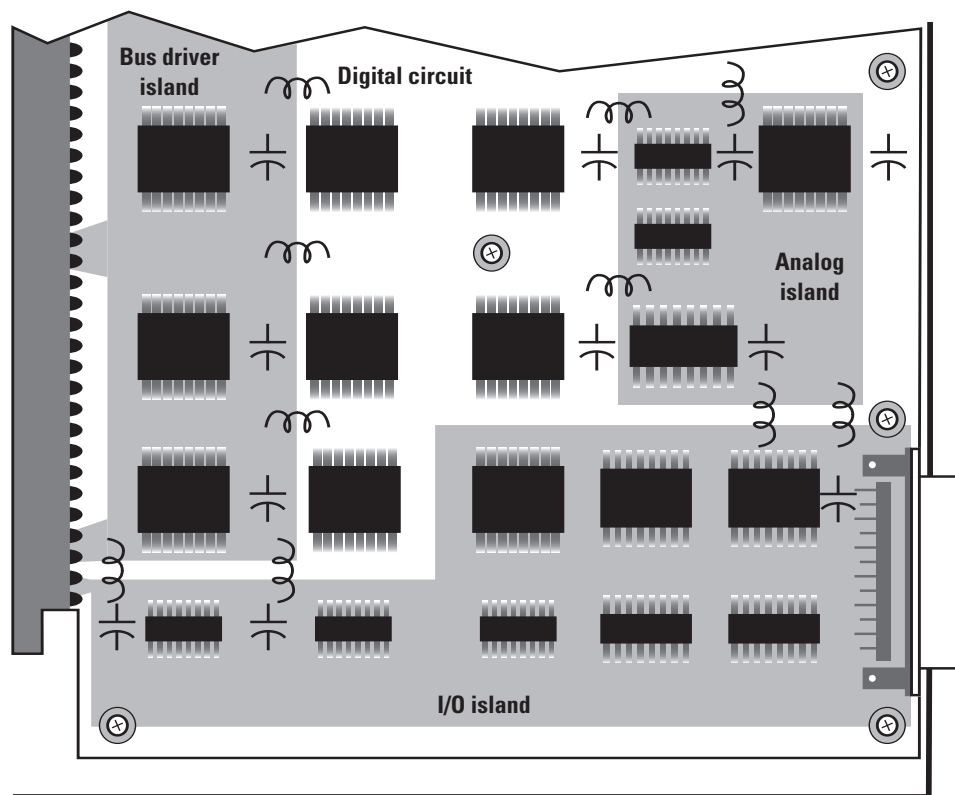
Figure 2.4. PCB organization and partitioning
