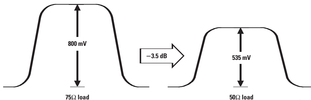
Figure 2.32. Effect of 50\Omega load on output level
