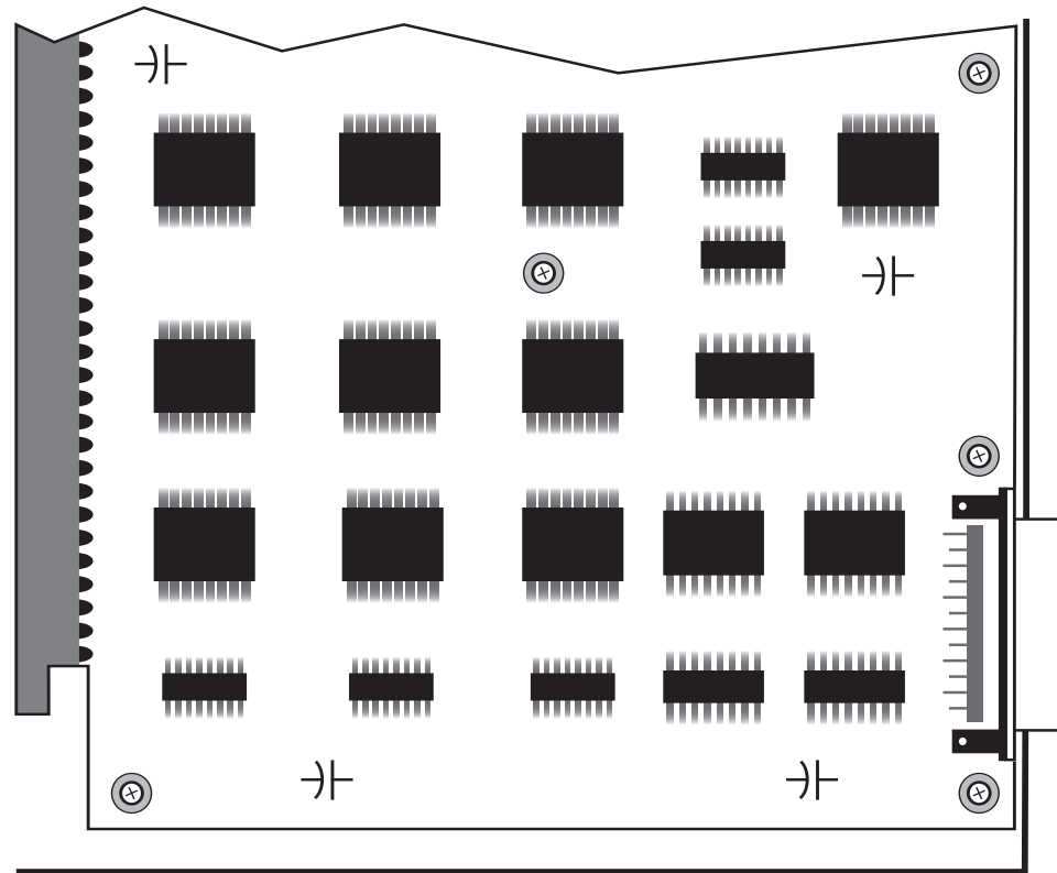
Figure 2.2. Insufficient bypassing
