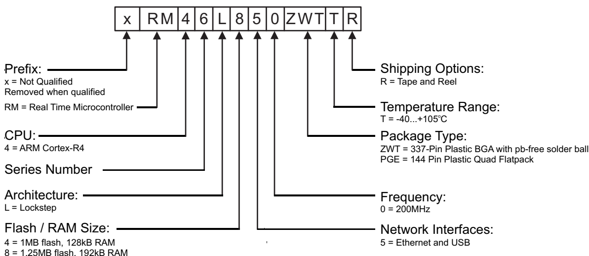
Figure 6-1. RM46Lx50 Device Numbering Conventions
