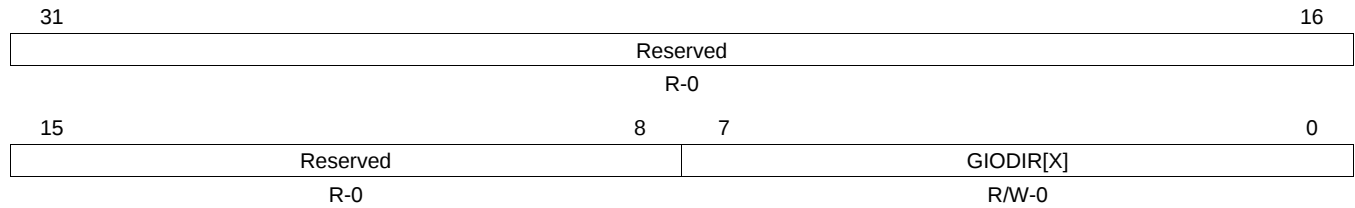
Figure 19-17. GIO Data Direction Registers [A-H][7:0] (IODIR[A-H]) [address = FFF7BC34h, FFF7BC54h, FFF7BC74h, FFF7BC94h, FFF7BCB4h, FFF7BCD4h, FFF7BCF4h, FFF7BD14h]
