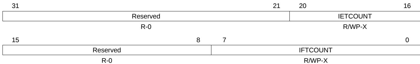
Figure 18-45. Initial Transfer Count Register (HTU ITCOUNT)
