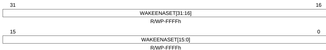
Figure 14-29. Wake-Up Enable Set Register 0 (WAKEENASET0) [offset = FFFF FE50h]
