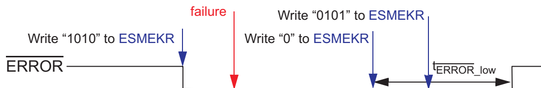
Figure 11-9. ERROR Pin Timing - Example 6
