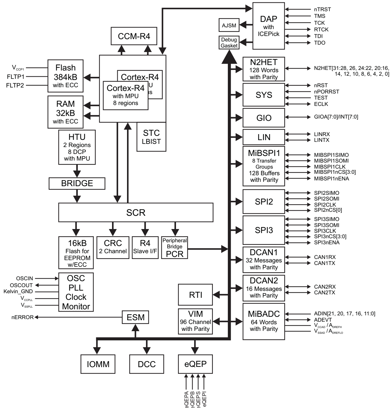
Figure 1-1. Block Diagram
