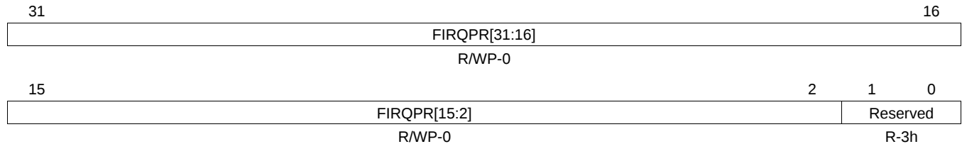
Figure 14-17. FIQ/IRQ Program Control Register 0 (FIRQPR0) [offset = FFFF FE10h]
