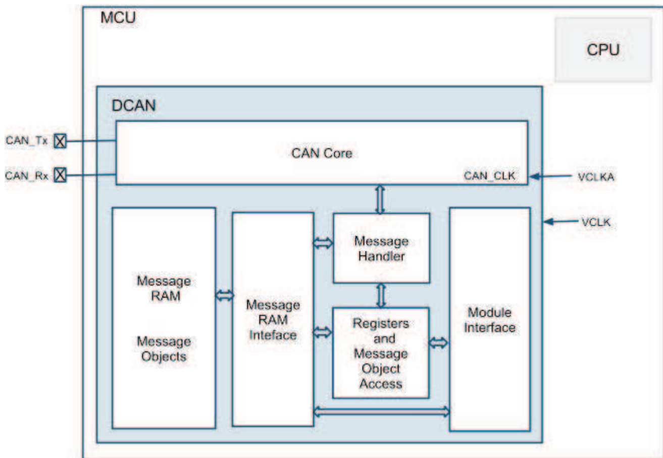
Figure 20-1. Block Diagram
