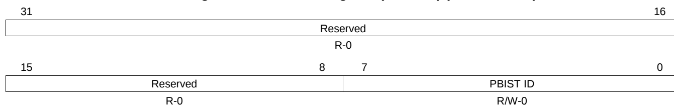
Figure 6-7. PBIST ID Register (PBISTID) (offset = 184h)
