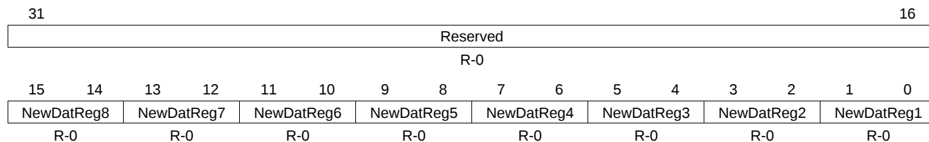
Figure 20-32. New Data X Register (DCAN NWDAT X) [offset = 98h]
