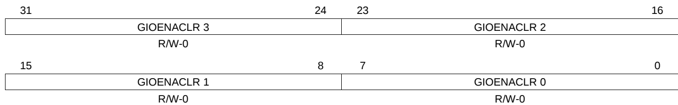
Figure 19-9. GIO Interrupt Enable Clear Register (GIOENACLR) [address = FFF7 BC14h]
