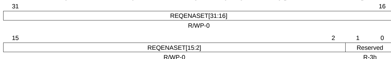
Figure 14-23. Interrupt Enable Set Register 0 (REQENASET0) [offset = FFFF FE30h]
