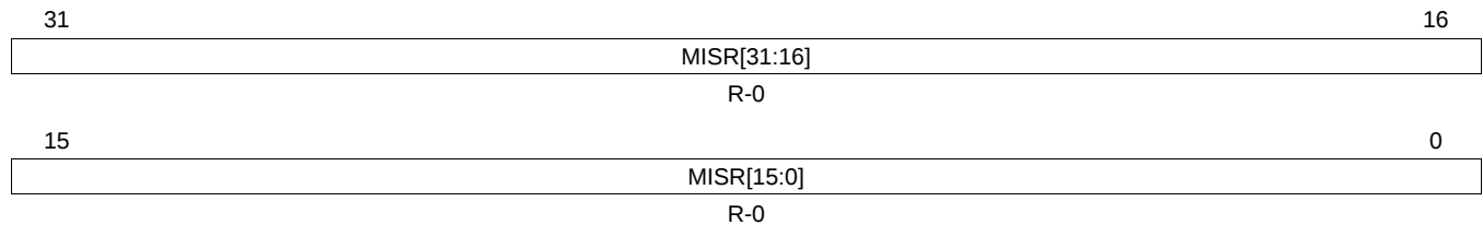
Figure 7-14. CPU2 Current MISR Register (CPU2_CURMISR3) (offset = 2Ch)
