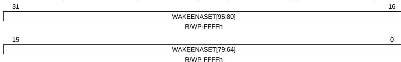
Figure 14-31. Wake-Up Enable Set Register 2 (WAKEENASET2) [offset = FFFF FE58h]
