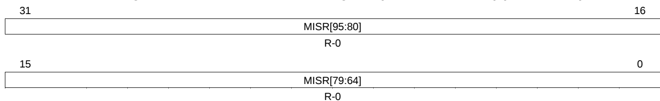
Figure 7-12. CPU1 Current MISR Register (CPU1_CURMISR1) (offset = 24h)
