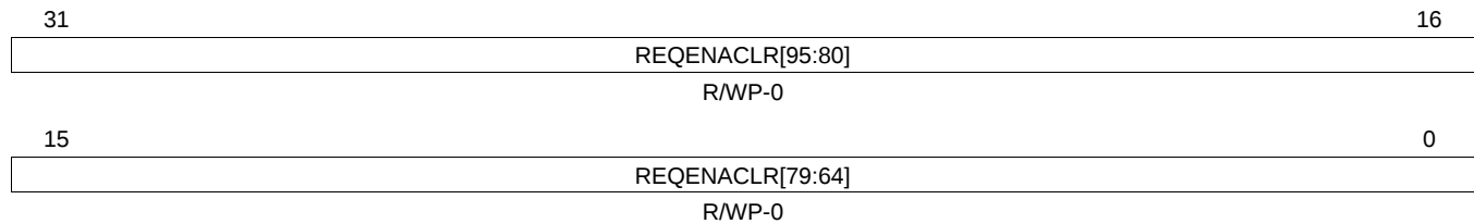
Figure 14-28. Interrupt Enable Clear Register 2 (REQENACLR2) [offset = FFFF FE48h]
