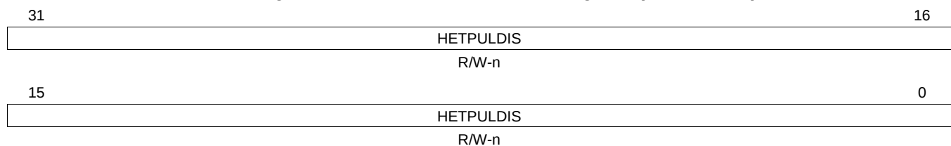
Figure 17-57. N2HET Pull Disable Register (HETPULDIS)
