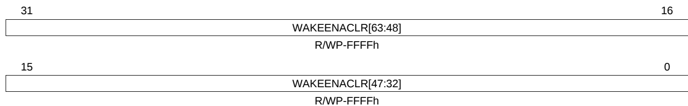
Figure 14-33. Wake-Up Enable Clear Register 1 (WAKEENACLR1) [offset = FFFF FE64h]
