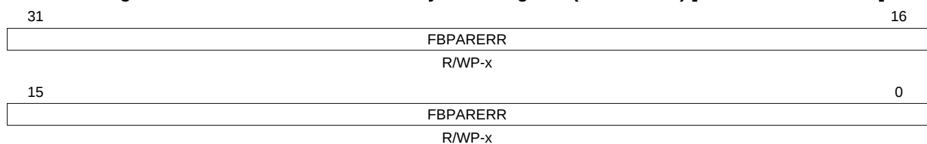
Figure 14-14. Fall-Back Address Parity Error Register (FBPARERR) [Offset = FFFF FDF8h]
