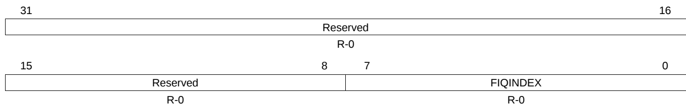
Figure 14-16. FIQ Index Offset Vector Register (FIQINDEX) [Offset = FFFF FE04h]
