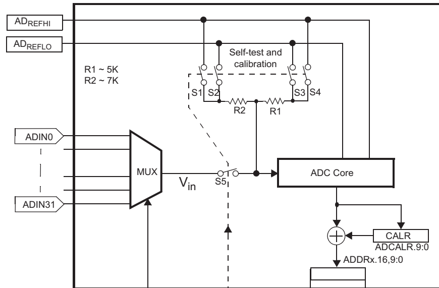
Figure 16-14. Self-Test and Calibration Logic
