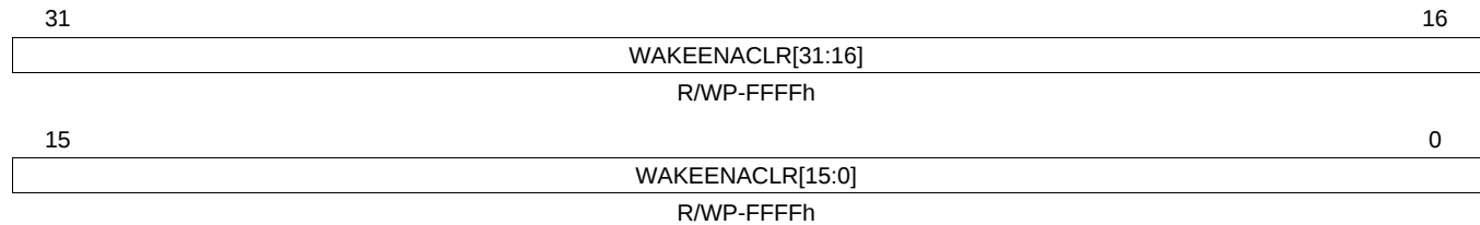
Figure 14-32. Wake-Up Enable Clear Register 0 (WAKEENACLR0) [offset = FFFF FE60h]
