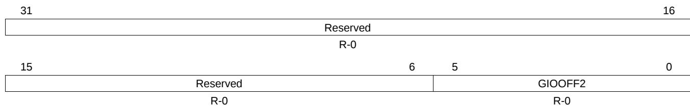
Figure 19-14. GIO Offset 2 Register (GIOFF2) [address = FFF7 BC28h]
