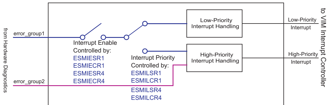
Figure 11-2. Interrupt Response Handling
