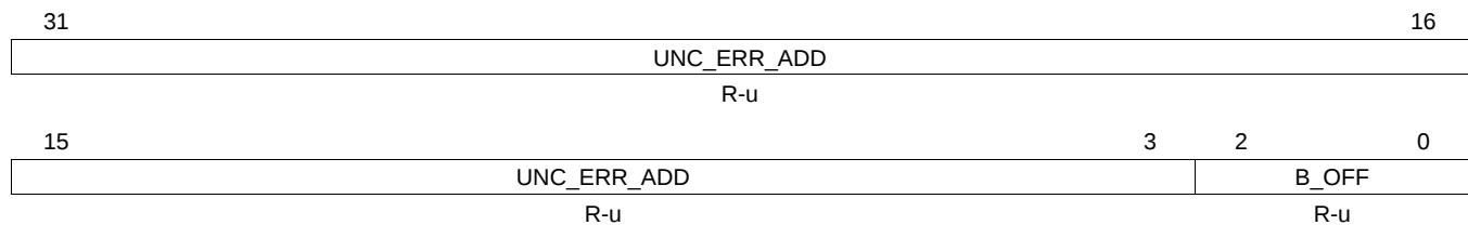
Figure 4-47. EEPROM Emulation Uncorrectable Error Address Register (EE_UNC_ERR_ADD) (offset = 320h)
