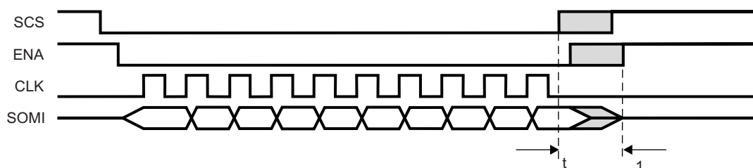
Figure 21-38. Transmit-Data-Finished-to-ENA-Inactive-Timeout
