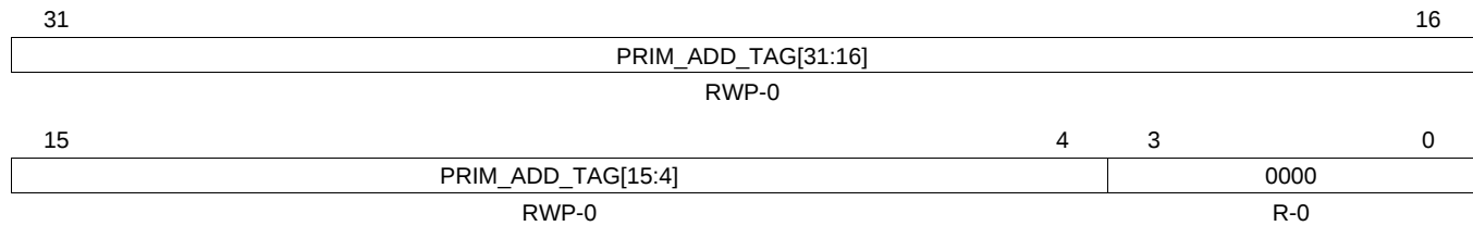
Figure 4-16. Primary Address Tag Register (FPRIM_ADD_TAG) (offset = 28h)
