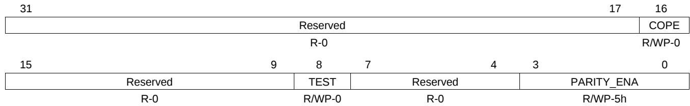
Figure 18-37. Parity Control Register (HTU PCR) [offset = 64h]
