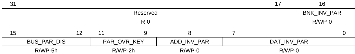
Figure 4-36. Parity Override Register (FPAR_OVR) (offset = 7Ch)
