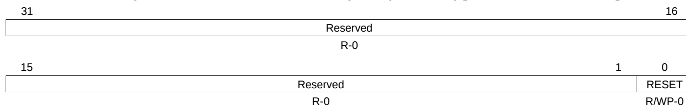
Figure 19-5. GIO Global Control Register (GIOGCR0) [address = FFF7 BC00h]
