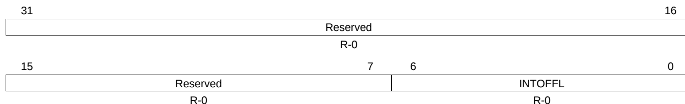
Figure 11-22. ESM Interrupt Offset Low Register (ESMIOFFLR) [offset = FFFF F52Ch]
