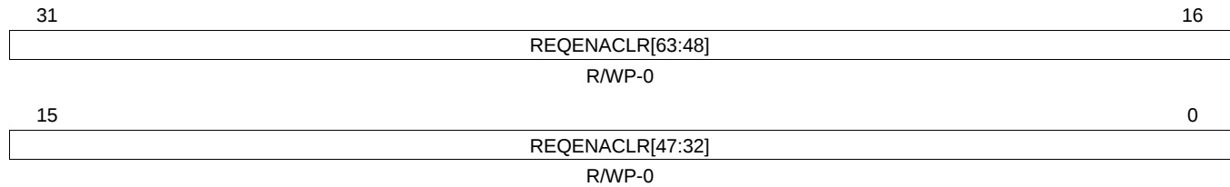
Figure 14-27. Interrupt Enable Clear Register 1 (REQENACLR1) [offset = FFFF FE44h]
