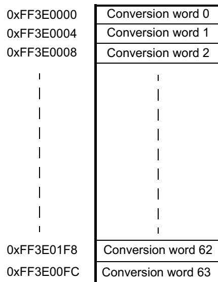
Figure 16-5. ADC Memory Mapping
