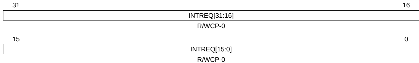
Figure 14-20. Pending Interrupt Read Location Register 0 (INTREQ0) [offset = FFFF FE20h]
