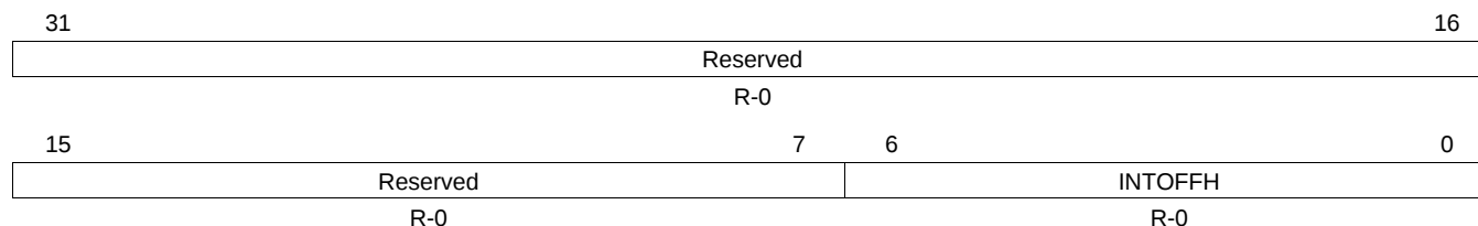
Figure 11-21. ESM Interrupt Offset High Register (ESMIOFFHR) [offset = FFFF F528h]
