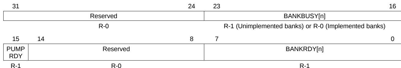
Figure 4-23. Flash Bank/Pump Ready Register (FBPRDY) (offset = FFF8 7044h)
