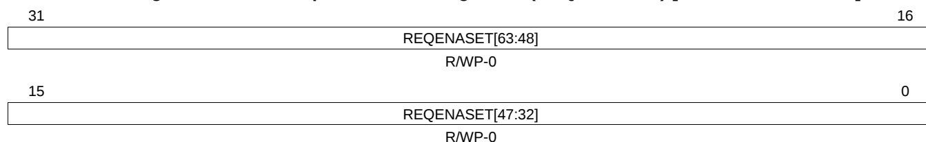
Figure 14-24. Interrupt Enable Set Register 1 (REQENASET1) [offset = FFFF FE34h]
