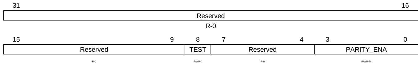
Figure 17-59. Parity Control Register (HETPCR)
