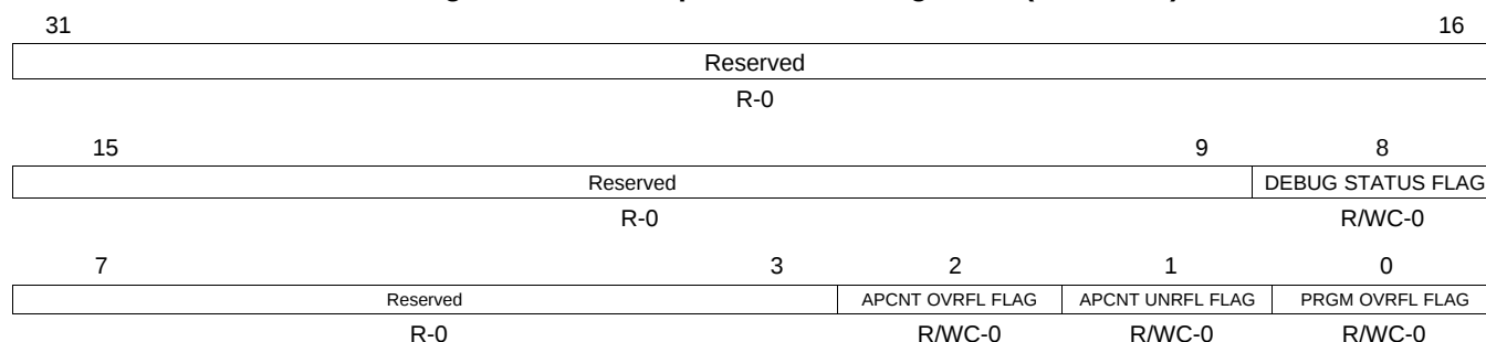
Figure 17-43. Exception Control Register 2 (HETEXC2)
