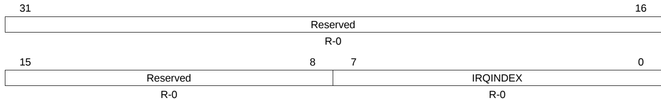
Figure 14-15. IRQ Index Offset Vector Register (IRQINDEX) [Offset = FFFF FE00h]
