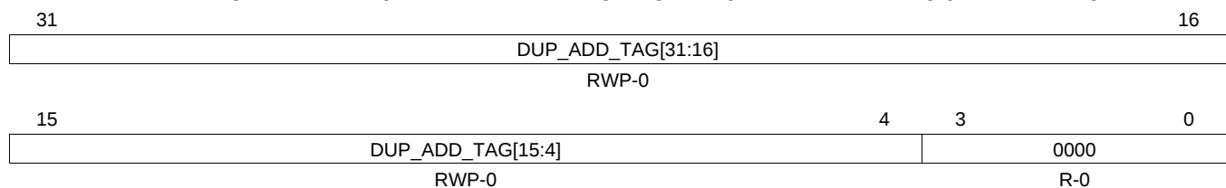
Figure 4-17. Duplicate Address Tag Register (FDUP_ADD_TAG) (offset = 2Ch)
