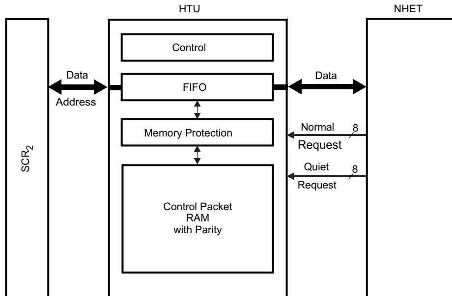
Figure 18-2. HTU Block Diagram
