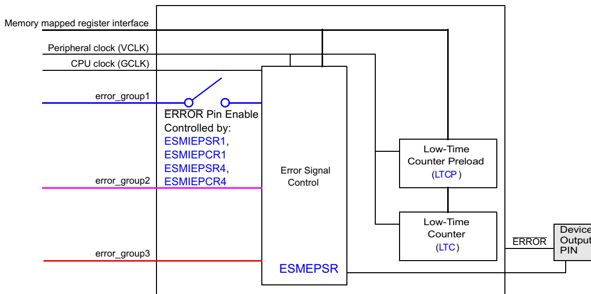
Figure 11-3. \overline{\text{ERROR}} Pin Response Handling
