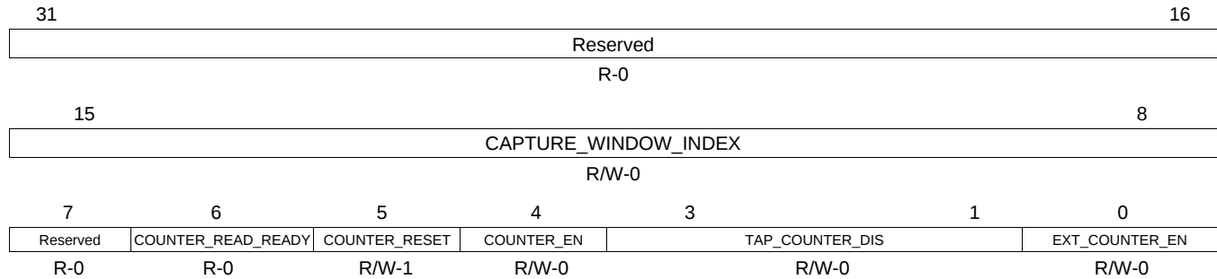
Figure 9-6. SSW PLL BIST Control Register 1 (SSWPLL1) (offset = 24h)
