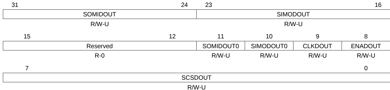
Figure 21-25. SPI Pin Control Register 3 (SPIPC3) [offset = 20h]
