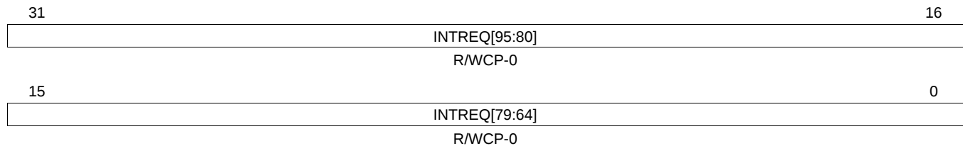
Figure 14-22. Pending Interrupt Read Location 2 (INTREQ2) Register [offset = FFFF FE28h]
