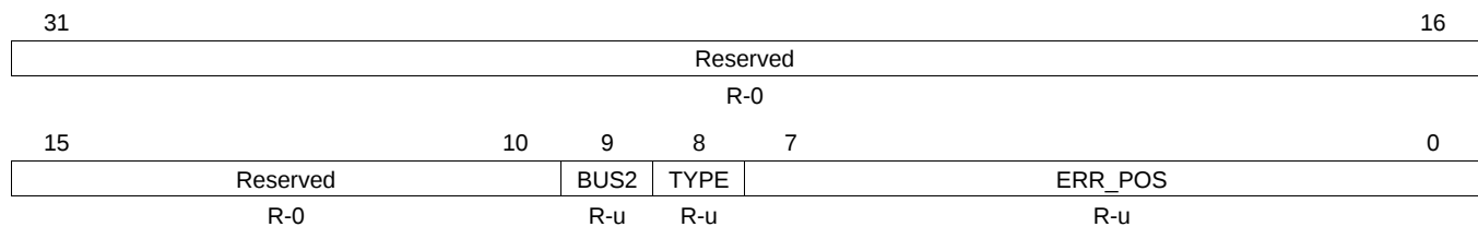
Figure 4-12. Flash Correctable Error Position Register (FCOR_ERR_POS) (offset = 18h)
