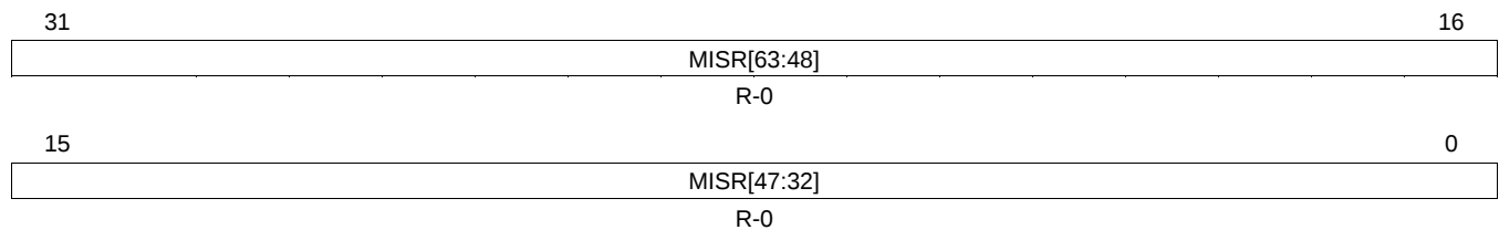
Figure 7-15. CPU2 Current MISR Register (CPU2_CURMISR2) (offset = 30h)
