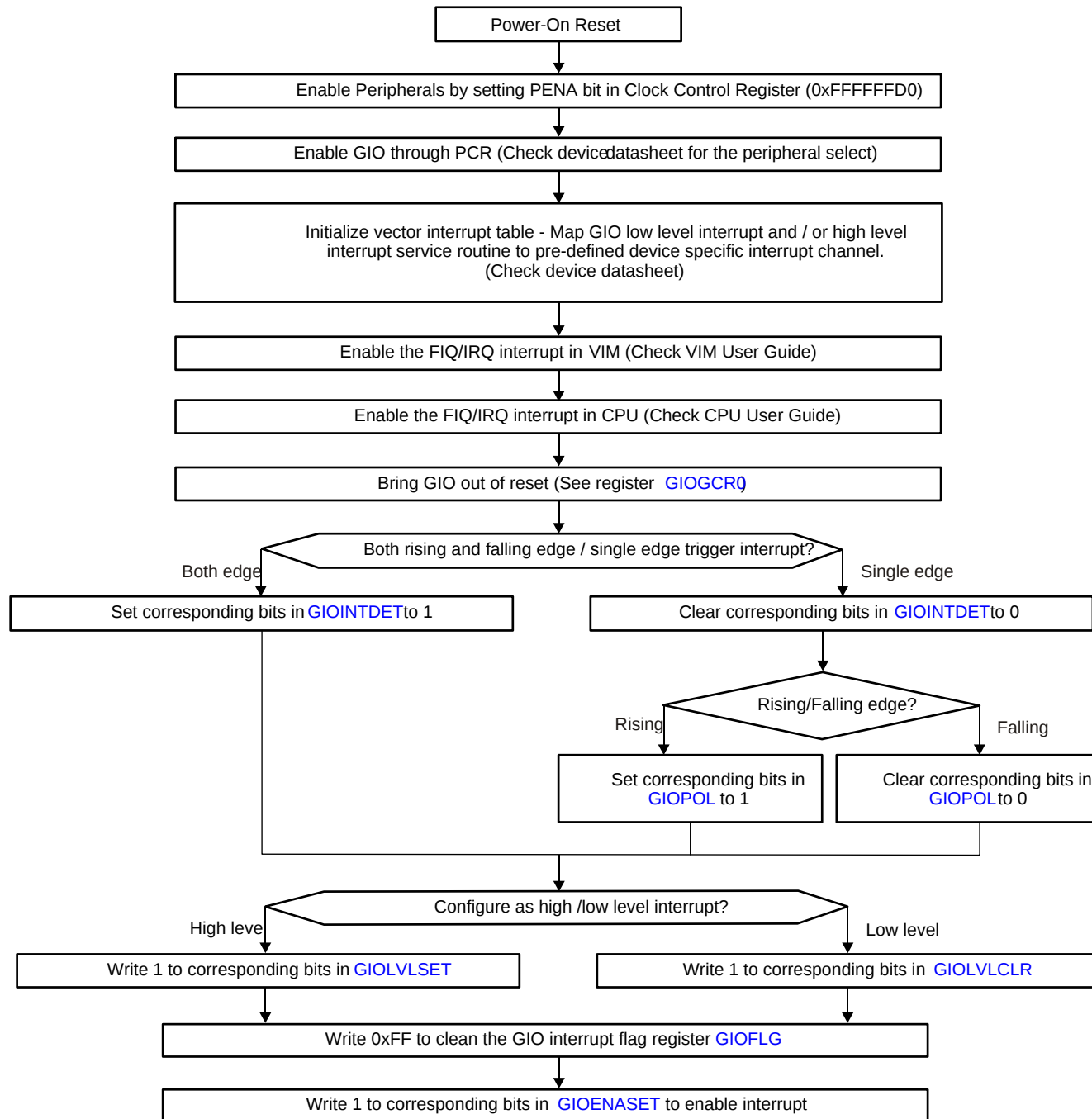
Figure 19-3. Interrupt Generation Function Quick Start Flow Chart
