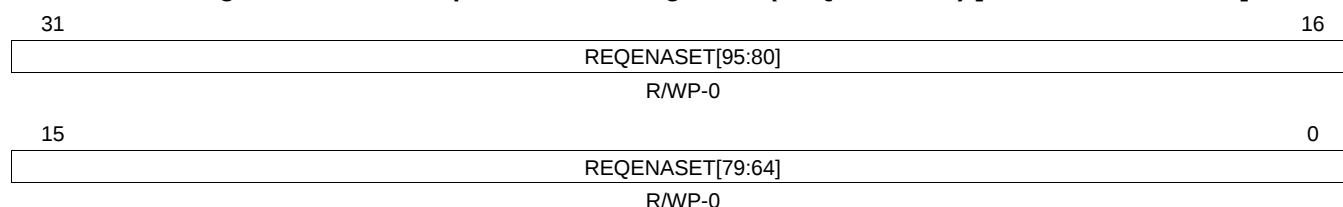
Figure 14-25. Interrupt Enable Set Register 2 (REQENASET2) [offset = FFFF FE38h]
