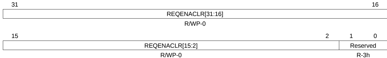
Figure 14-26. Interrupt Enable Clear Register 0 (REQENACLR0) [offset = FFFF FE40h]
