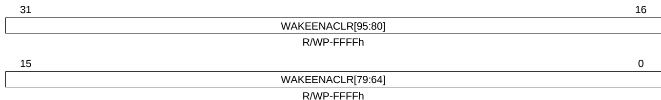
Figure 14-34. Wake-Up Enable Clear Register 2 (WAKEENACLR2) [offset = FFFF FE68h]
