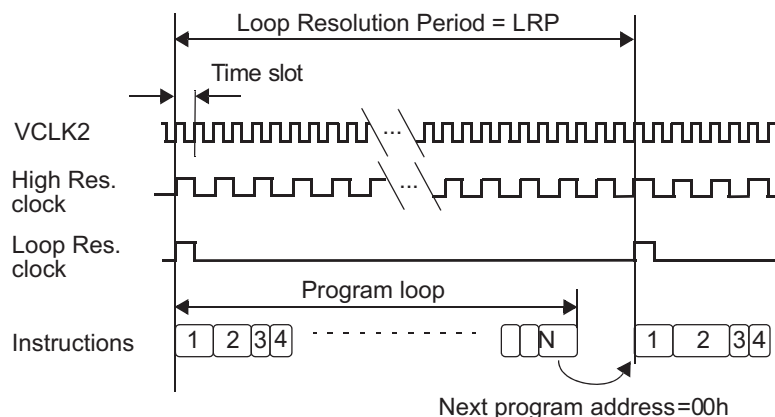
Figure 17-3. Program Flow Timings
