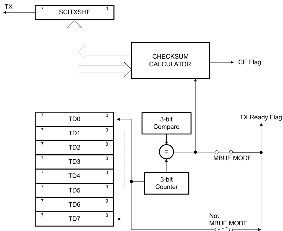
Figure 22-9. Transmit Buffers
