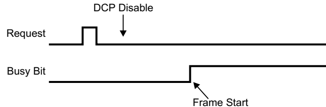
Figure 18-8. Timing for Disabling Control Packets
