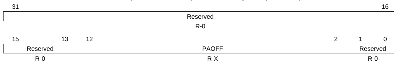
Figure 17-60. Parity Address Register (HETPAR)
