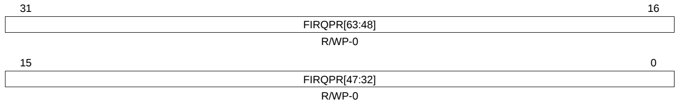
Figure 14-18. FIQ/IRQ Program Control Register 1 (FIRQPR1) [offset = FFFF FE14h]
