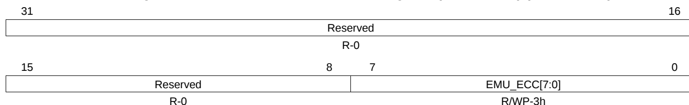
Figure 4-30. EEPROM Emulation ECC Register (FEMU_ECC) (offset = 60h)
