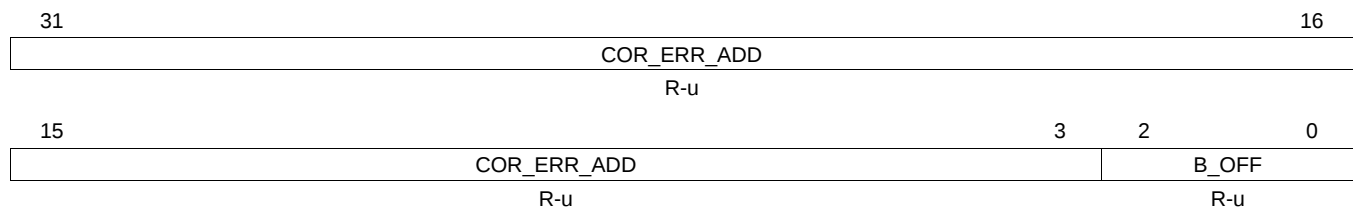
Figure 4-11. Flash Correctable Error Address Register (FCOR_ERR_ADD) (offset = 14h)
