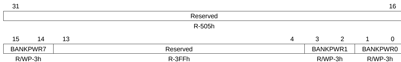
Figure 4-22. Flash Bank Fallback Power Register (FBFALLBACK) (offset = 40h)
