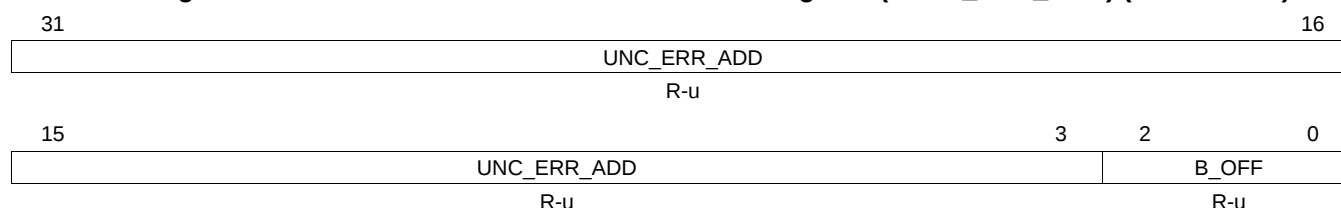
Figure 4-14. Flash Uncorrectable Error Address Register (FUNC_ERR_ADD) (offset = 20h)
