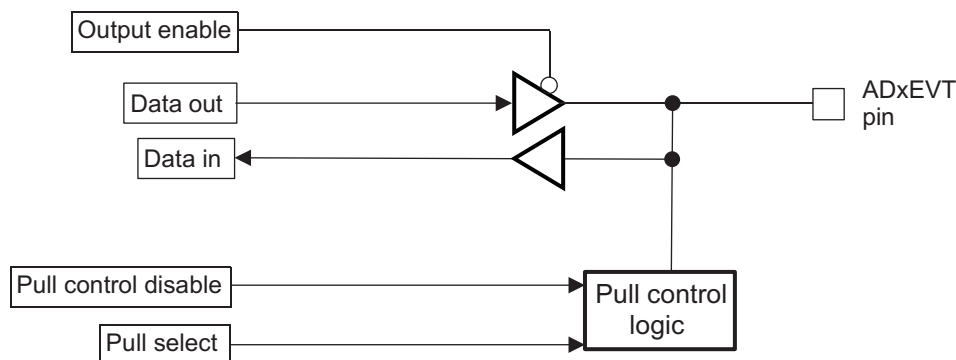
Figure 16-18. GPIO Functionality of ADxEVT
