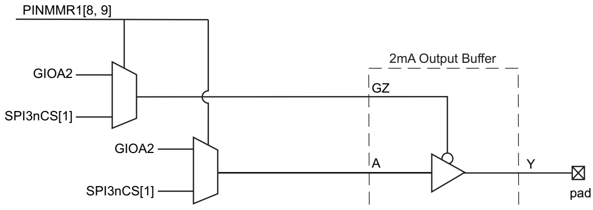
Figure 3-2. Output Multiplexing Example
