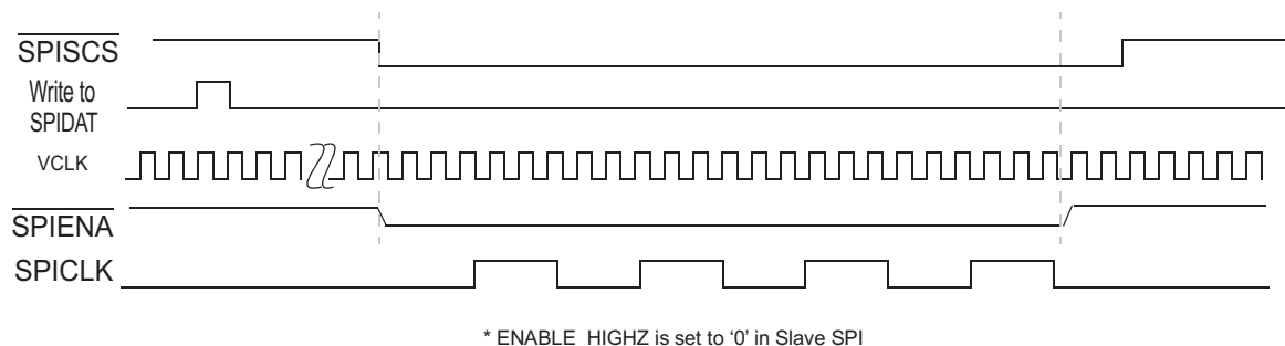
Figure 21-73. SPI/MibSPI pins during Slave mode in 5pin configuration - (Single Slave).
