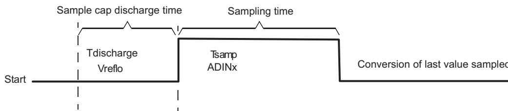
Figure 16-16. Timing for Sample Capacitor Discharge Mode
