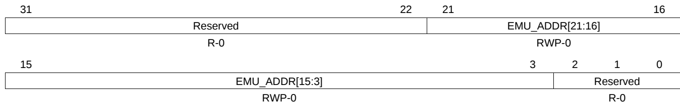
Figure 4-31. EEPROM Emulation Address Register (FEMU_ADDR) (offset = 68h)
