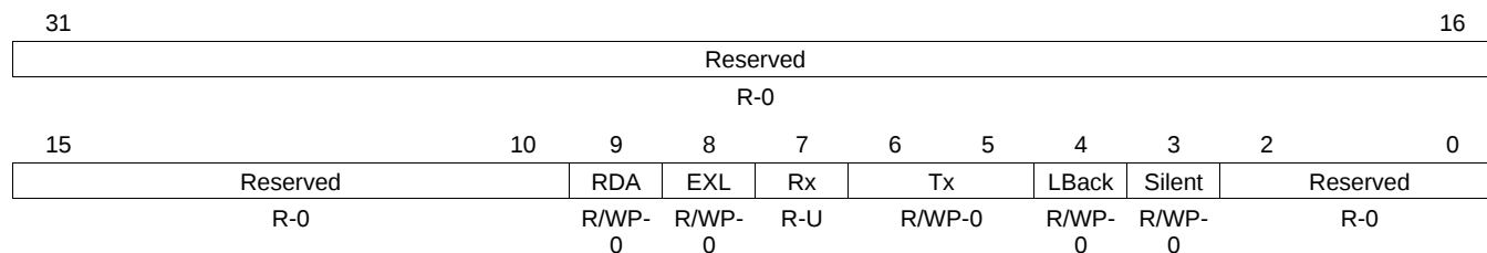
Figure 20-24. Test Register (DCAN TEST) [offset = 14h]
