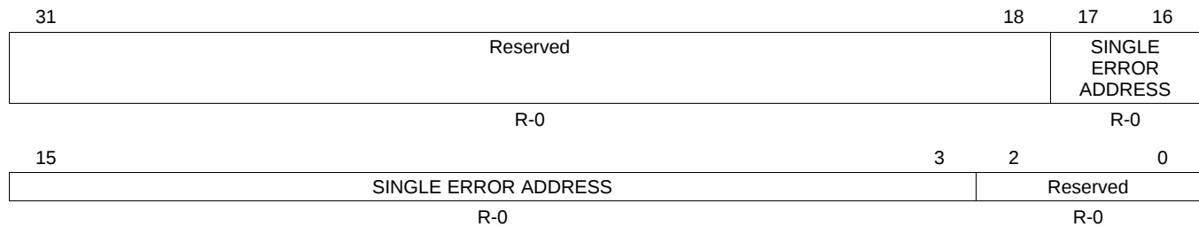
Figure 5-8. TCRAM Module Single-Bit Error Address Register (RAMSERRADDR) (offset = 14h)
