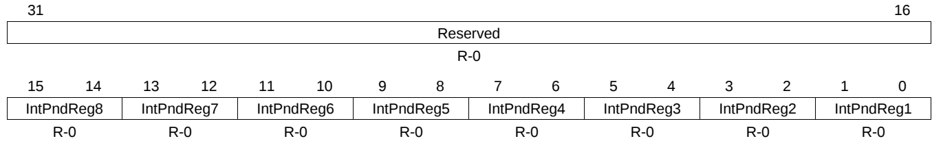
Figure 20-37. Interrupt Pending X Register (DCAN INTPND X) [offset = ACh]
