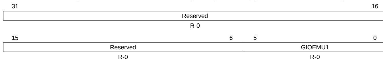
Figure 19-15. GIO Emulation 1 Register (GIOEMU1) [address = FFF7 BC2Ch]
