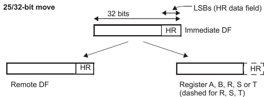
Figure 17-116. MOV32 Move Operation for REGTOREM (Case 10)
