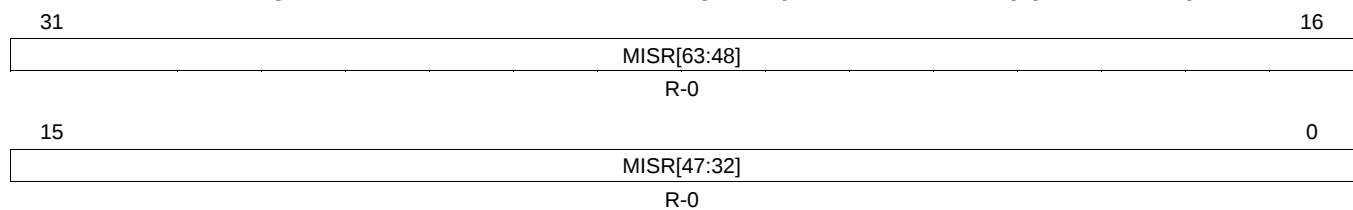
Figure 7-11. CPU1 Current MISR Register (CPU1_CURMISR2) (offset = 20h)
