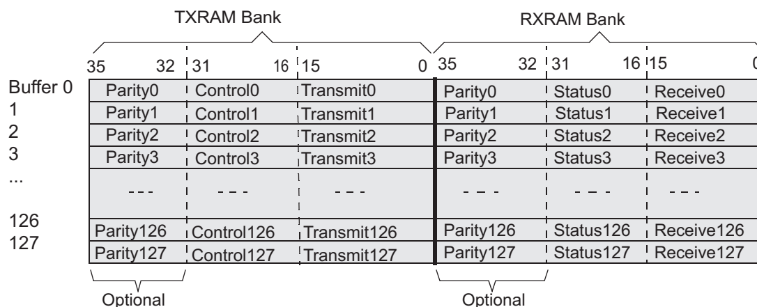
Figure 21-62. Multi-Buffer RAM Configuration
