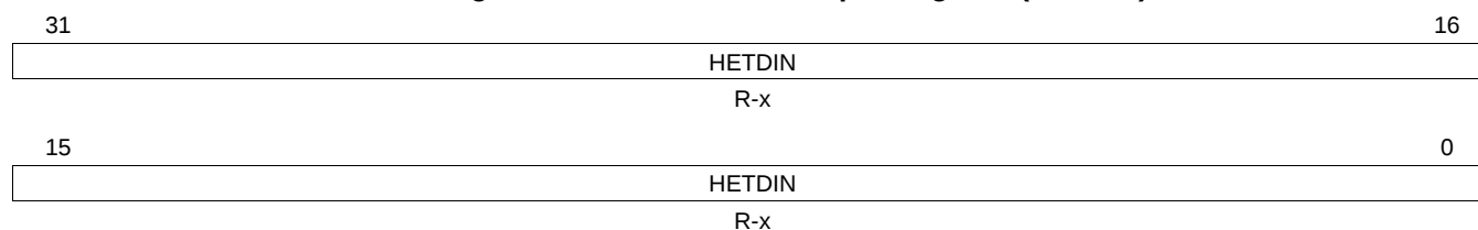
Figure 17-52. N2HET Data Input Register (HETDIN)
