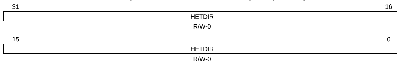
Figure 17-51. N2HET Direction Register (HETDIR)
