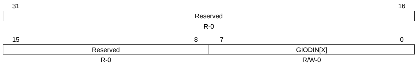
Figure 19-18. GIO Data Input Registers [A-H][7:0] (IODIN[A-H]) [address = FFF7BC38h, FFF7BC58h, FFF7BC78h, FFF7BC98h, FFF7BCB8h, FFF7BCD8h, FFF7BCF8h, FFF7BD18h]
