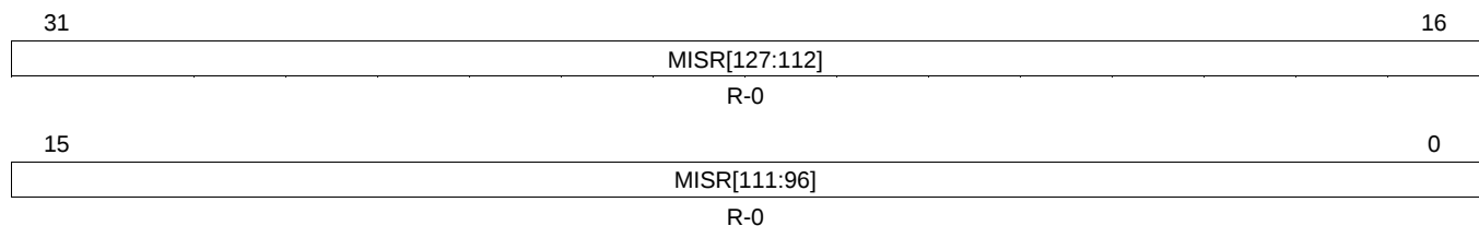
Figure 7-13. CPU1 Current MISR Register (CPU1_CURMISR0) (offset = 28h)
