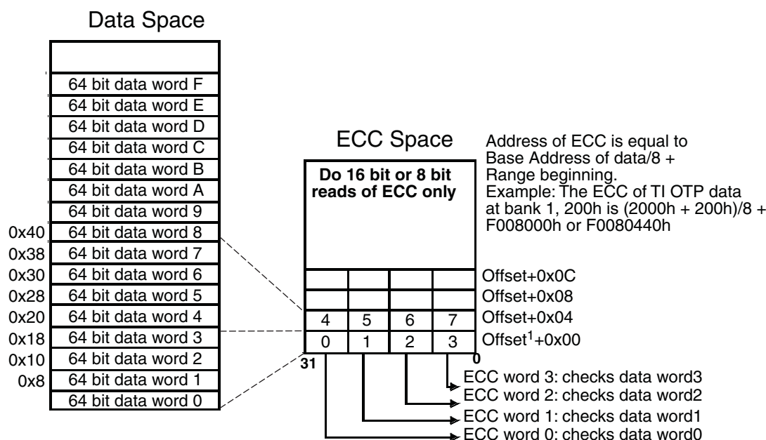
Figure 4-1. ECC Byte Mapping
