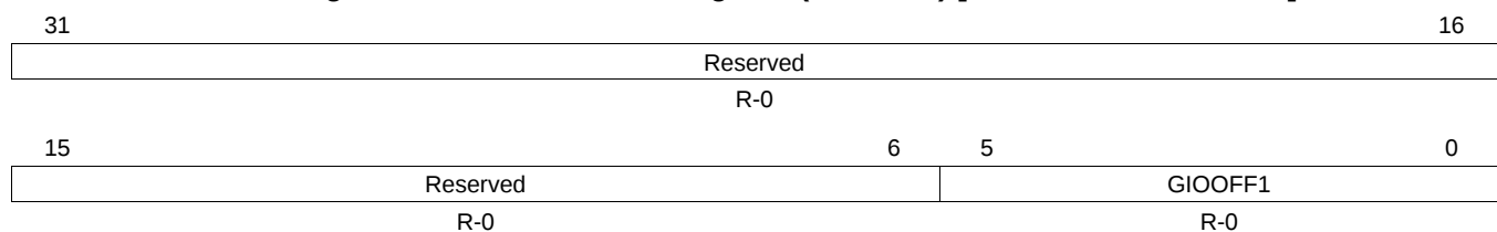
Figure 19-13. GIO Offset 1 Register (GIOOFF1) [address = FFF7 BC24h]
