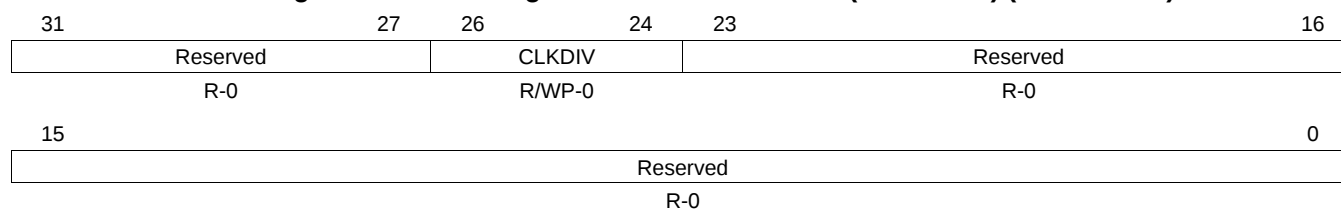
Figure 2-58. CPU Logic BIST Clock Prescaler (STCLKDIV) (offset = 08h)
