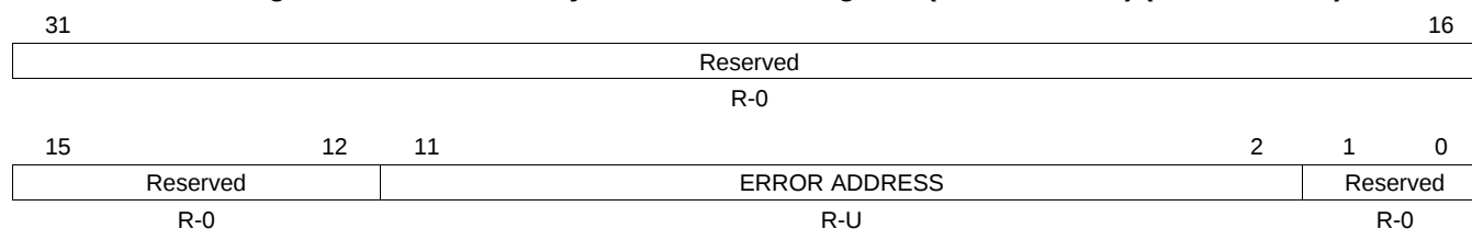
Figure 16-82. ADC Parity Error Address Register (ADPARADDR) (offset = 184h)
