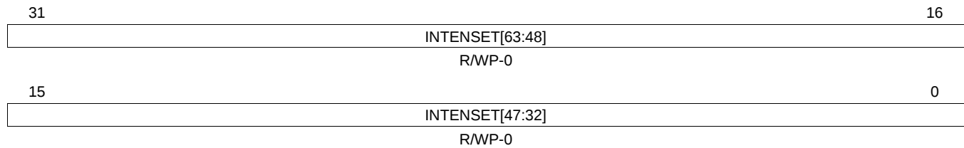
Figure 11-29. ESM Interrupt Enable Set/Status Register 4 (ESMIESR4) [offset = FFFF F548h]
