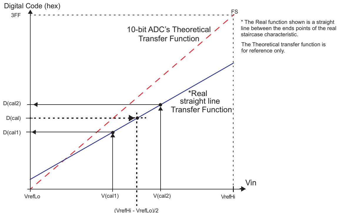
Figure 16-13. Mid-point Value Calculation
