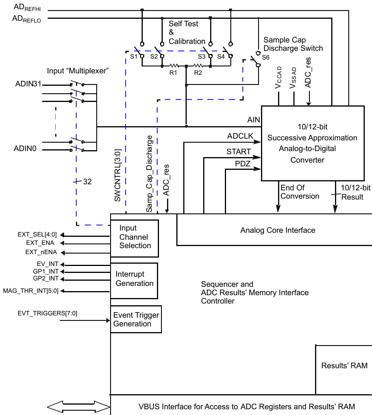
Figure 16-1. ADC Block Diagram
