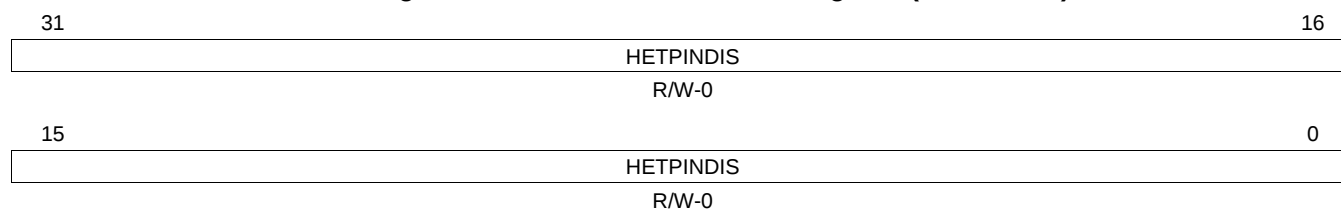
Figure 17-66. N2HET Pin Disable Register (HETPINDIS)
