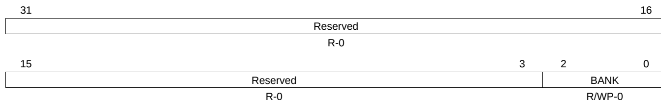
Figure 4-26. Flash Module Access Control Register (FMAC) (offset = 50h)
