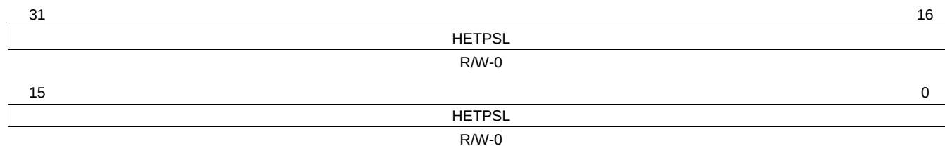
Figure 17-58. N2HET Pull Select Register (HETPSL)
