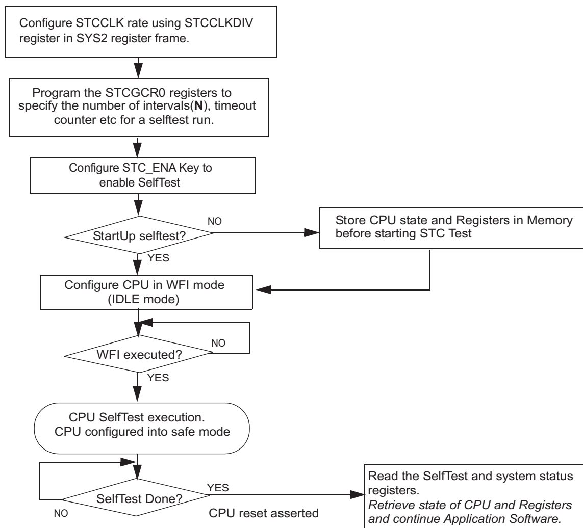
Figure 7-2. Application Self-Test Flow Chart
