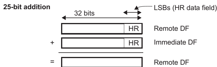
Figure 17-77. ADCNST Operation if Remote Data Field [31:7] Is Zero
