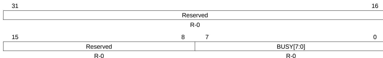
Figure 4-20. Flash Bank Busy Register (FBBUSY) (offset = 38h)
