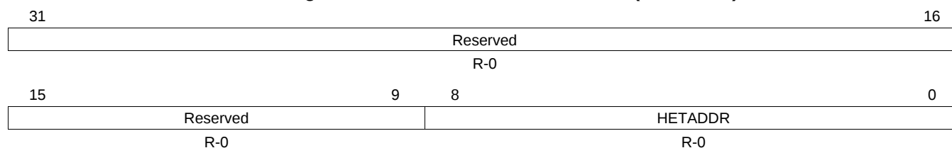
Figure 17-37. N2HET Current Address (HETADDR)
