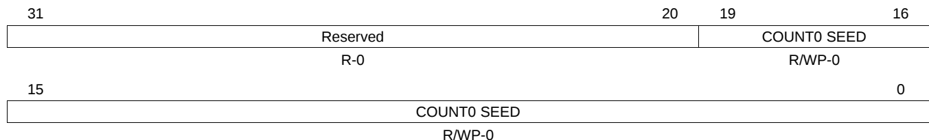
Figure 10-9. DCC Counter0 Seed Register (DCCNT0SEED) (offset = 08h)
