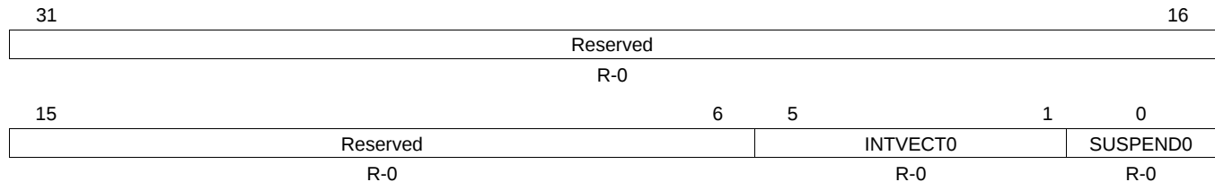
Figure 21-42. Interrupt Vector 0 (NTVECT0) [offset = 60h]
