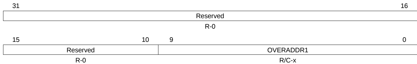
Figure 21-56. RXRAM Uncorrectable Parity Error Address Register (UERRADDR1) [offset = 128h]
