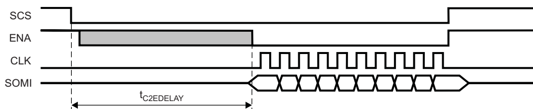
Figure 21-39. Chip-Select-Active-to-ENA-Signal-Active-Timeout
