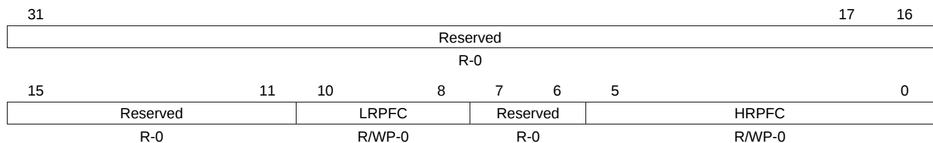
Figure 17-36. Prescale Factor Register (HETPFR)
