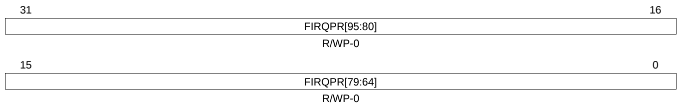
Figure 14-19. FIQ/IRQ Program Control Register 2 (FIRQPR2) [offset = FFFF FE18h]
