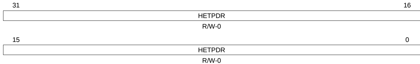
Figure 17-56. N2HET Open Drain Register (HETPDR)
