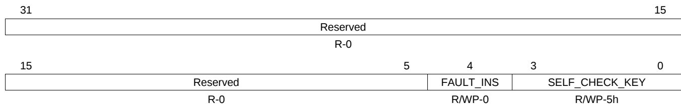
Figure 7-18. Signature Compare Self Check Register (STCSCSCR) (offset = 3Ch)
