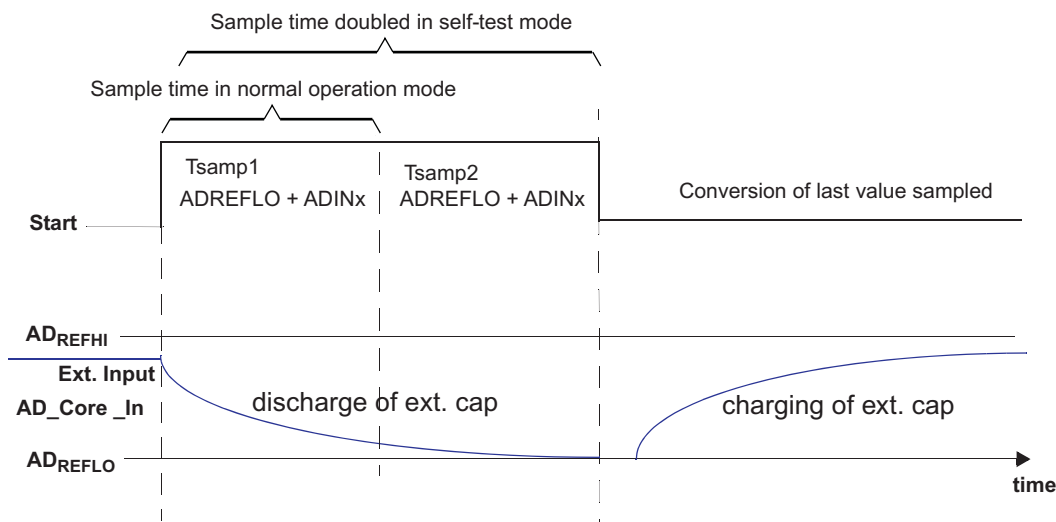
Figure 16-15. Timing for Self-Test Mode
