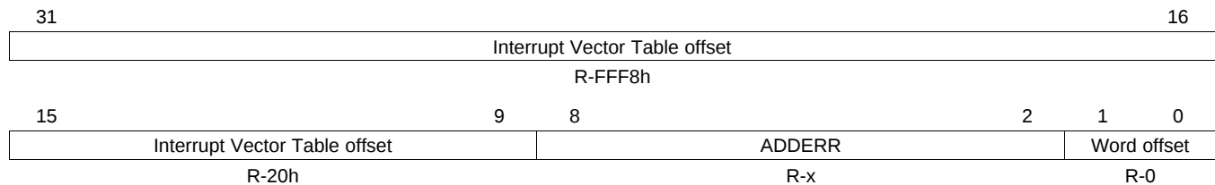
Figure 14-13. Address Parity Error Register (ADDERR) [Offset = FFFF FDF4h]
