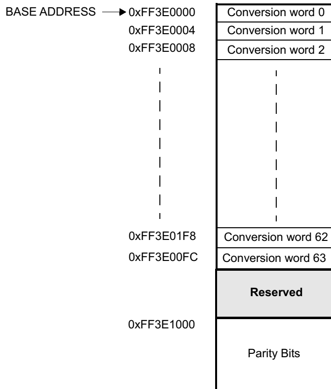
Figure 16-17. ADC Memory Map in Parity Test Mode
