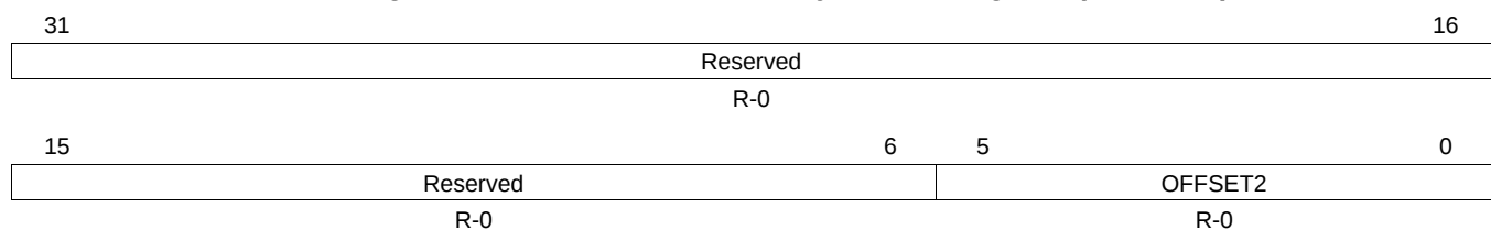
Figure 17-39. Offset Index Priority Level 2 Register (HETOFF2)
