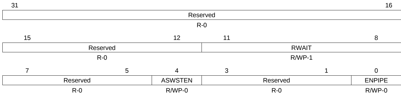
Figure 4-7. Flash Option Control Register (FRDCNTL) (offset = 00h)
