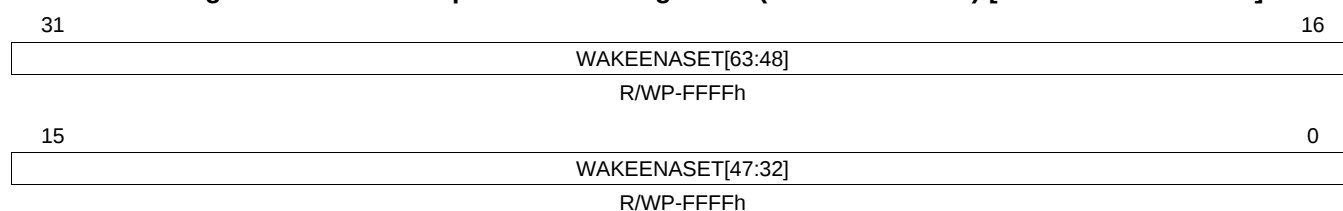
Figure 14-30. Wake-Up Enable Set Register 1 (WAKEENASET1) [offset = FFFF FE54h]
