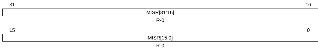
Figure 7-10. CPU1 Current MISR Register (CPU1_CURMISR3) (offset = 1Ch)
