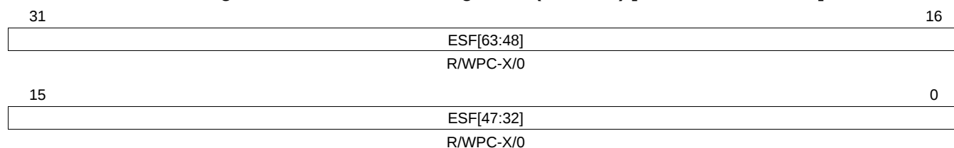
Figure 11-33. ESM Status Register 4 (ESMSR4) [offset = FFFF F558h]
