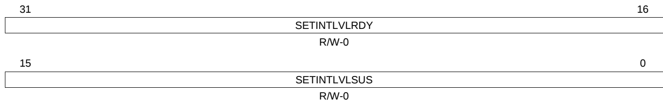
Figure 21-47. Transfer Group Interrupt Level Set Register (TGITLVST) [offset = 7Ch]
