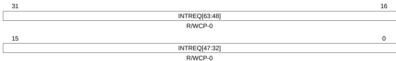
Figure 14-21. Pending Interrupt Read Location 1 (INTREQ1) Register [offset = FFFF FE24h]
