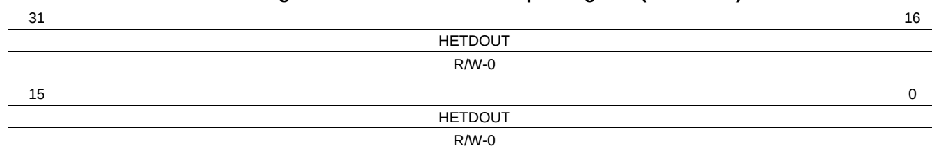
Figure 17-53. N2HET Data Output Register (HETDOUT)
