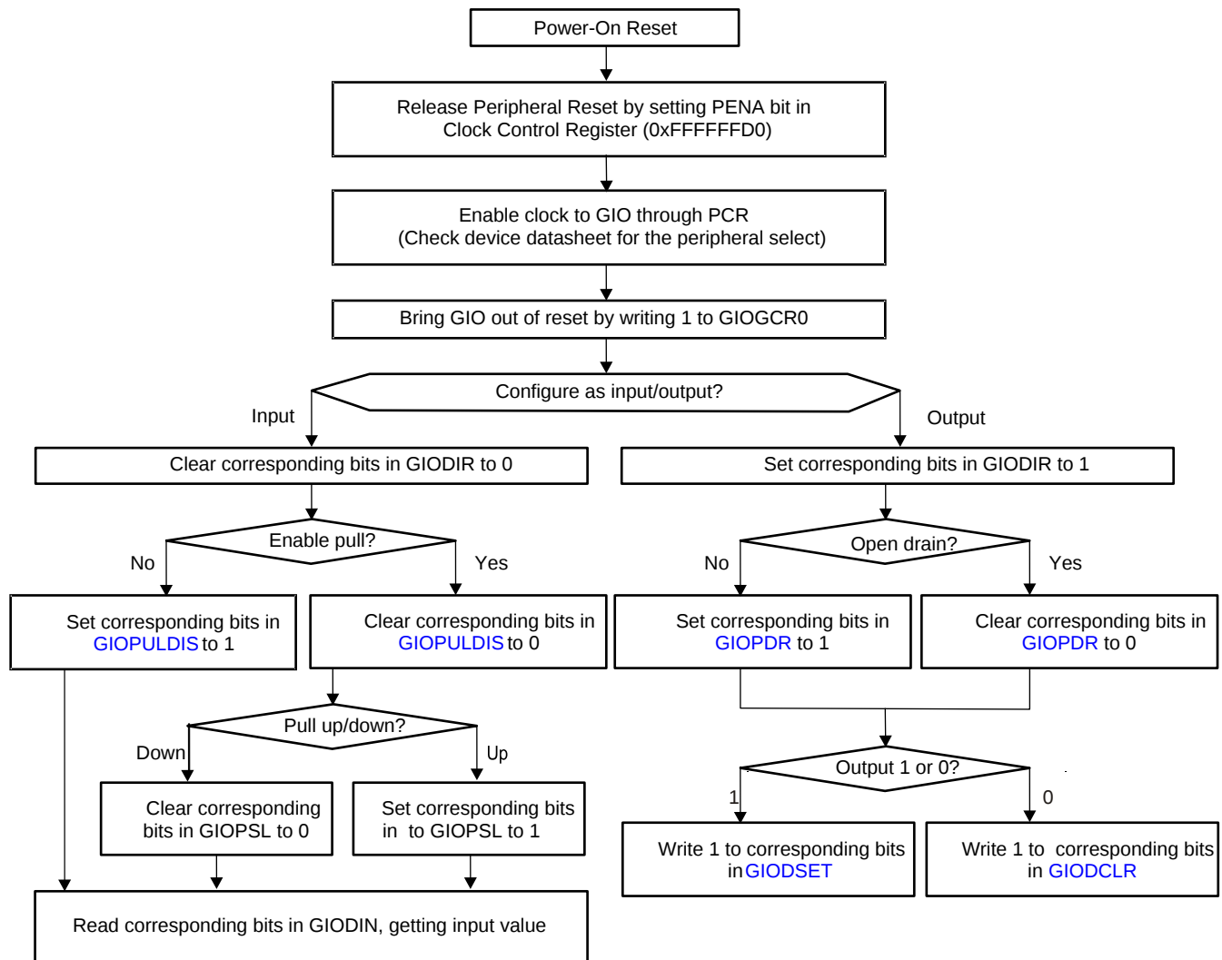
Figure 19-2. I/O Function Quick Start Flow Chart
