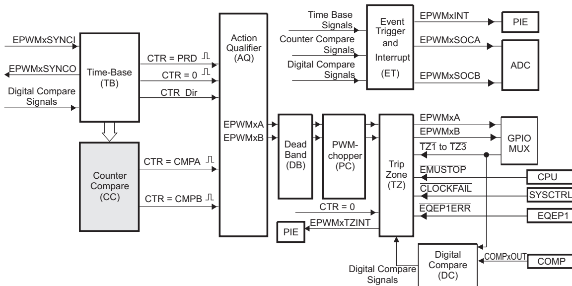
Figure 3-14. Counter-Compare Submodule
