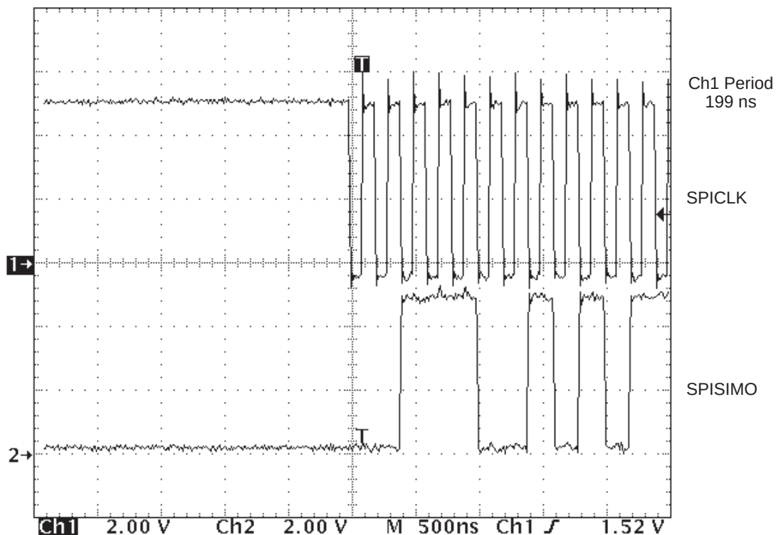
Figure 12-26. CLOCK POLARITY = 1, CLOCK PHASE = 0 (All data transitions are during the falling edge. Inactive level is high.)
