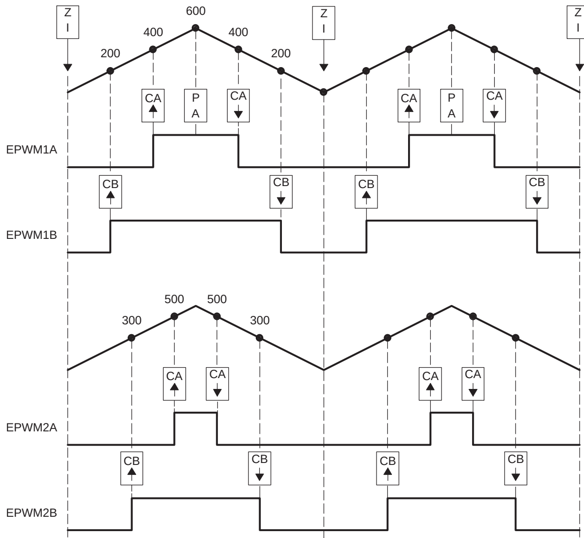
Figure 3-59. Buck Waveforms for Figure 3-58 (Note: F_{PWM2} = F_{PWM1} )
