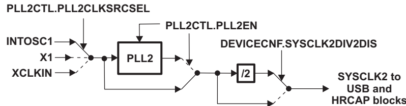
Figure 1-28. PLL2 Input and Output Configurations
