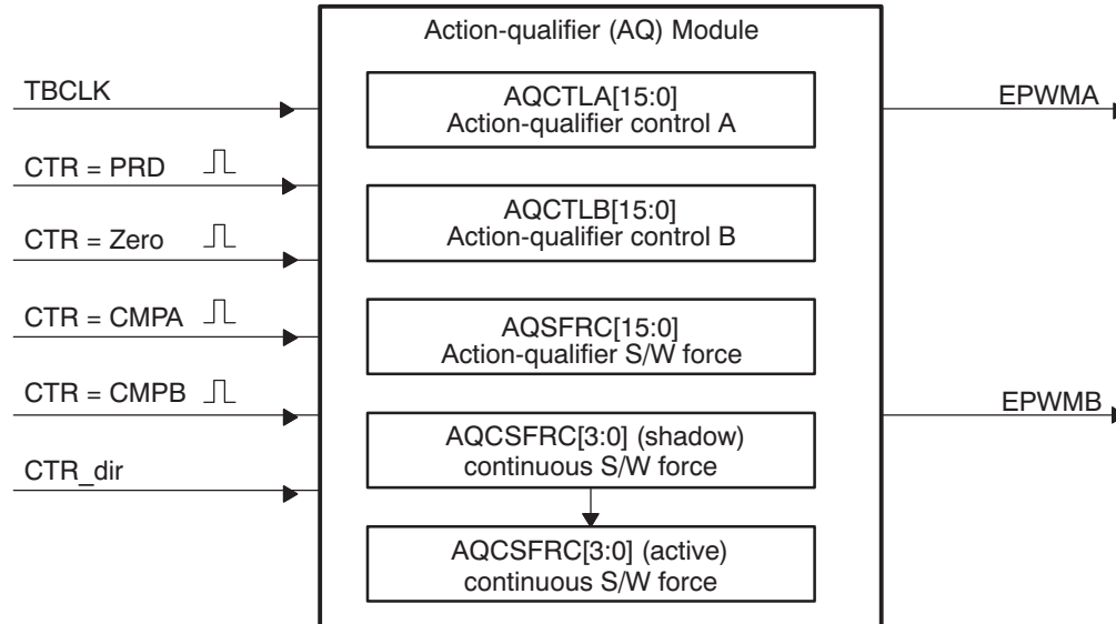
Figure 3-21. Action-Qualifier Submodule Inputs and Outputs
