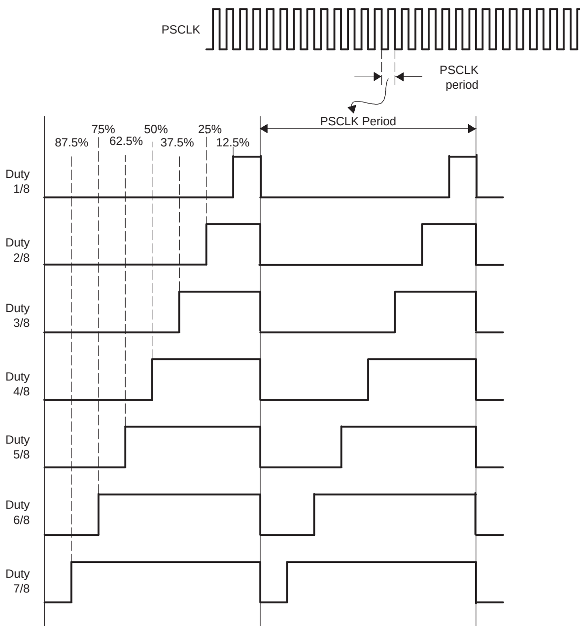
Figure 3-37. PWM-Chopper Submodule Waveforms Showing the Pulse Width (Duty Cycle) Control of Sustaining Pulses
