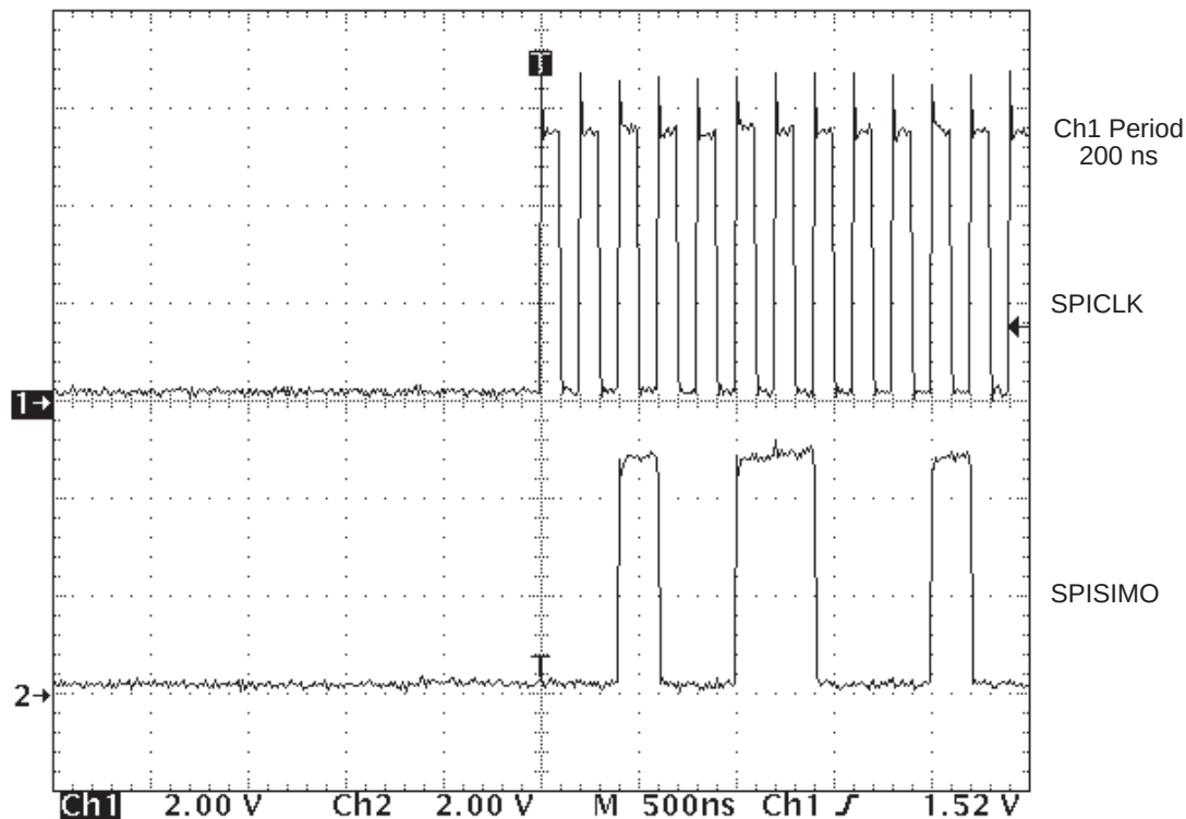
Figure 12-24. CLOCK POLARITY = 0, CLOCK PHASE = 0 (All data transitions are during the rising edge, non-delayed clock. Inactive level is low.)
