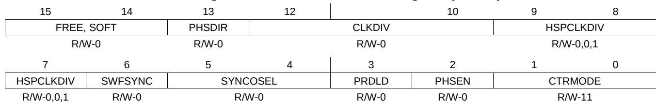
Figure 3-81. Time-Base Control Register (TBCTL)
