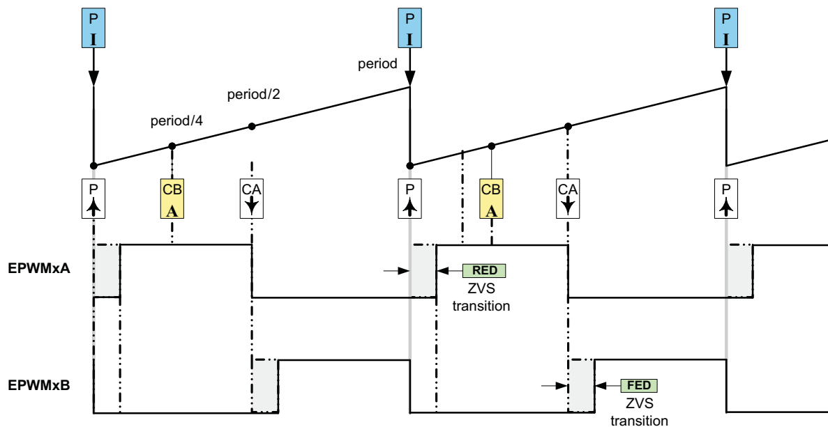
Figure 3-73. H-Bridge LLC Resonant Converter PWM Waveforms
