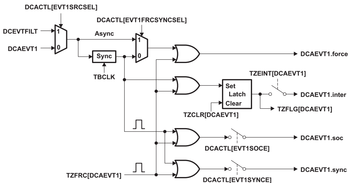
Figure 3-48. DCAEVT1 Event Triggering
