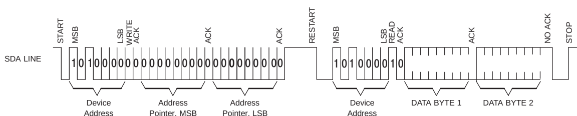
Figure 2-25. Sequential Read
