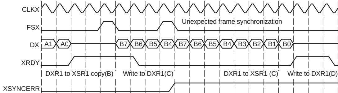
Figure 15-30. An Unexpected Frame-Synchronization Pulse During a McBSP Transmission
