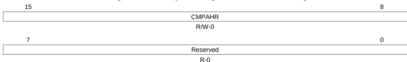
Figure 3-89. Compare A High Resolution Mirror Register
