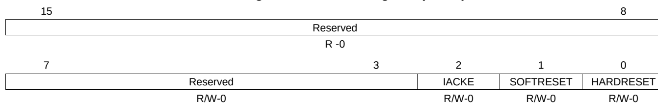
Figure 9-3. Control Register (MCTL)
