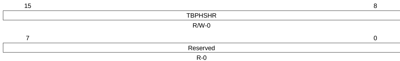
Figure 3-79. Time-Base Phase High Resolution Register (TBPHSHR)
