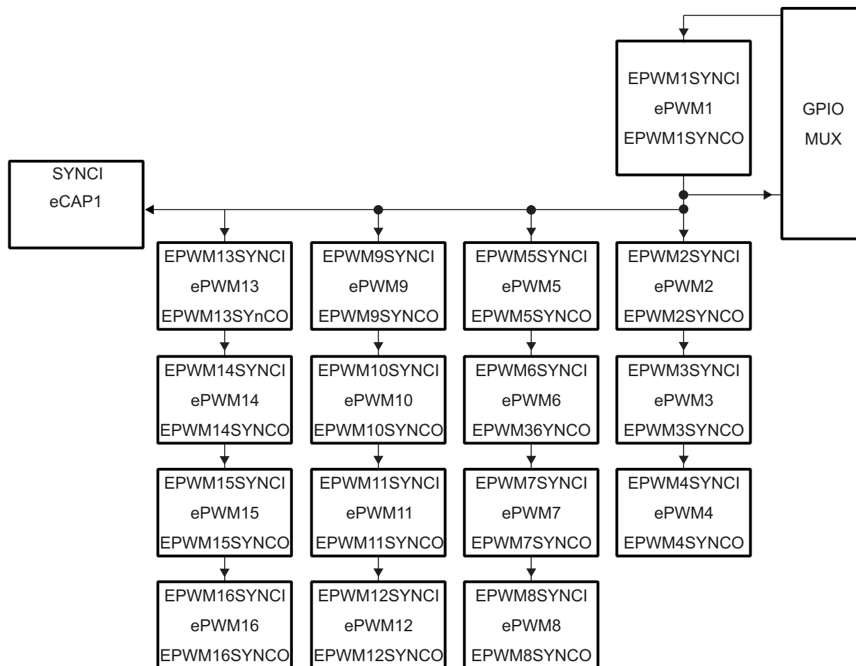
Figure 3-8. Time-Base Counter Synchronization Scheme 2
