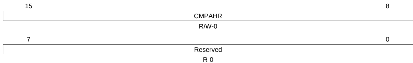
Figure 3-87. Compare A High Resolution Register (CMPAHR)
