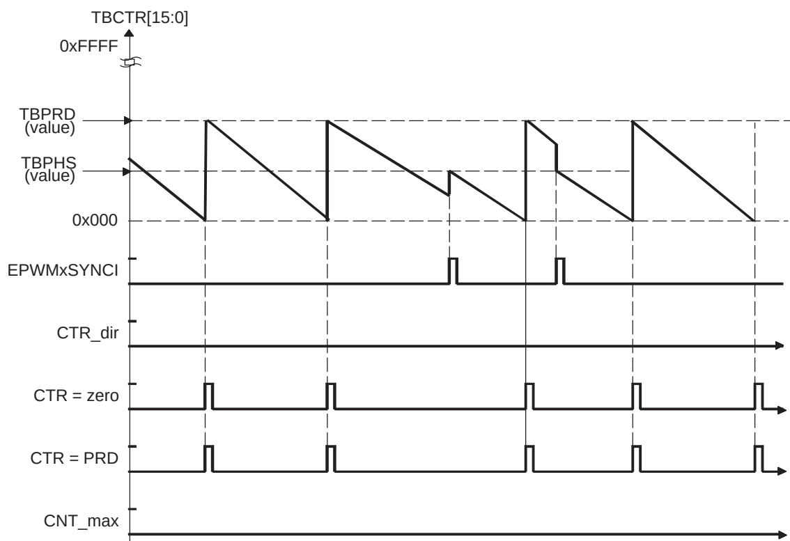
Figure 3-11. Time-Base Down-Count Mode Waveforms
