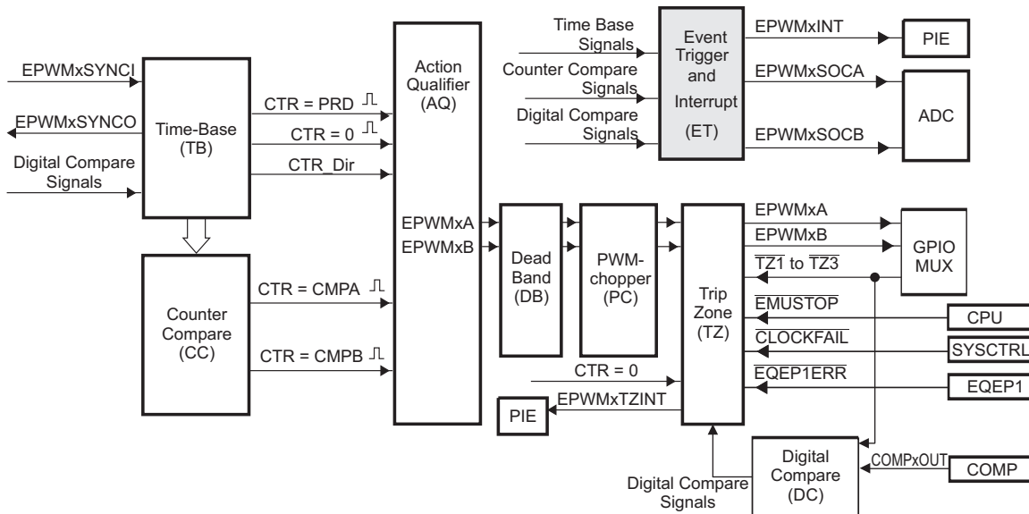
Figure 3-41. Event-Trigger Submodule
