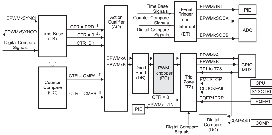
Figure 3-33. PWM-Chopper Submodule
