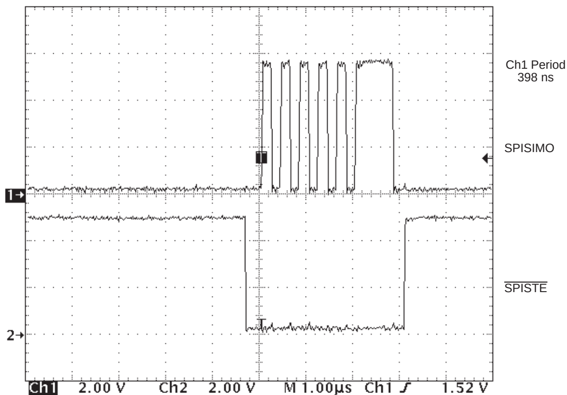
Figure 12-29. \overline{\text{SPISTE}} Behavior in Slave Mode (Slave's \overline{\text{SPISTE}} is lowered during the entire 16 bits of transmission.)
