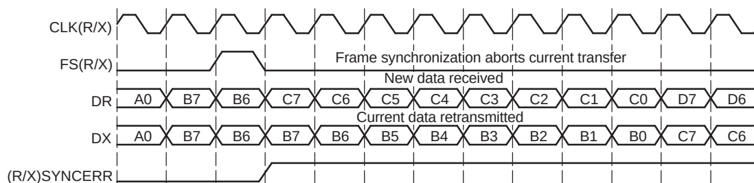
Figure 15-51. Unexpected Frame-Synchronization Pulse With (R/X) FIG = 0
