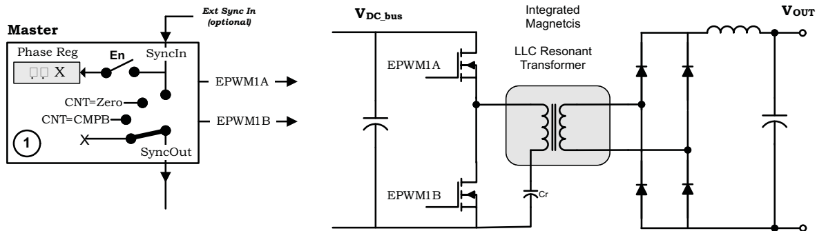
Figure 3-72. Control of Two Resonant Converter Stages
