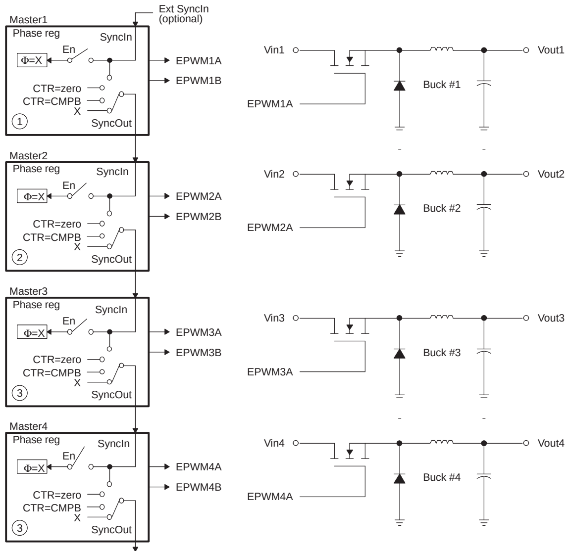
Figure 3-56. Control of Four Buck Stages. Here F_{PWM1} \neq F_{PWM2} \neq F_{PWM3} \neq F_{PWM4}
