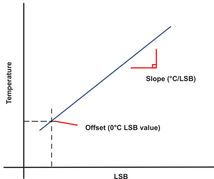
Figure 8-38. Temperature Sensor Transfer Function
