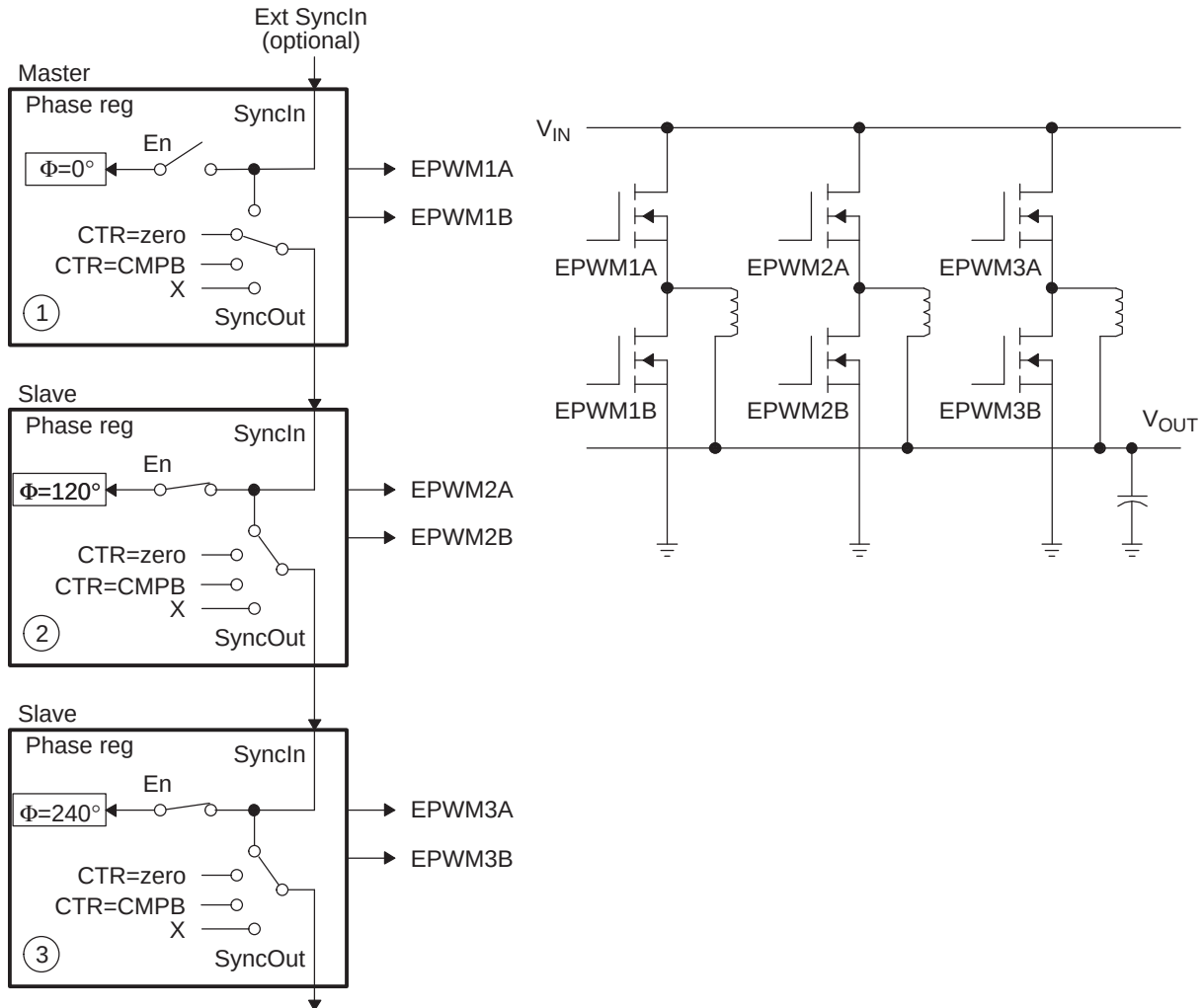
Figure 3-66. Control of a 3-Phase Interleaved DC/DC Converter
