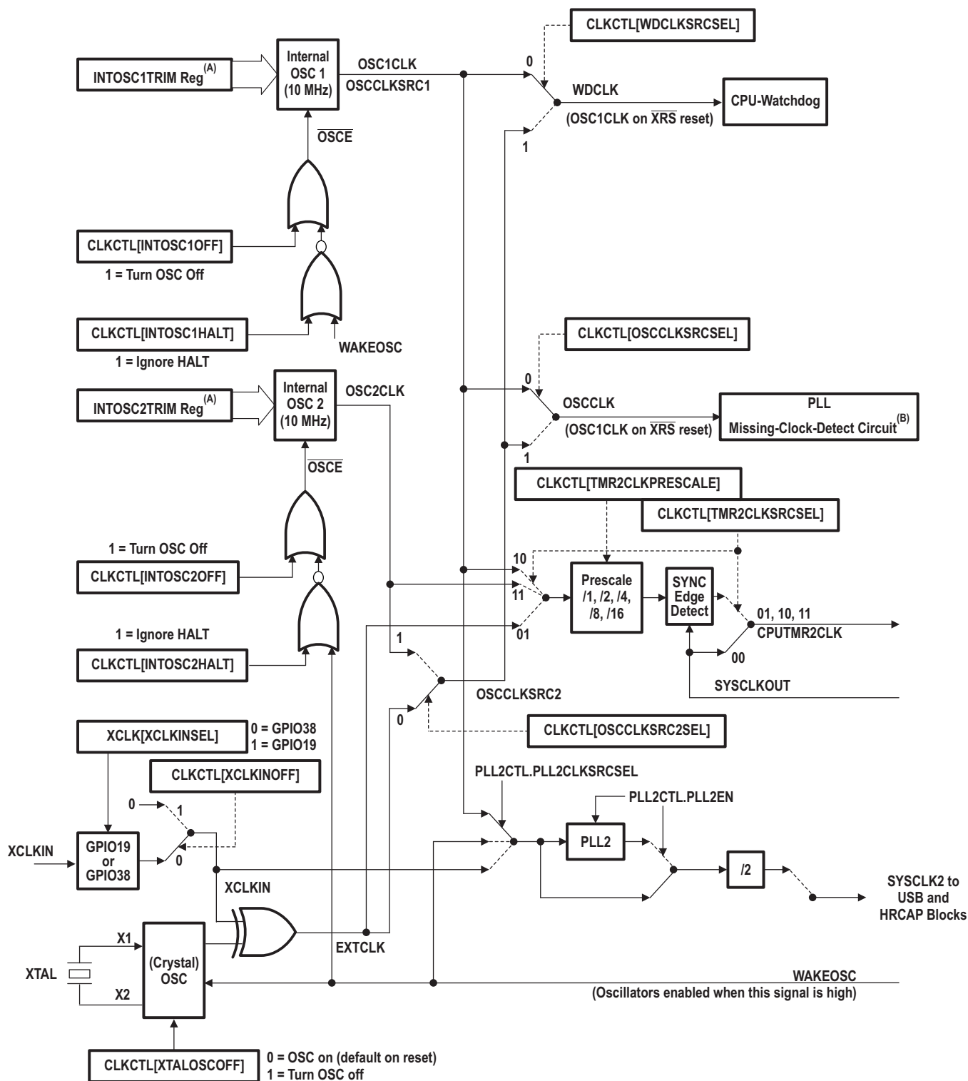
Figure 1-19. Clocking Options
