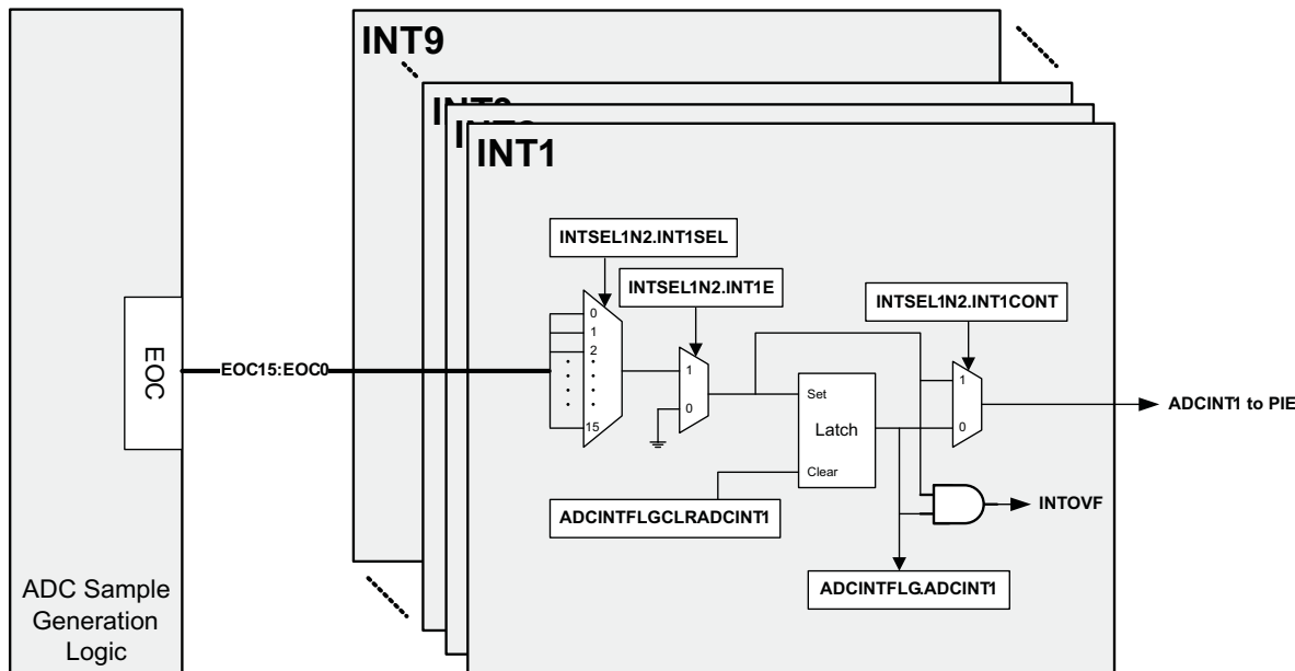
Figure 8-7. Interrupt Structure
