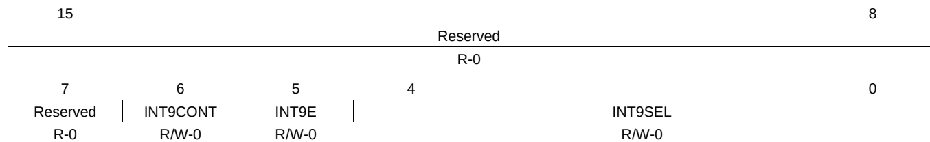
Figure 8-18. Interrupt Select 9 And 10 Register (INTSEL9N10) (Address Offset 0Ch)
