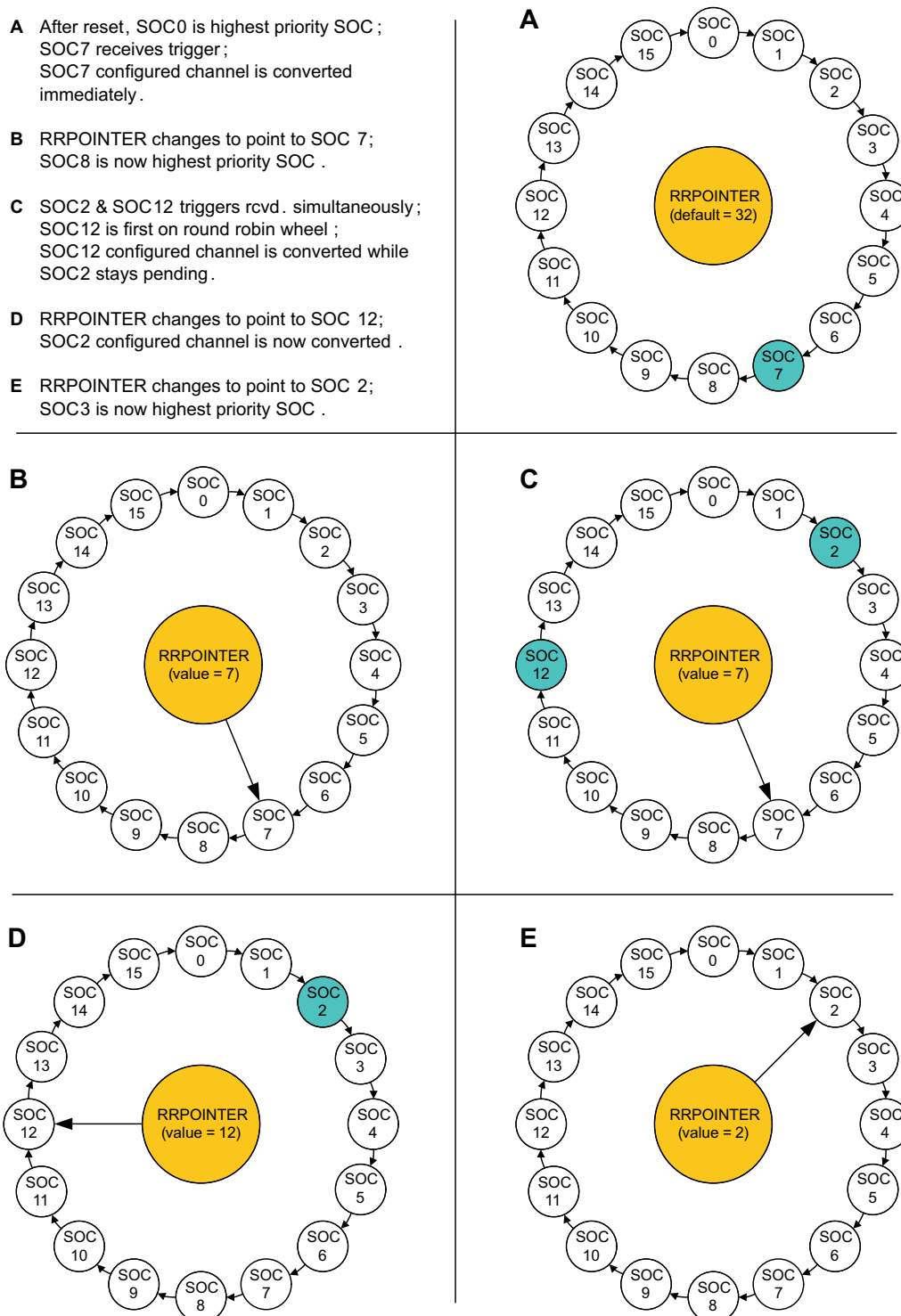
Figure 8-5. Round Robin Priority Example
