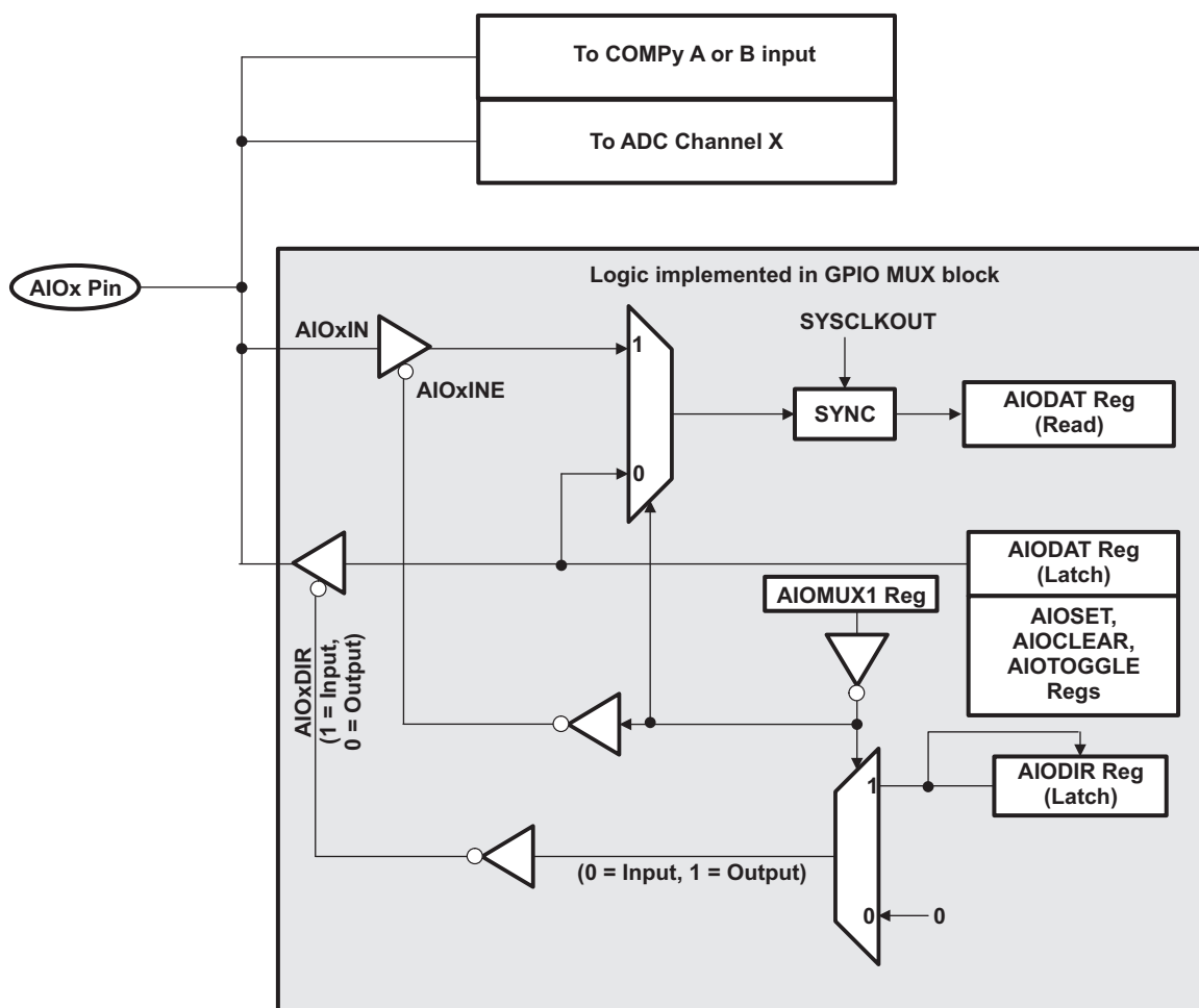
Figure 1-55. Analog/GPIO Multiplexing
