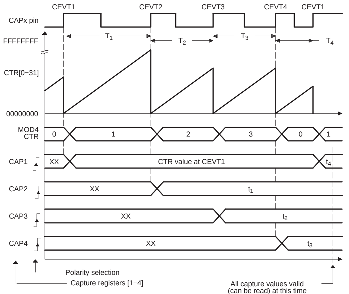
Figure 6-23. Capture Sequence for Delta Mode Time-stamp and Rising Edge Detect
