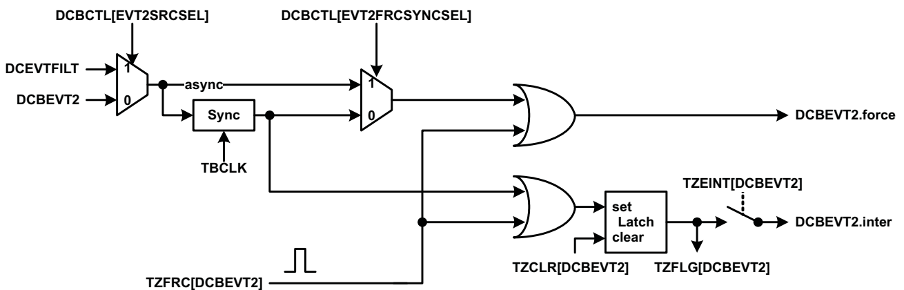
Figure 3-51. DCBEVT2 Event Triggering
