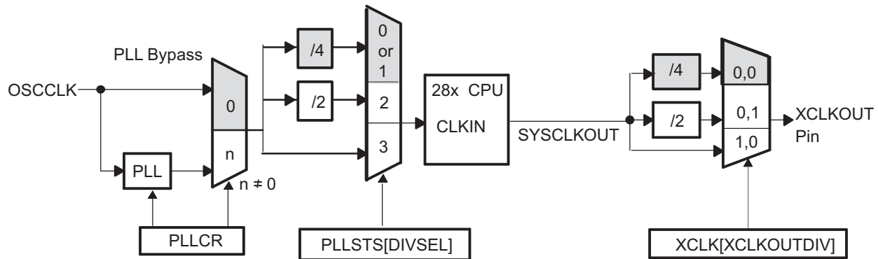
Figure 1-35. XCLKOUT Generation
