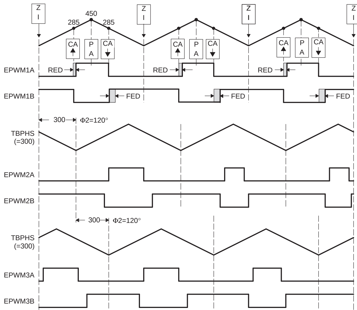
Figure 3-67. 3-Phase Interleaved DC/DC Converter Waveforms for Figure 3-66
