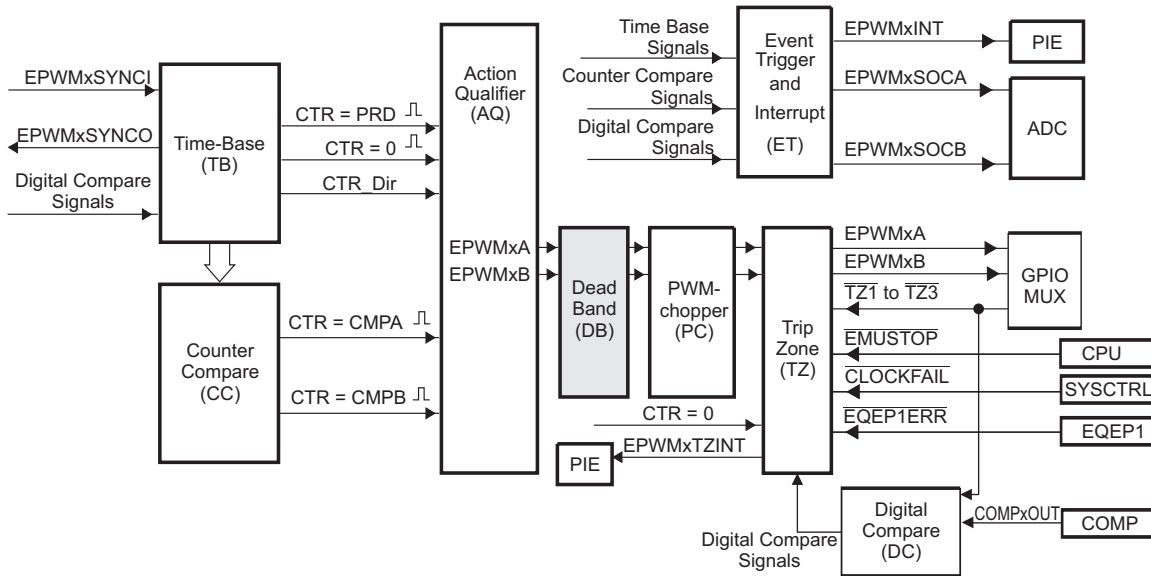
Figure 3-30. Dead_Band Submodule
