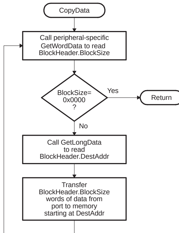
Figure 2-10. Overview of CopyData Function
