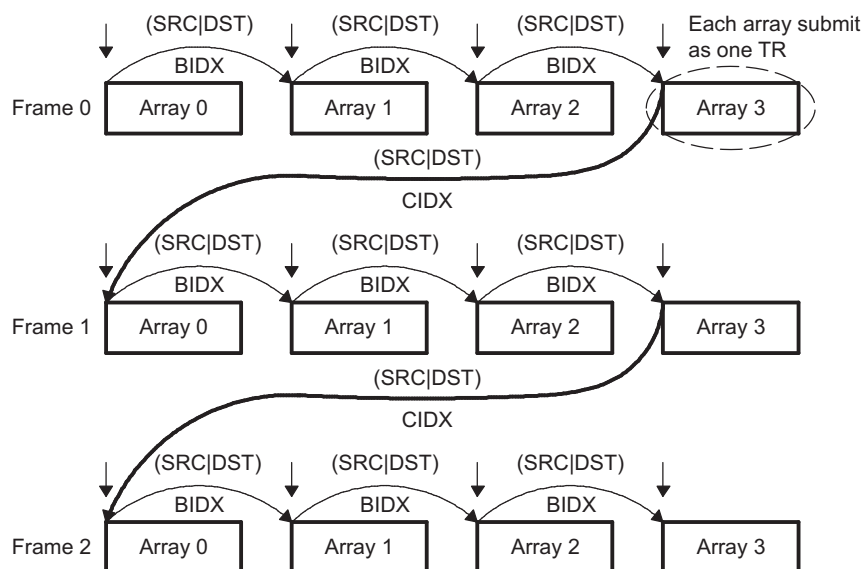
Figure 18-5. A-Synchronized Transfers (ACNT = n, BCNT = 4, CCNT = 3)
