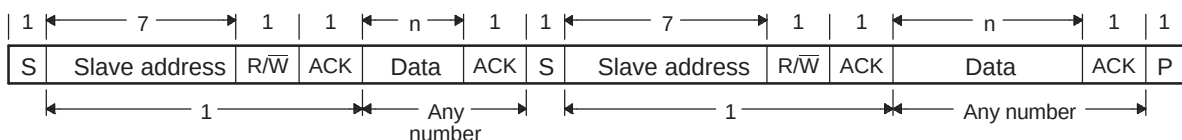
Figure 22-11. I2C Peripheral 7-Bit Addressing Format With Repeated START Condition (FDF = 0, XA = 0 in ICMR)
