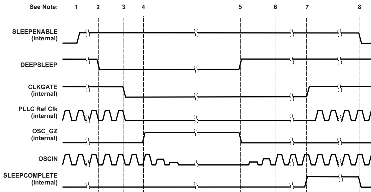
Figure 10-1. Deep Sleep Mode Sequence
