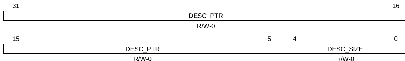
Figure 30-114. Queue Manager Queue N Control Register D (CTRLD[ N ])
