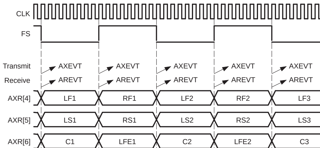
Figure 23-27. DMA Events in an Audio Example—Two Events
