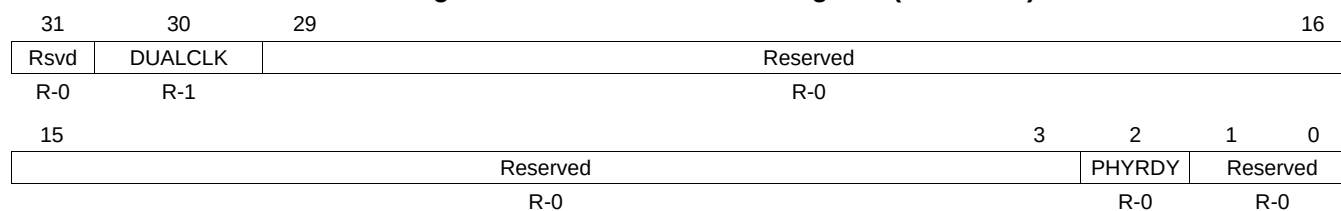
Figure 15-21. SDRAM Status Register (SDRSTAT)
