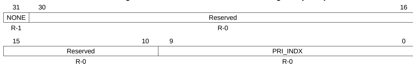
Figure 12-16. Global Prioritized Index Register (GPIR)
