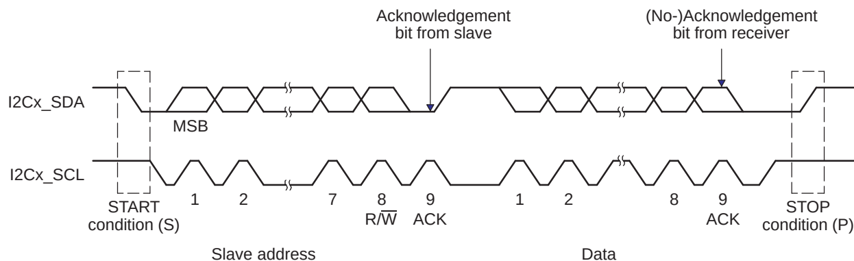
Figure 22-7. I2C Peripheral Data Transfer
