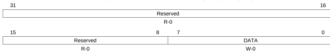
Figure 29-10. Transmitter Holding Register (THR)
