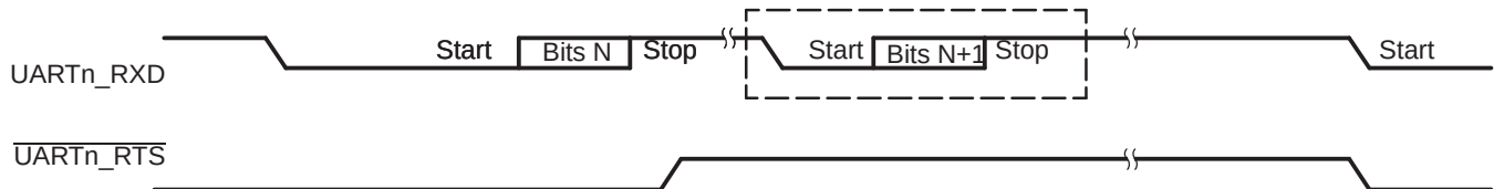
Figure 29-6. Autoflow Functional Timing Waveforms for UARTn_RTS
