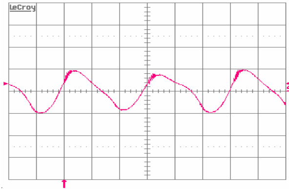
Figure 10. Output voltage ripple (20 mV/div.) at full rated load current into a resistive load with C_o = 10\ \mu\text{F} tantalum + 1\ \mu\text{F} ceramic and V_{in} = 48\ \text{V} . Time scale: 1\ \mu\text{s}/\text{div.}
