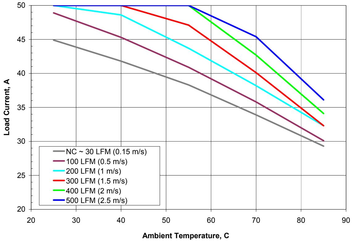
Figure 1. Available load current vs. ambient air temperature and airflow rates for SQE48T50012 converter mounted vertically with air flowing from pin 3 to pin 1, MOSFET temperature \leq 120\text{ }^{\circ}\text{C} , V_{in} = 48\text{ V} .
