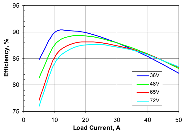
Figure 2. Efficiency vs. load current and input voltage for SQE48T50012 converter mounted vertically with air flowing from pin 3 to pin 1 at 300 LFM (1.5 m/s) and T_a = 25^{\circ}\text{C} .
