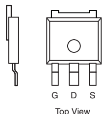
TO-252 Reverse Lead DPAK
